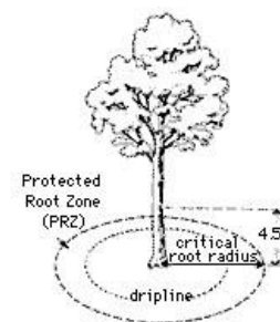
Figure 2. Approximate a tree's PRZ by calculating the critical root radius (CRR). First, measure the tree diameter in inches at breast height (DBH). Then multiply that number by 1.5 or 1.0. Express the result in feet.
