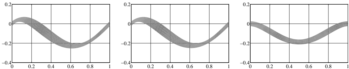
FIGURE 1. Deformation of the cross-section of a plate in plane strain as determined by the Reissner–Mindlin, elastic, and Kirchhoff–Love models, respectively
