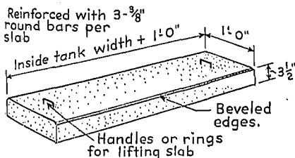
Fig. 5. Concrete cover slab.
