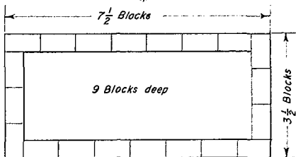
Fig. 6. Layout of concrete block septic tank.
