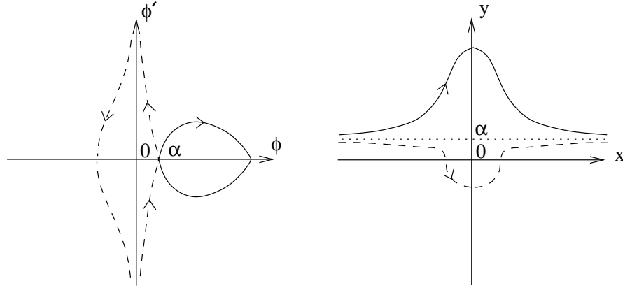
Fig. 2. Trajectories and graphs of the analytic and tipon solitary wave solutions of the K(3,3) equation.
