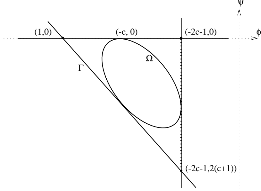
Fig. 3. The phase plane for the Boussinesq system.
