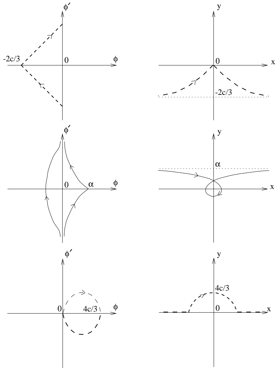
Fig. 1. Trajectories and graphs of the peakon, loopon and compacton solutions of the K(2,2) equation.
