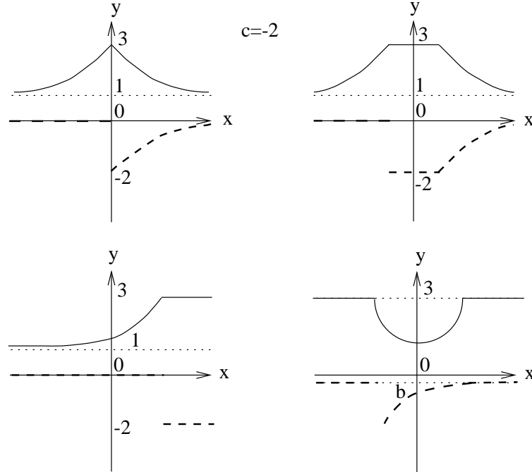
Fig. 4. Graphs of the peakon, mesaon, rampon and compacton solutions of the dual Boussinesq system.
