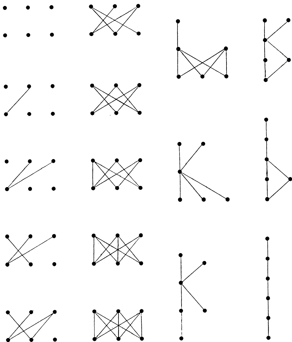
Figure 3: Maximal chain \mathcal{H}_6^l listed from top to bottom and left to right.
