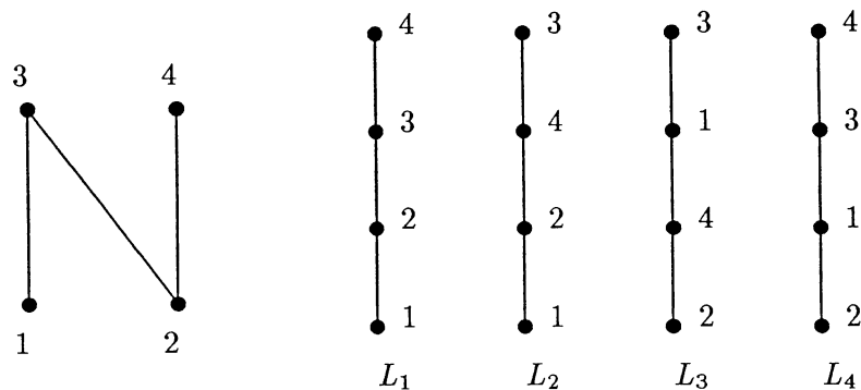
Figure 2: The poset N and its linear extensions.
