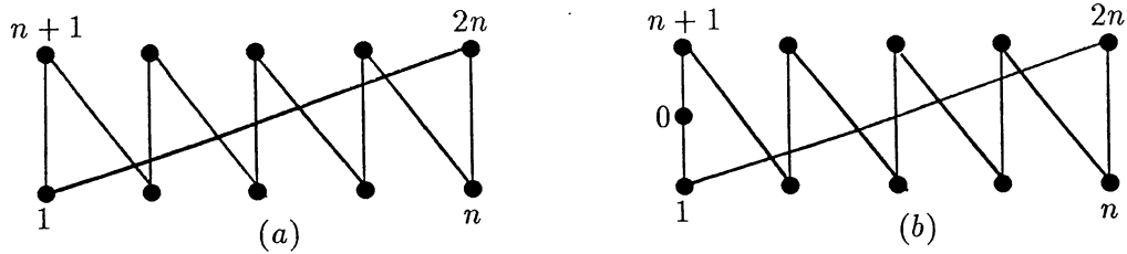
Figure 1: [n \geq 2] (a) Crown (b) C
