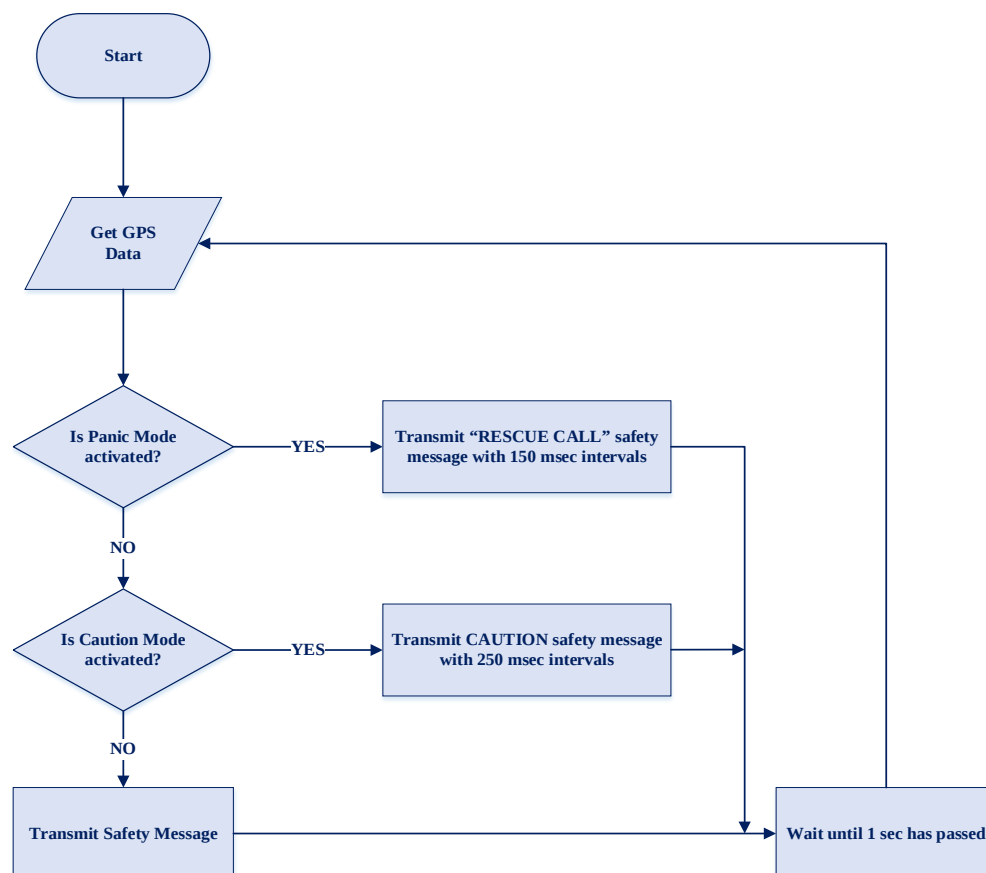
Figure 3.2 WSD software flowchart
