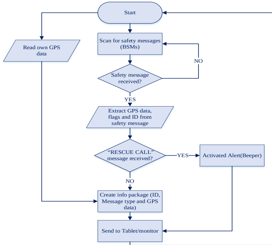
Figure 3.7 Construction Vehicle onboard DSRC device software flowchart
