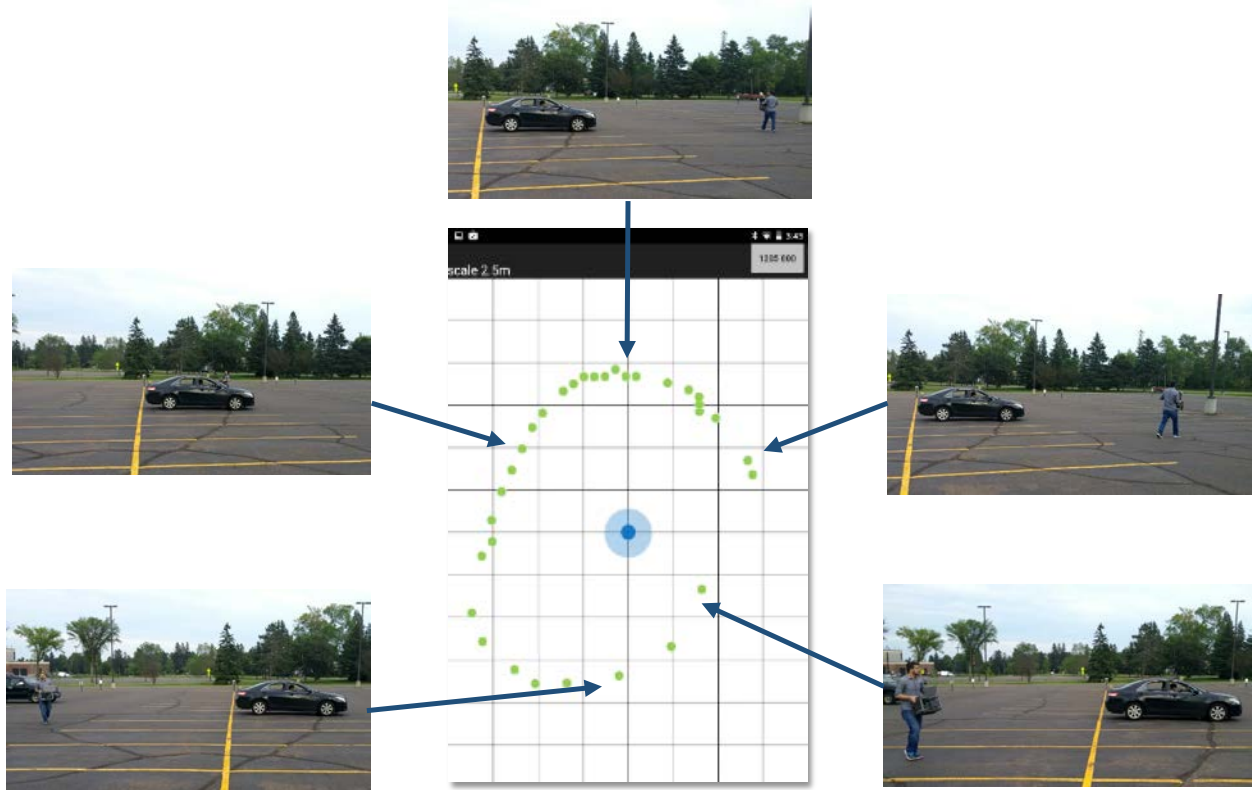
Figure 4.5 Tablet screen snapshot showing the trajectory of a worker walking around the construction vehicle in a circle.
