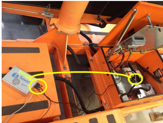
Figure 3.14 Serial connection between VMS and DSRC device.
