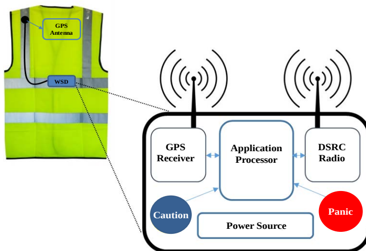
Figure 3.1 High level architectural design of the proposed WSD for worker. The inset shows the worker's vest with embedding locations of WSD and GPS antenna.
