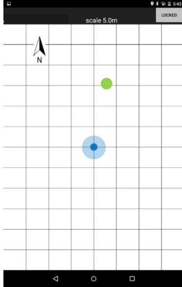
(a) Construction vehicle facing North without orientation correction (Correct position)
