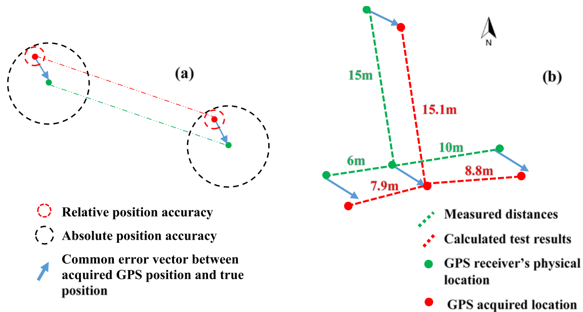
Figure 2.2 Conceptual diagram to show (a) absolute and relative position errors, and (b) measured test results.
