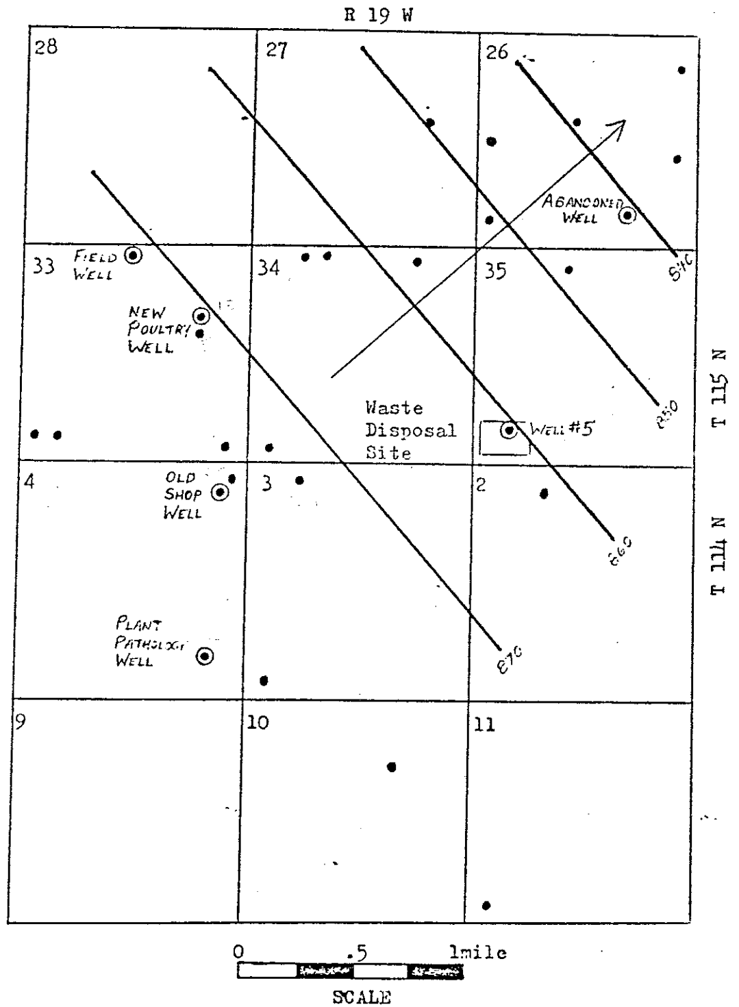
FIG. IV-6 PIEZOMETRIC HEAD AND FLOW DIRECTION IN THE PRAIRIE DU CHIEN-JORDAN AQUIFER
