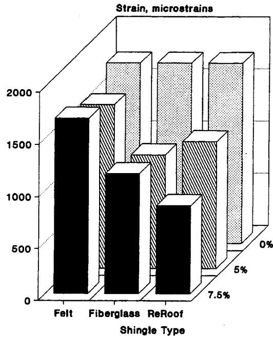
Figure 22. Low Temperature Properties (Strain at Peak Stress) for Dense Graded Mixtures, 120/150 AC.
