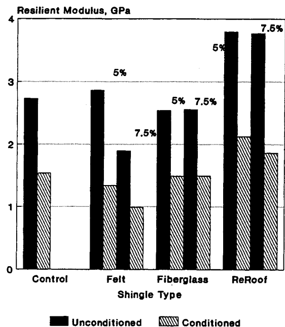
Figure 11. Moisture Sensitivity (Resilient Modulus) of Dense Graded Mixtures, 120/150 AC.
