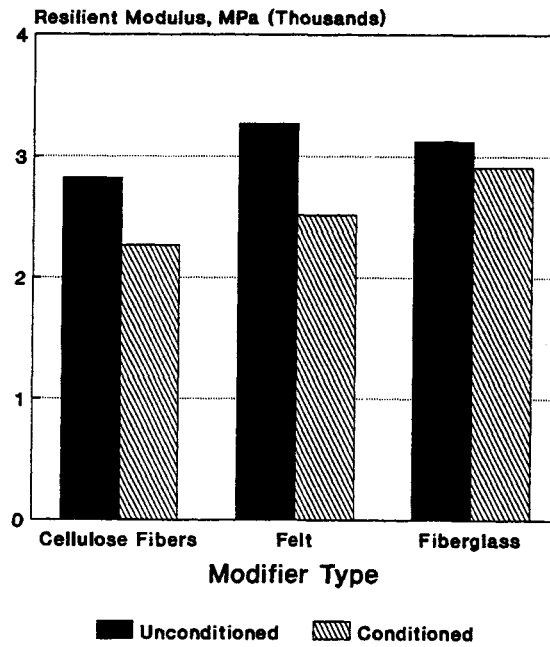
Figure 17. Moisture Sensitivity (Resilient Modulus) for SMA Mixtures.
