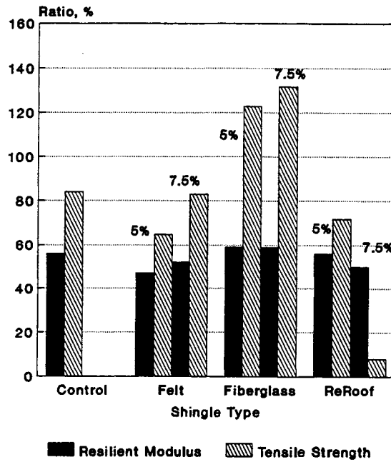
Figure 15. Moisture Sensitivity (Retained Parameter Ratios) for Dense Graded Mixtures, 120/150 AC.
