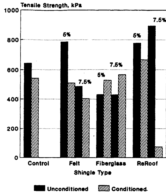
Figure 13. Moisture Sensitivity (Indirect Tensile Strength) of Dense Graded Mixtures, 120/150 AC.
