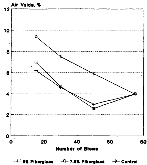
Figure 3. Influence of Compactive Effort on Air Voids for Mixtures Containing Fiberglass Shingles and 85/100 AC.
