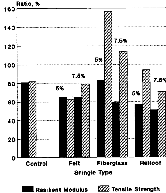
Figure 16. Moisture Sensitivity (Retained Parameter Ratios) for Dense Graded Mixtures, 85/100 AC.
