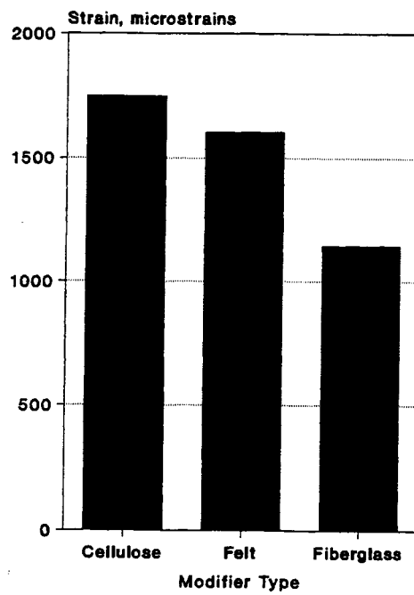
Figure 25. Low Temperature Properties (Strain at Peak Stress) for SMA Mixtures.
