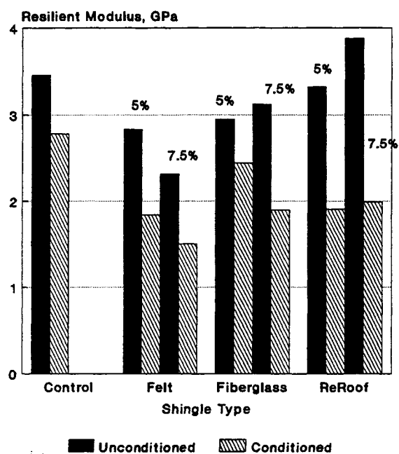
Figure 12. Moisture Sensitivity (Resilient Modulus) of Dense Graded Mixtures, 85/100 AC.
