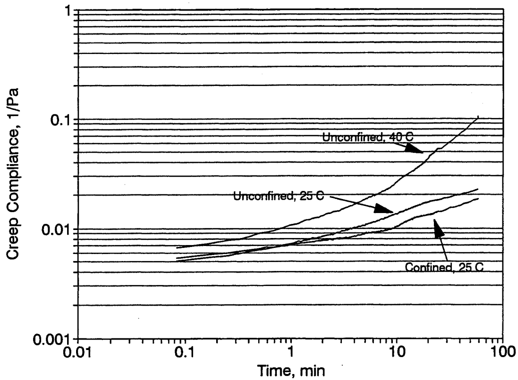
Figure 29. Creep Compliance Curves for SMA Mixtures, Fiberglass Shingles.
