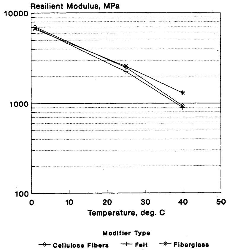
Figure 10. Temperature Susceptibility for SMA Mixtures.
