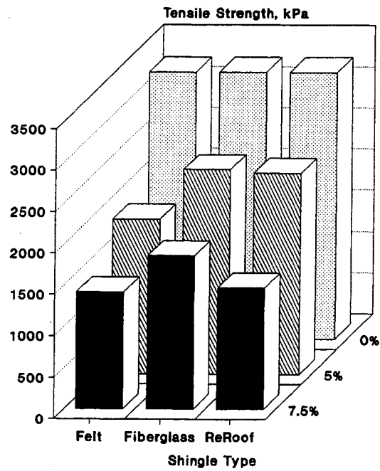
Figure 21. Low Temperature Properties (Peak Tensile Strength) for Dense Graded Mixtures, 85/100 AC.
