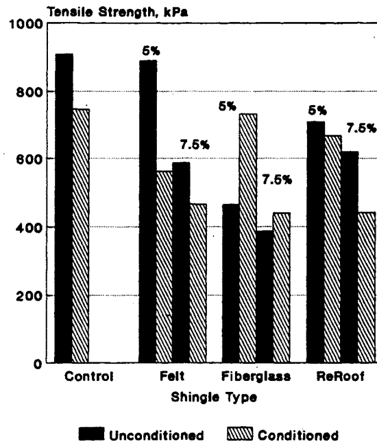
Figure 14. Moisture Sensitivity (Indirect Tensile Strength) of Dense Graded Mixtures, 85/100 AC.
