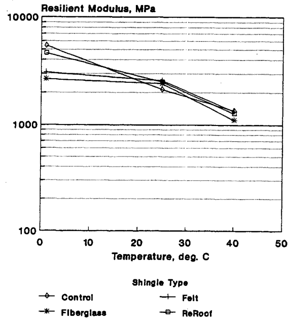
Figure 8. Temperature Susceptibility for Dense Graded Mixtures Containing 5% Shingles, 85/100 AC.
