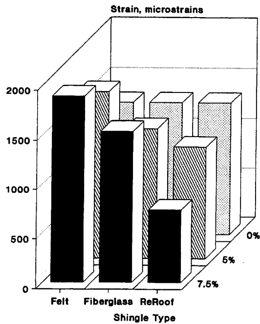
Figure 23. Low Temperature Properties (Strain at Peak Stress) for Dense Graded Mixtures, 85/100 AC.
