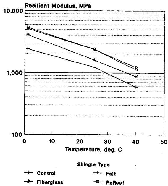
Figure 7. Temperature Susceptibility for Dense Graded Mixtures Containing 7.5% Shingles, 120/150 AC.
