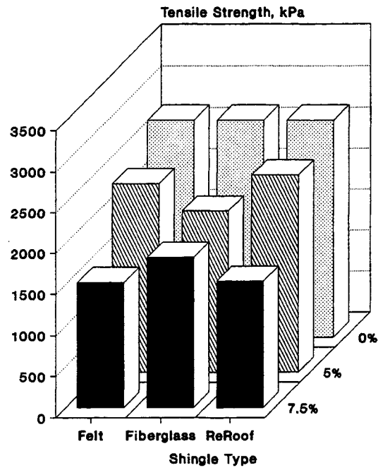
Figure 20. Low Temperature Properties (Peak Tensile Strength) for Dense Graded Mixtures, 120/150 AC.
