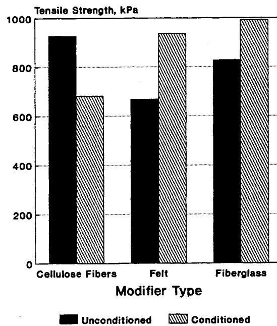
Figure 18. Moisture Sensitivity (Indirect Tensile Strength) for SMA Mixtures.
