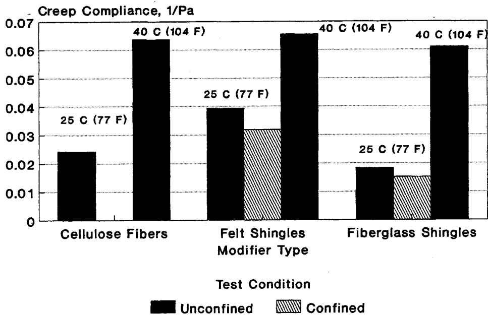
Figure 30. Creep Compliance for SMA Mixtures
