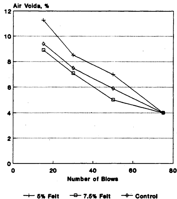
Figure 2. Influence of Compactive Effort on Air Voids for Mixtures Containing Felt Shingles and 85/100 AC.
