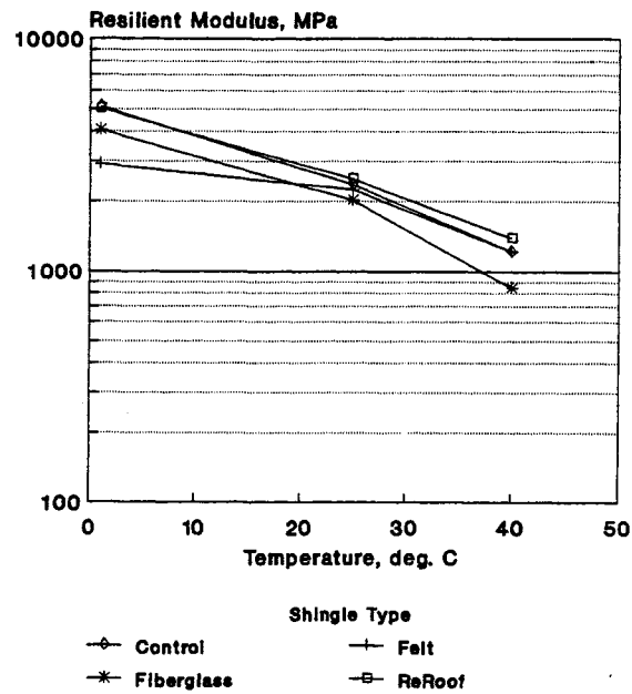
Figure 6. Temperature Susceptibility for Dense Graded Mixtures Containing 5% Shingles, 120/150 AC.
