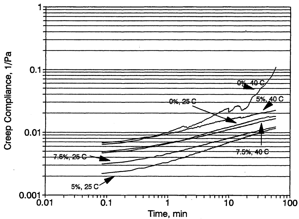
Figure 28. Creep Compliance Curves for Dense Graded Mixtures, Fiberglass Shingles, 120/150 AC.
