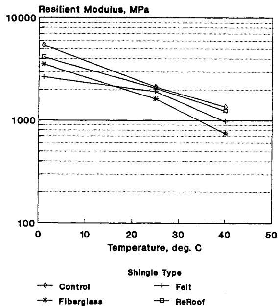
Figure 9. Temperature Susceptibility for Dense Graded Mixtures Containing 7.5% Shingles, 85/100 AC.
