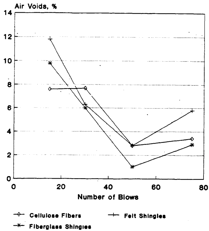
Figure 4. Influence of Compactive Effort on Air Voids for SMA Mixtures.
