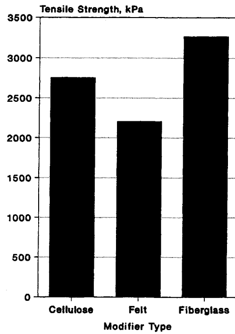
Figure 24. Low Temperature Properties (Peak Tensile Strength) for SMA Mixtures
