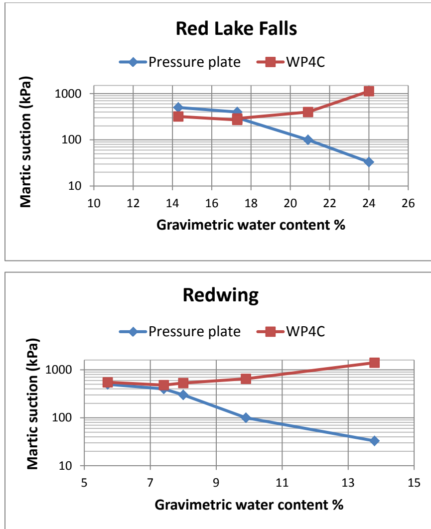
Figure 8. (continued) Graphs for each test soil showing the relationship between the water content and the pressure plate matric and the matric suction given by the WP4C.
