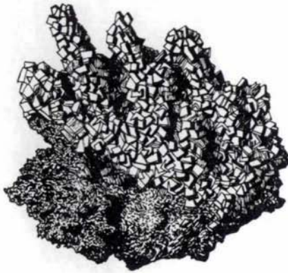
Siderite Rhombs
