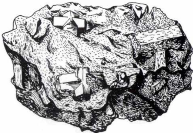
Staurolite Crystals
