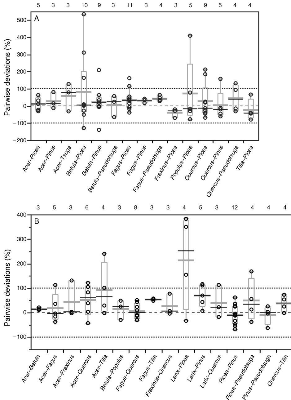
FIG. 2. Differences in net N mineralization ( N_{min} ) rates between co-occurring genera. Positive deviations indicate higher net N_{min} beneath the first genus listed in the pair (e.g., Betula in the Betula-Picea pair). Panel (A) shows DA-EG genus pairs only, with the DA genus always listed first. Panel (B) shows DA-DA and EG-EG pairs, plus pairs of Larix , a deciduous conifer genus, with other genera. For each pair of genera, the number of independent contrasts is listed above the boxplot. Boxplots show the median (horizontal black bar), mean (horizontal gray bar), and 25% and 75% quartiles. Whiskers extend from each quartile to the maximum and minimum values or to the outermost point that does not extend beyond the upper or lower quartile by a value more than 1.5 times the interquartile range. Dashed and dotted lines, respectively, denote 0%, +100%, and -100% on the y-axis.
