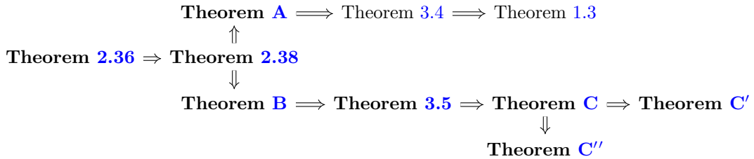
Figure 1.1: Graph of logical dependencies.
