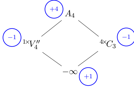
Figure 3.2: Centralizers of cyclic subgroups in A_4 and the Möbius function \mu(-\infty, ?) .
