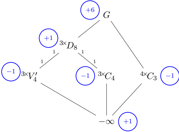
Figure 3.1: Centralizers of cyclic subgroups in S_4 and the Möbius function \mu(-\infty, ?) .
