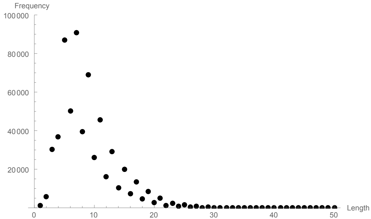
Figure 1: Terminating lengths of \frac{x}{y} ( x, y < 1000 ) with numerator \frac{3}{2} and the max algorithm.
