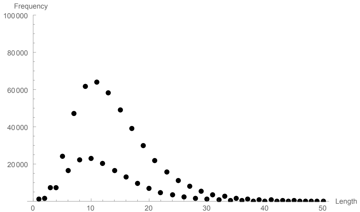
Figure 4: Terminating lengths of \frac{x}{y} ( x, y < 1000 ) with numerator \frac{4}{3} and the min algorithm.
