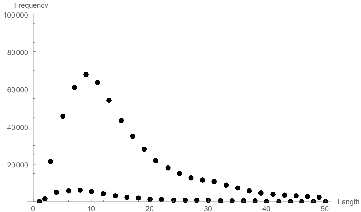
Figure 5: Terminating lengths of \frac{x}{y} ( x, y < 1000 ) with numerator \frac{99}{13} and the max algorithm.
