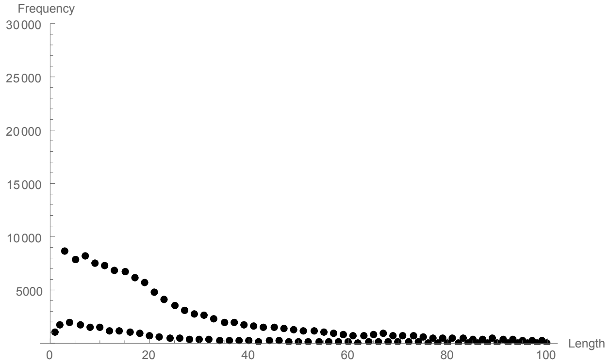
Figure 8: Terminating lengths of \frac{x}{y} ( x, y < 1000 ) with numerator \frac{19}{6} and the max algorithm.
