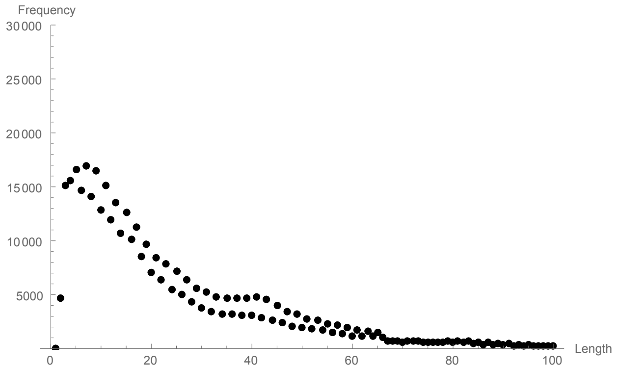
Figure 9: Tail lengths of \frac{x}{y} ( x, y < 1000 ) with numerator \frac{19}{6} and the max algorithm.
