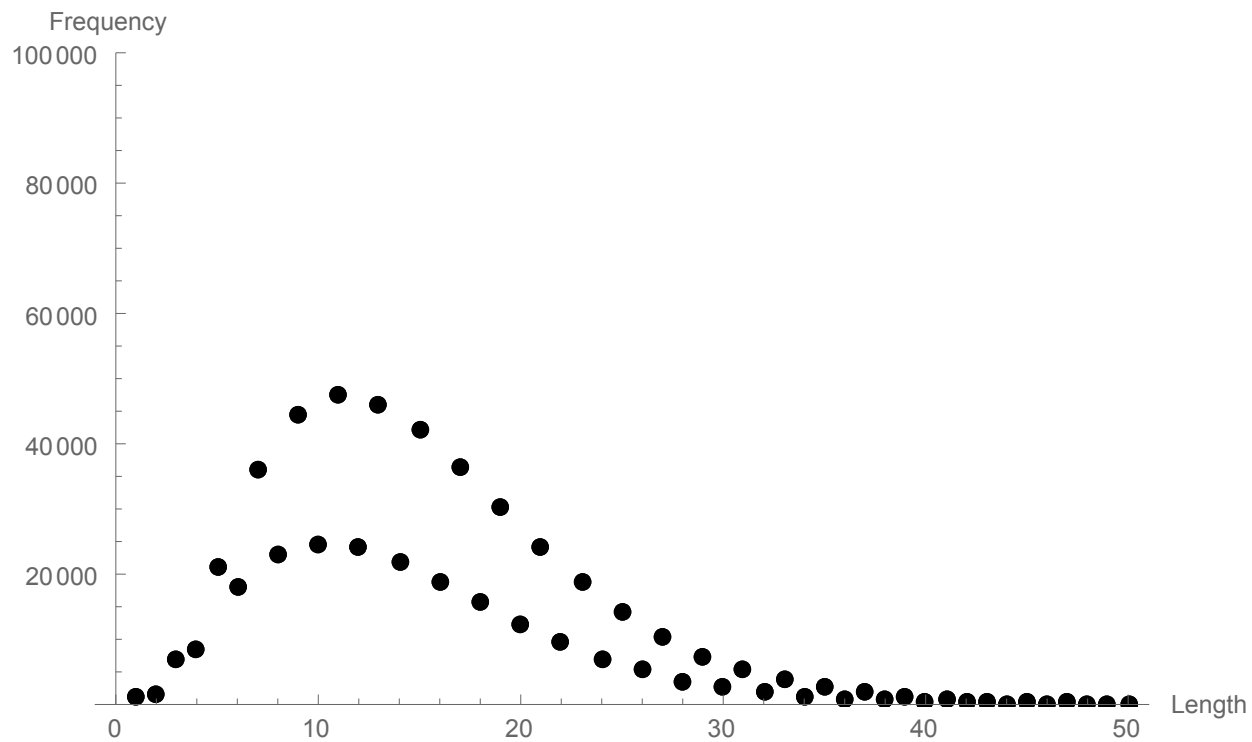
Figure 2: Terminating lengths of \frac{x}{y} ( x, y < 1000 ) with numerator \frac{3}{2} and the min algorithm.
