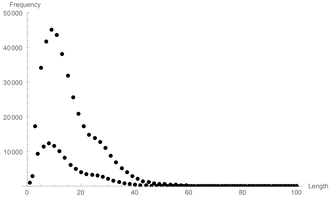
Figure 6: Terminating lengths of \frac{x}{y} ( x, y < 1000 ) with numerator \frac{7}{4} and the max algorithm.
