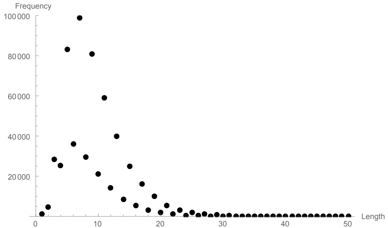
Figure 3: Terminating lengths of \frac{x}{y} ( x, y < 1000 ) with numerator \frac{4}{3} and the max algorithm.
