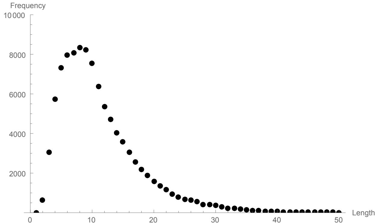
Figure 7: Tail lengths of \frac{x}{y} ( x, y < 1000 ) with numerator \frac{7}{4} and the max algorithm.
