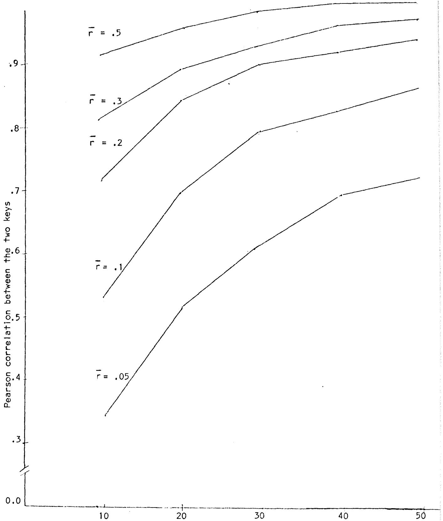
Figure 1. The Pearson correlation between two keys as a function of the common keylength for different values of the common average interitem correlation within key, \bar{r} .
