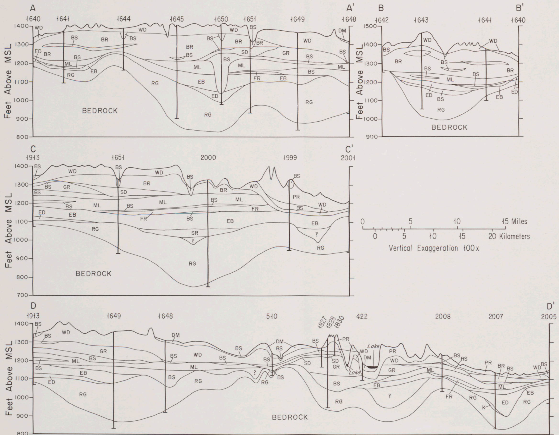
BEDROCK TOPOGRAPHY AND CROSS SECTIONS
