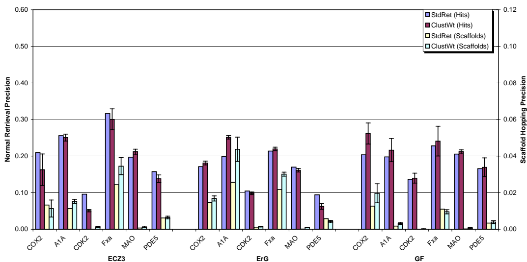
Figure 1: StdRet versus ClustWt.
