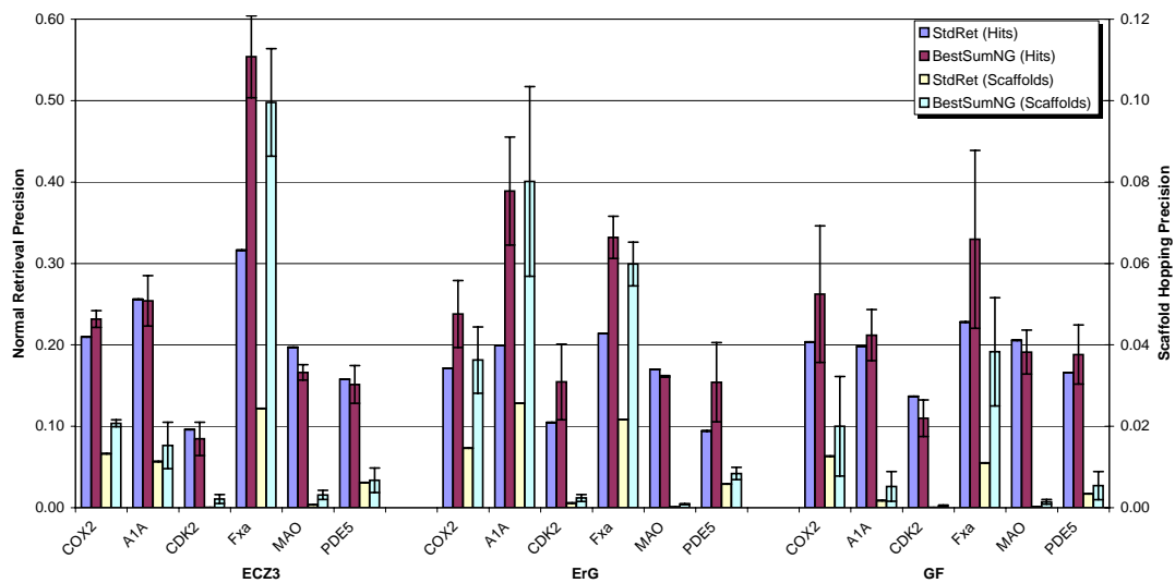
Figure 2: StdRet versus BestSumNG.
