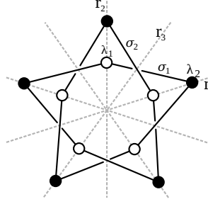
Figure 2.3: System (W, R, \Lambda) with W = I_2(5) and R = \{r_1, r_2\} . The system (W, R) is well-framed for some nonreal \Lambda = \{\lambda_1, \lambda_2\} \subset \mathbb{C}^2 , but not for any real \Lambda \subset \mathbb{R}^2 .
