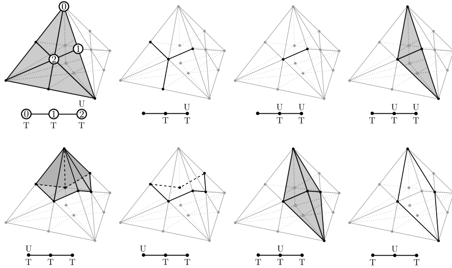
Figure 3.1: A sampling of \Delta_T^U for W = \mathfrak{S}_4 .
