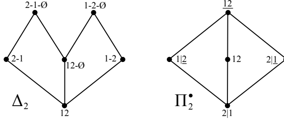
Figure 3.3: Ehrenborg and Jung’s pointed objects.
