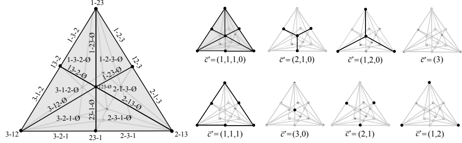
Figure 3.7: Ehrenborg and Jung’s \Delta_{\vec{c}} for all possible choices of \vec{c} \vdash 3 (with last part is allowed to be 0).
