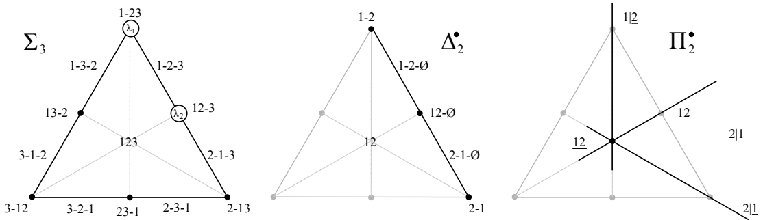
Figure 3.6: The geometry of Ehrenborg and Jung's \Delta_2 and \Pi_2^\bullet from Figure 3.3.
