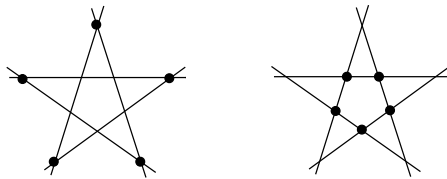
Figure 5.1: Two regular polygons with symmetry group I_2(5) .
