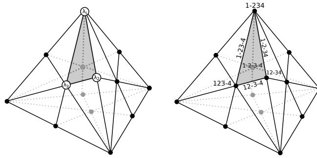
Figure 3.5: The chamber \Lambda_R with vertices \lambda_1, \lambda_2, \lambda_3 (left) and its image under \phi (right) in the case when W = \mathfrak{S}_4 .
