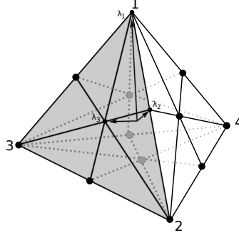
Figure 3.4: W = \mathfrak{S}_4 with the subdivision of facet \mathcal{P}_2 shaded.
