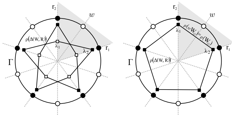
Figure 2.2: Systems (W, R, \Lambda) that are not well-framed for W = I_2(5) , R = \{r_1, r_2\} , and real \Lambda = \{\lambda_1, \lambda_2\} .
