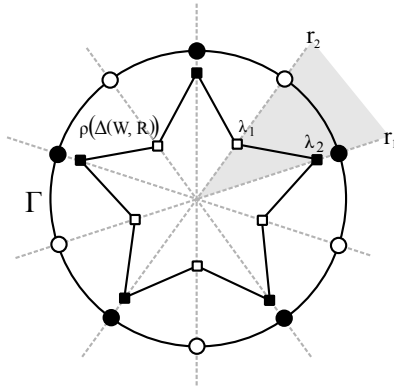
Figure 2.1: A well-framed system and shaded Weyl chamber for I_2(5) .
