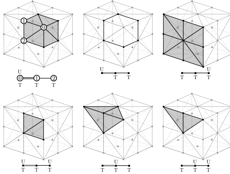
Figure 3.2: A sampling of \Delta_T^U for W = \mathbb{Z}/2\mathbb{Z} \wr \mathcal{E}_3 .
