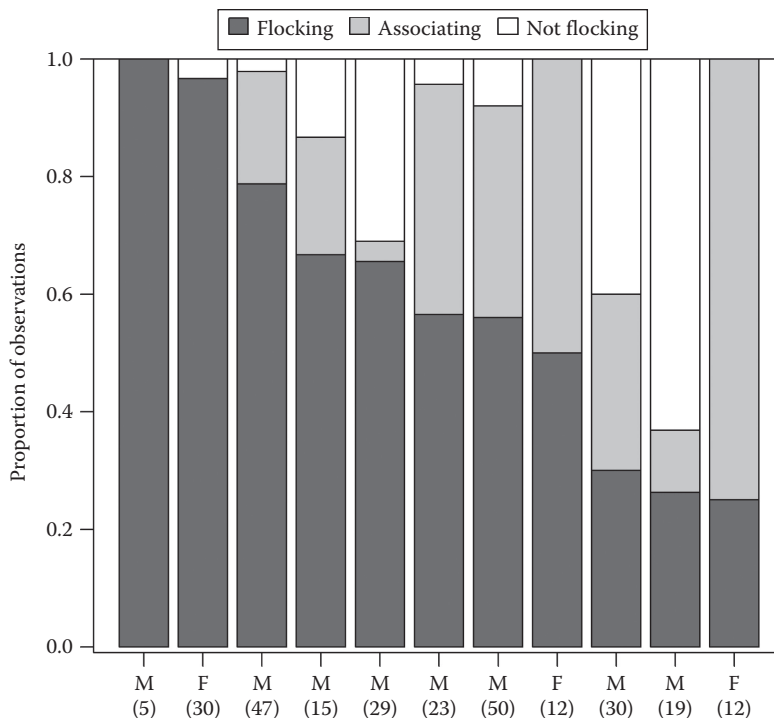
Figure 11.6. Proportion of observations in which 11 individual Golden-winged Warblers were flocking in Costa Rica during the nonbreeding season. Associating refers to cases where an individual occurred with other species but was not moving together in concert. Individuals are ranked by propensity for flocking and referenced by sex (M, male; F, female) with sample size of observations in parentheses.
