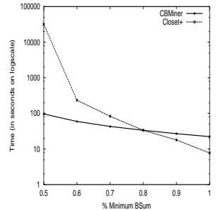
Fig. 11. Runtime ( sports ).
