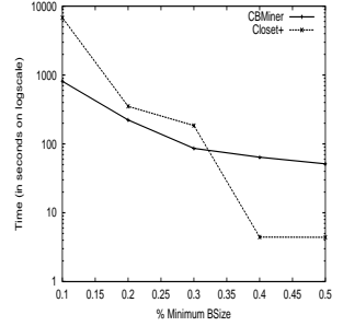
Fig. 9. Runtime ( T40I10D100K ).
