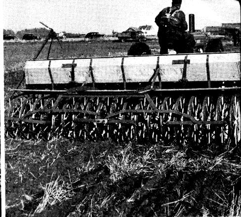
FIG. 8. (LEFT) THE BASIN TILLER ROUGHENS THE SURFACE (RIGHT) THE PRESS DRILL PACKS LIKE A SUBSURFACE PACKER
