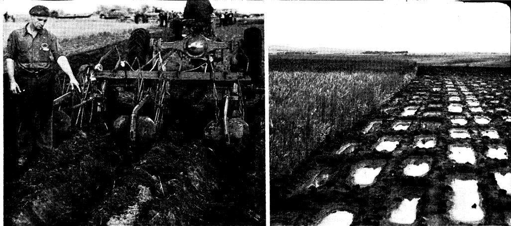
FIG. 12. (LEFT) HOW THE BASIN LISTER OPERATES (RIGHT) WORK OF THE BASIN LISTER
