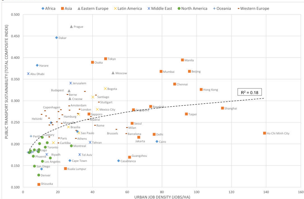
Figure 3: Aggregate sustainability of public transport by population and job density
