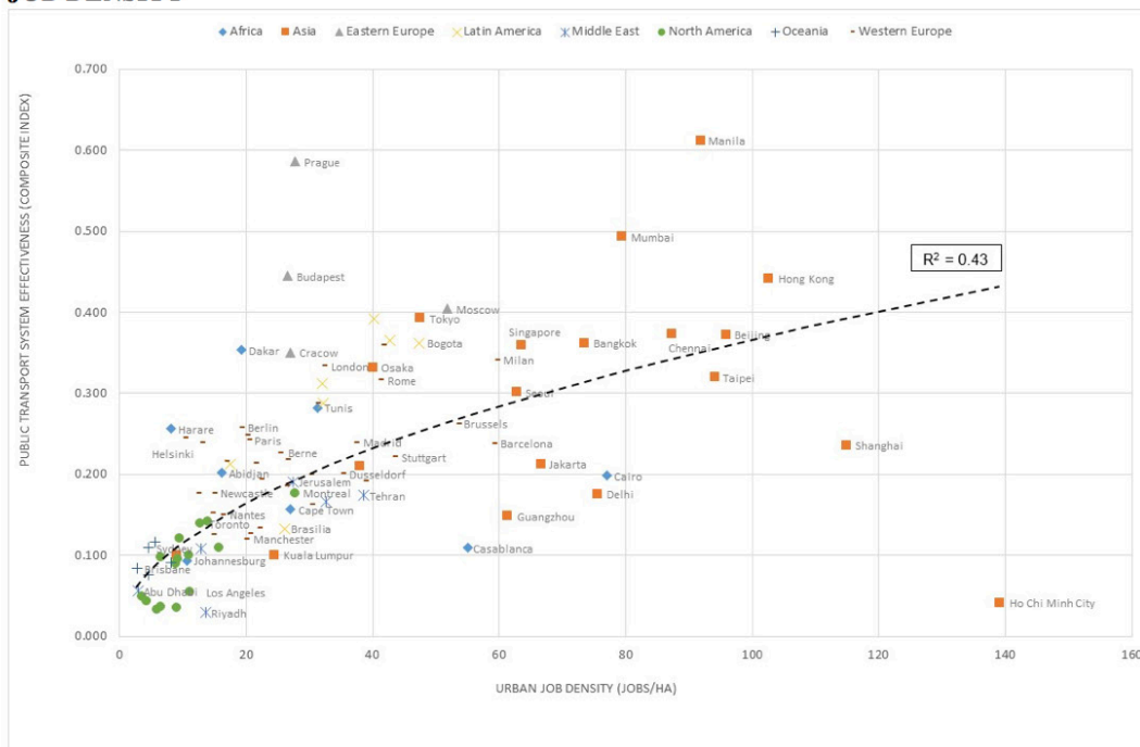
Figure 4: Aggregate system effectiveness sustainability of public transport by population and job density
