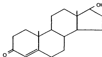
TESTOSTERONE
