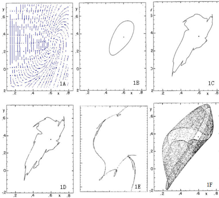
Figure 1. A. The phase portrait of dx/dt = 0.36x - xy , dy/dt = x^2 - y with x(0) = y(0) = 1 . B. The attractor of X_{n+1} = (1 + 36t)X_n - tX_nY_n , Y_{n+1} = (1-t)Y_n + tX_n^2 with t = 1.50 C. Same as B, but t = 1.775 D. Same as C, but t = 1.785 E. Magnification of 1D F. Same as D, but t = 1.92
