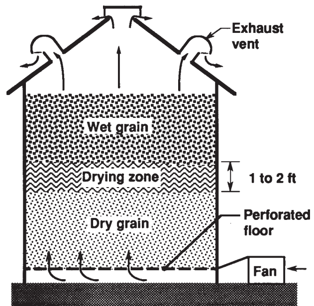
Figure 1. Schematic of natural-air drying bin.
