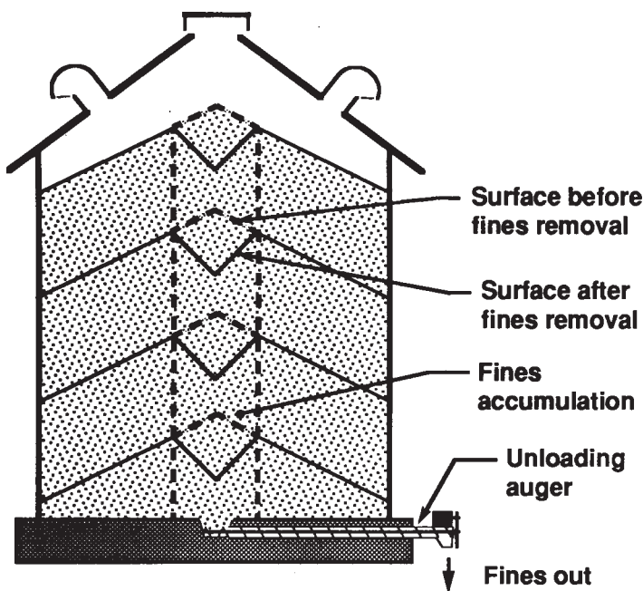
Figure 2. Removing fines during bin filling.
