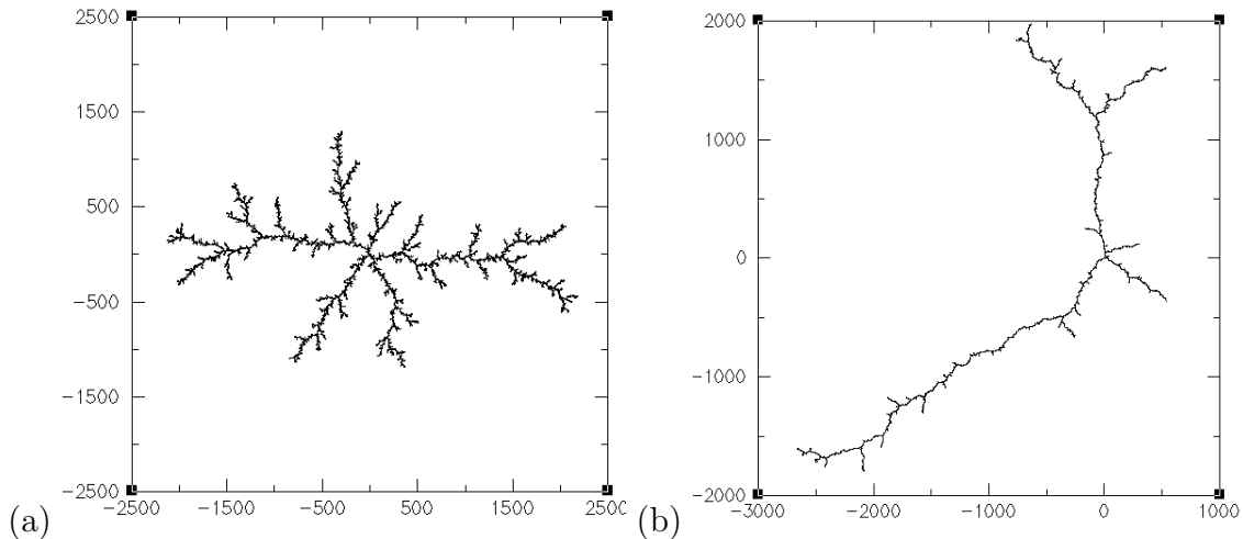
Figure 10: Conformal-mapping simulations by Hastings (2001) of the Dielectric Breakdown Model with (a) \eta = 2 and (b) \eta = 3.5 . [Courtesy of Matt Hastings.]
