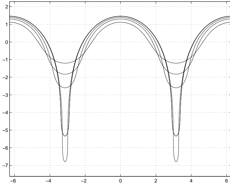
Figure 3: Conformal-map dynamics for the strongly nonlinear regime of the Richtmyer-Meshkov instability (Yoshikawa and Balk (1999)). [Courtesy of Toshio Yoshikawa and Alexander Balk.]
