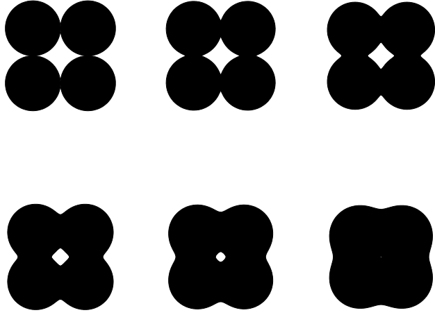
Figure 6: The coalescence of fluid blobs and collapse of cylindrical pores in a model of viscous sintering. This sequence of images shows an analytical solution by Crowdy (2003) using complex-variable methods.
