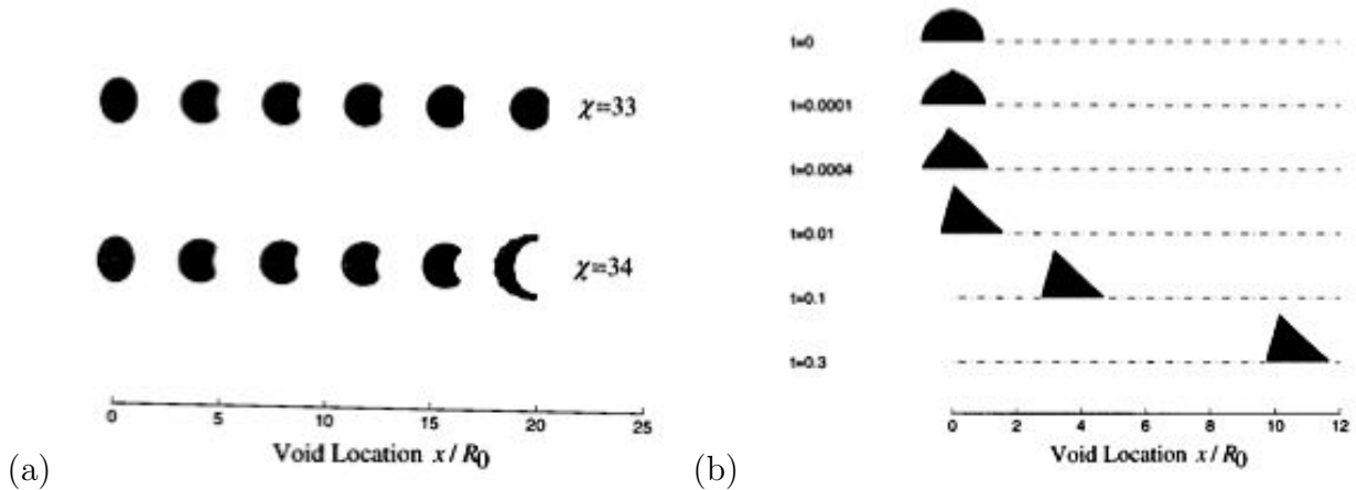
Figure 4: Numerical conformal-mapping simulations of the electromigration of voids in aluminum interconnects (Wang et al. (1996)). (a) A small shape perturbation of a cylindrical void decaying (above) or deforming into a curved slit (below), depending on a dimensionless group, \chi , comparing the electron wind to surface-tension gradients. (b) A void evolving with anisotropic surface diffusivity ( \chi = 100, g_d = 100, m = 3 ). [Courtesy of Zhigang Suo.]
