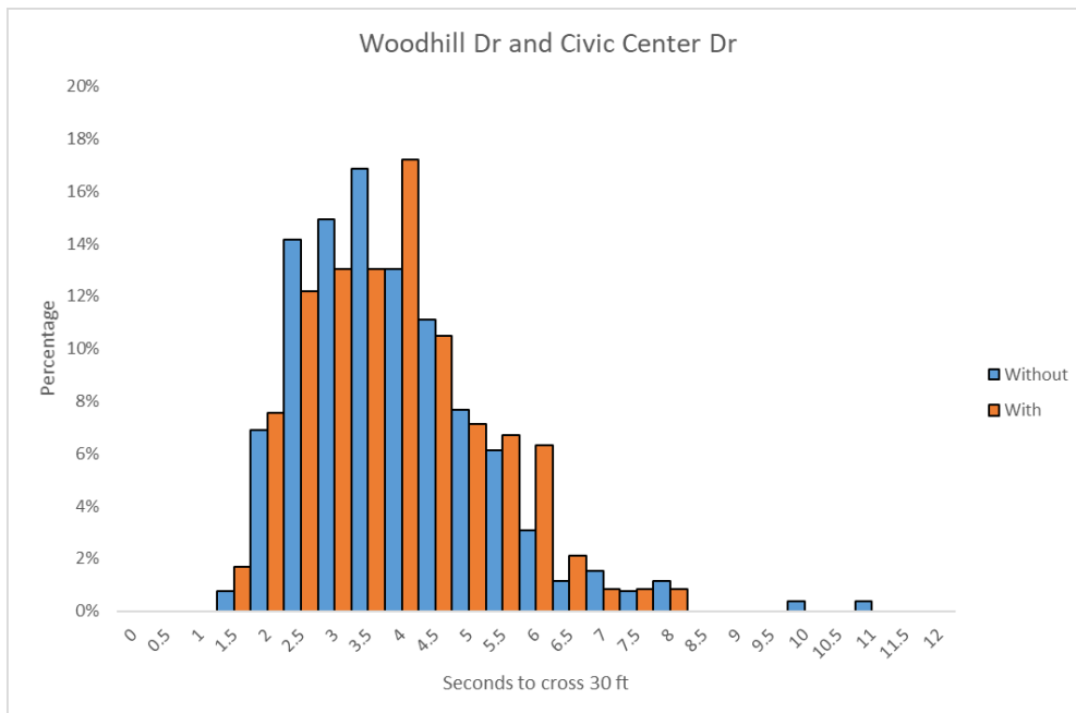
Figure 3.37 Woodhill Dr and Civic Center Dr Histogram of Roll and Ignore behaviors, in seconds to travel 30 ft
