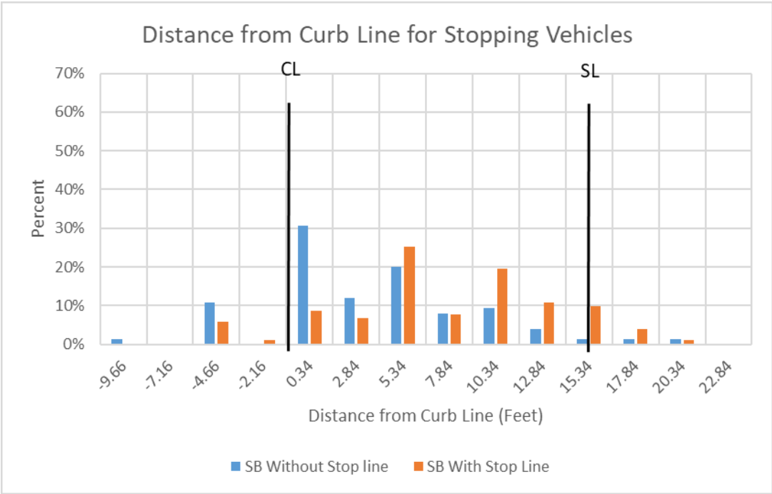
Figure 3.108 Raleigh Ave SB and W 28 th St Distribution of Stopping Distance During Stop Events
