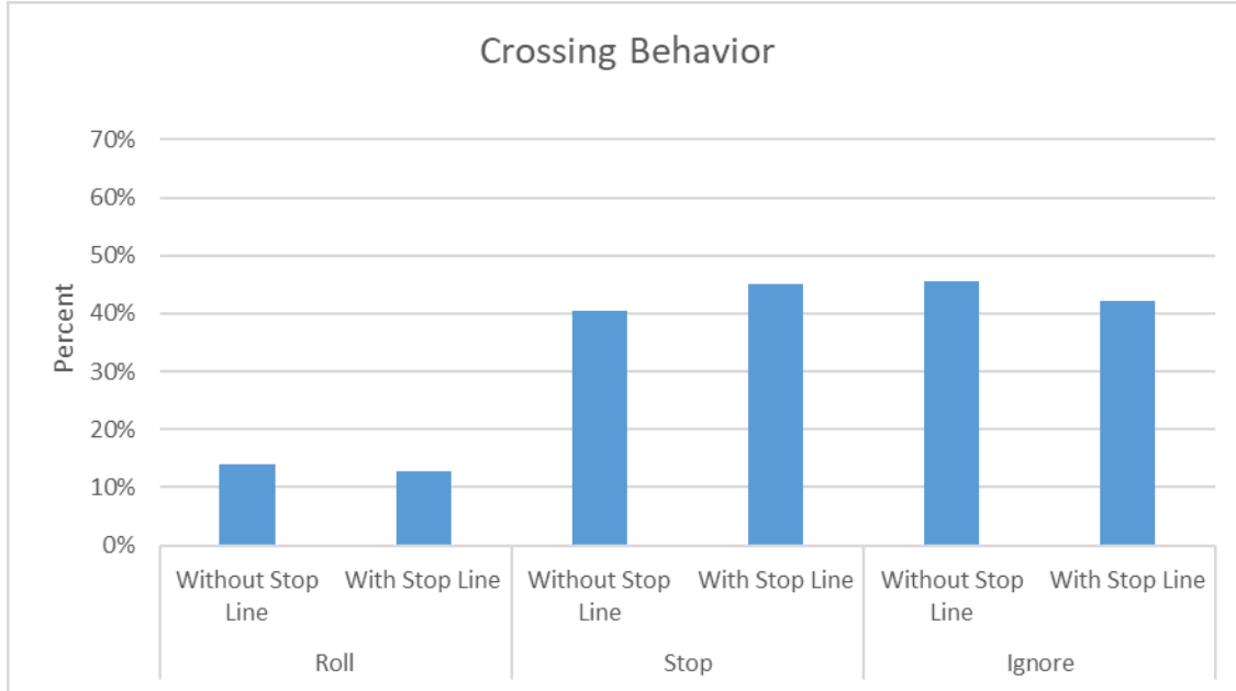
Figure 3.84 Warner Rd and Fish Hatchery Rd N distribution of driver crossing behavior as a percentage of all events without- vs with-stop line
