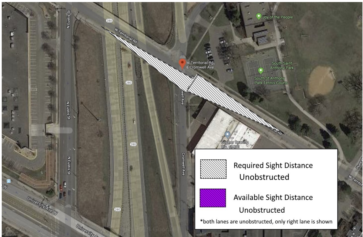
Figure 3.90 Available sight distance and required sight distance at W Territorial Rd and Cromwell Ave
