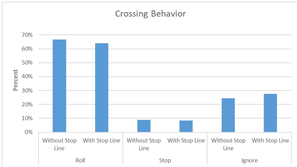
Figure 3.106 Raleigh Ave SB distribution of driver crossing behavior as a percentage of all events without- vs with-stop line
