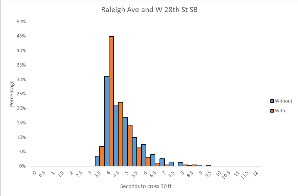
Figure 3.109 Raleigh Ave SB and W 28 th St Histogram of Roll and Ignore behaviors, in seconds to travel 30 ft
