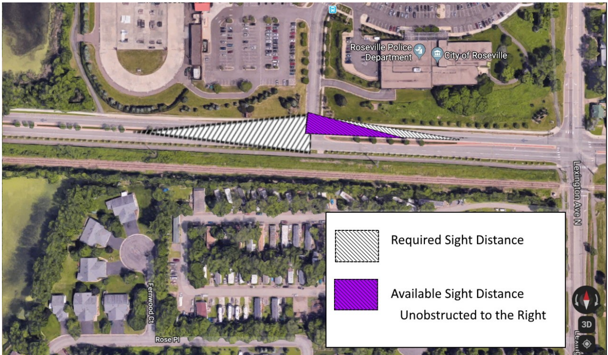
Figure 3.112 Available sight distance and required sight distance at County Rd C W and Civic Center Dr
