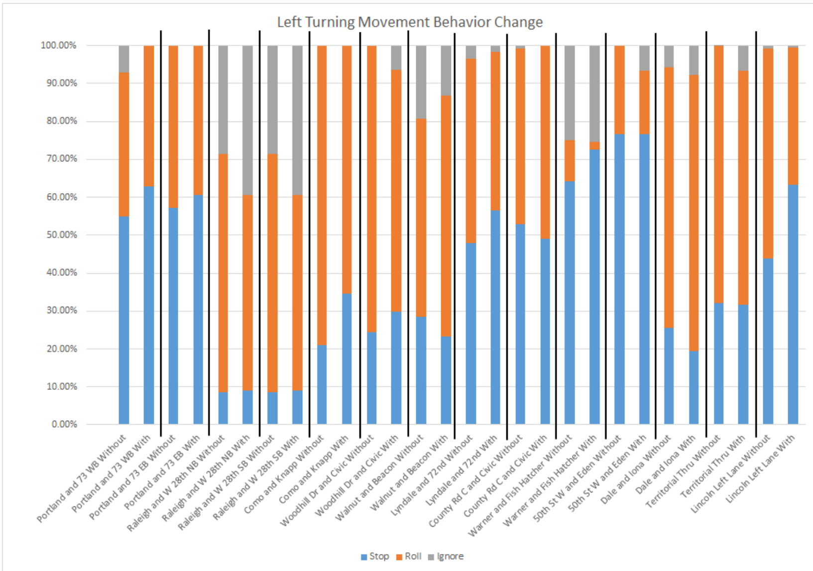
Figure 3.120 Left Turning Movement Crossing Behaviors before and after the Stop Line installation
