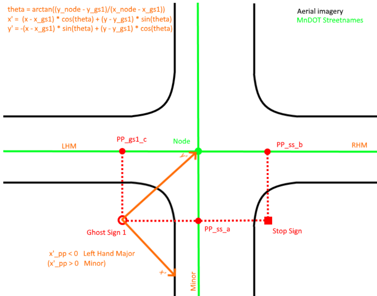
Figure A-0.7 Identification and assignment of approaches – Step 7
