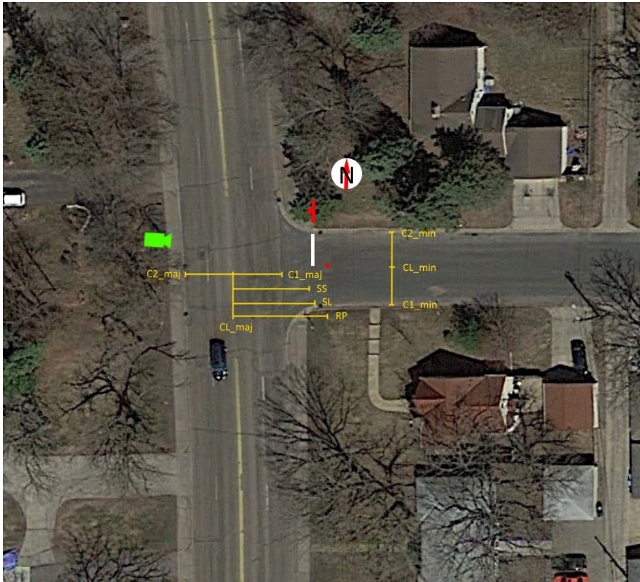
Figure 3.17 – Aerial view of the intersection of Lyndale Ave S and W 72nd St with measurements marked
