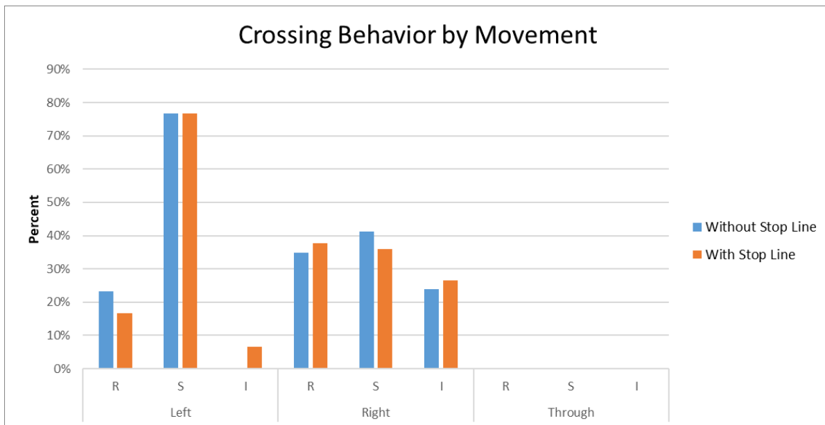
Figure 3.59 50th St W and Eden Ave distribution of driver crossing behavior as a percentage of all events without- vs with-stop line, by driver movement
