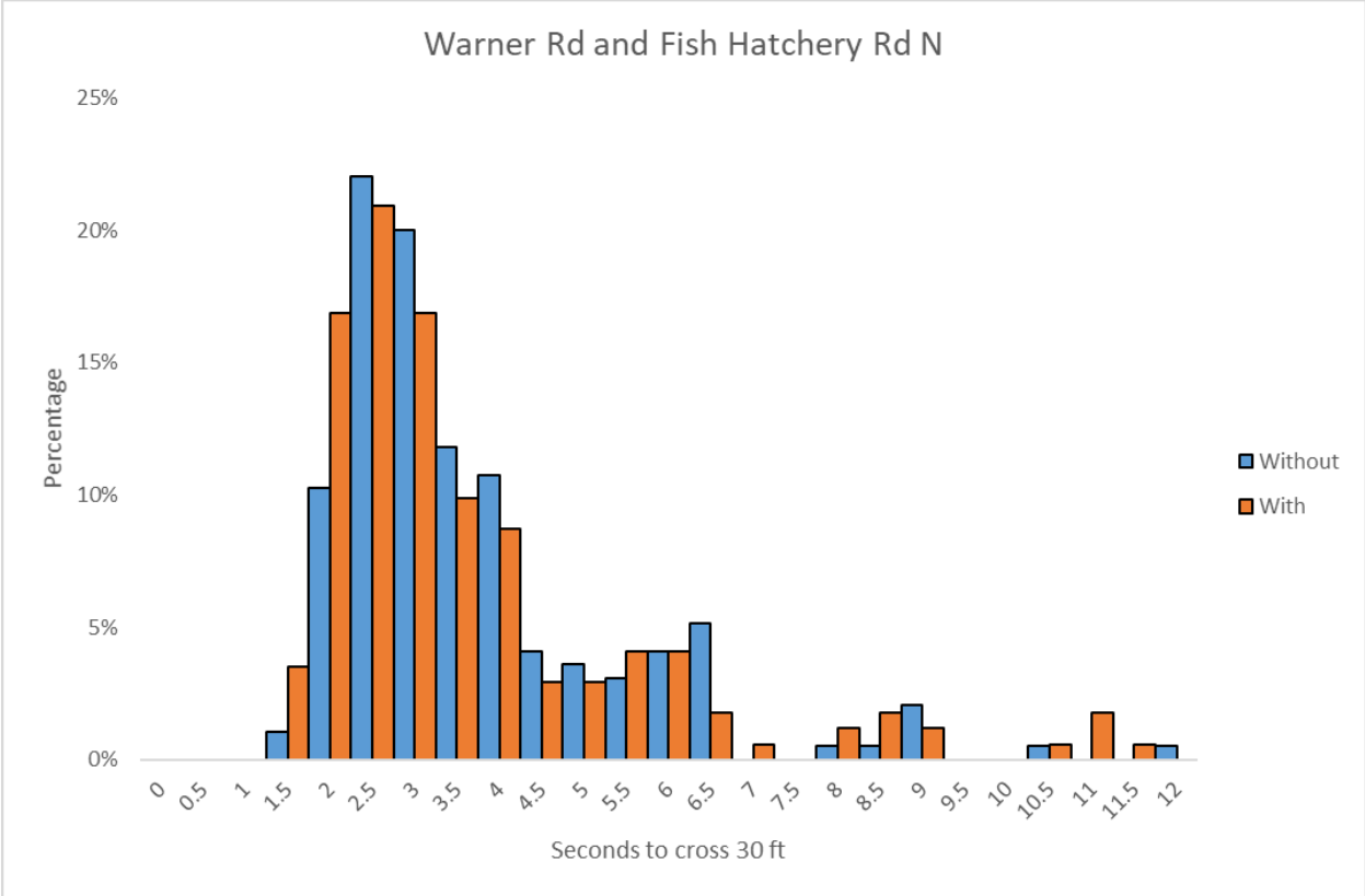
Figure 3.87 Warner Rd and Fish Hatchery Rd N Histogram of Roll and Ignore behaviors, in seconds to travel 30 ft
