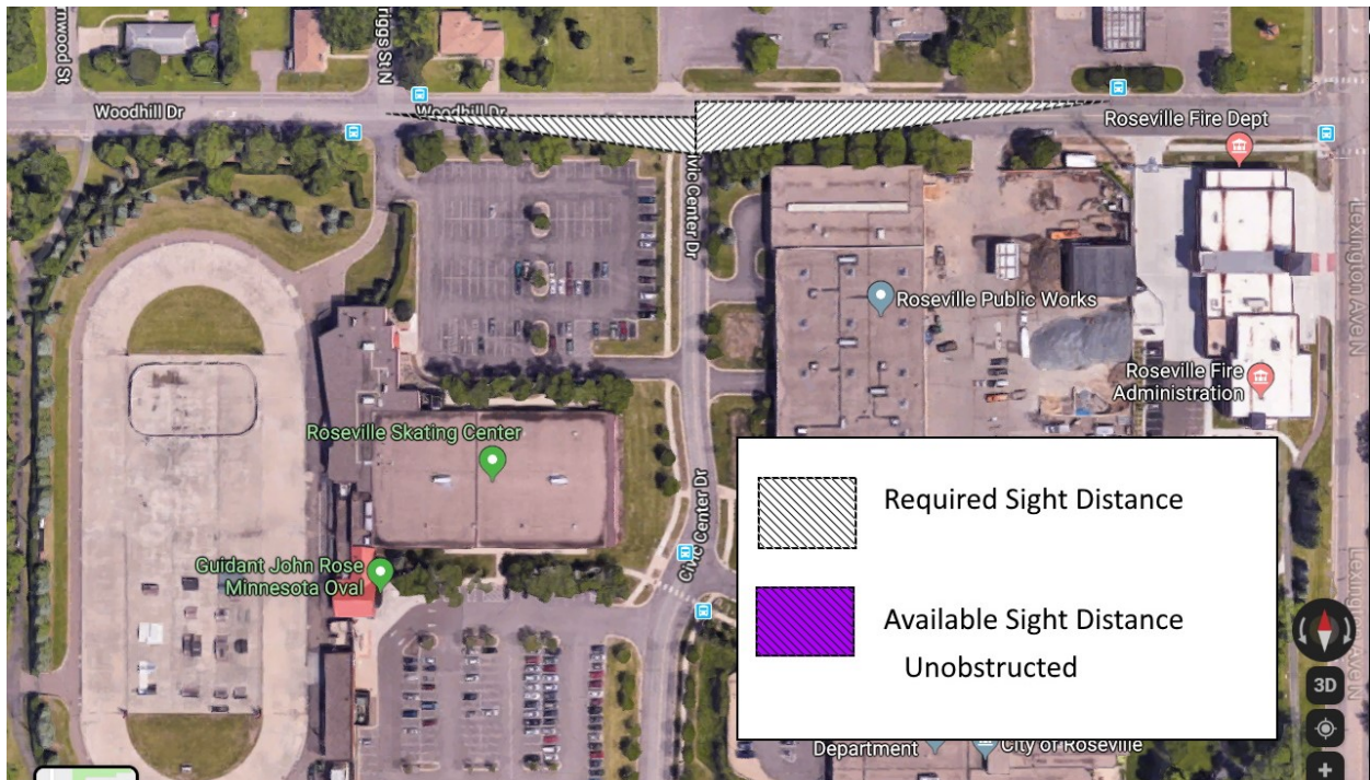
Figure 3.33 Available sight distance and required sight distance at Woodhill Dr and Civic Center Dr
