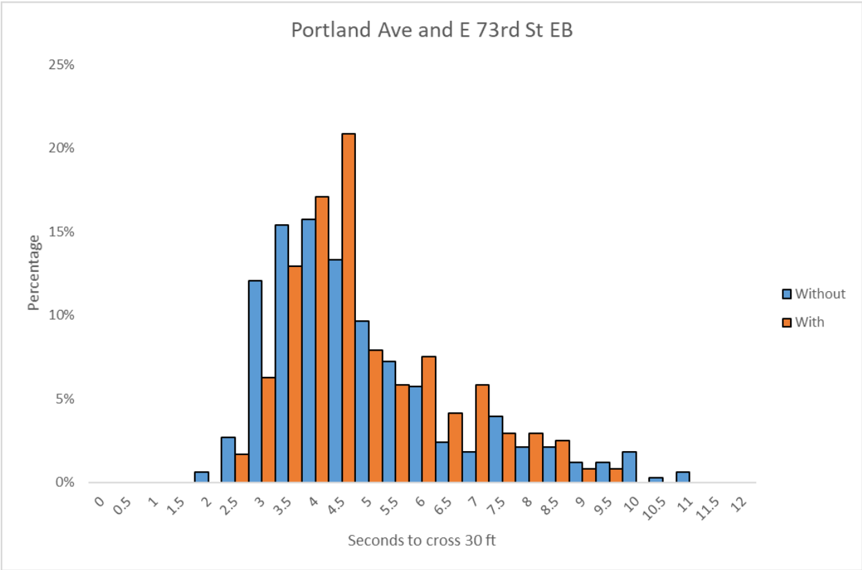
Figure 3.74 Portland Ave and E 73rd St EB Histogram of Roll and Ignore behaviors, in seconds to travel 30 ft
