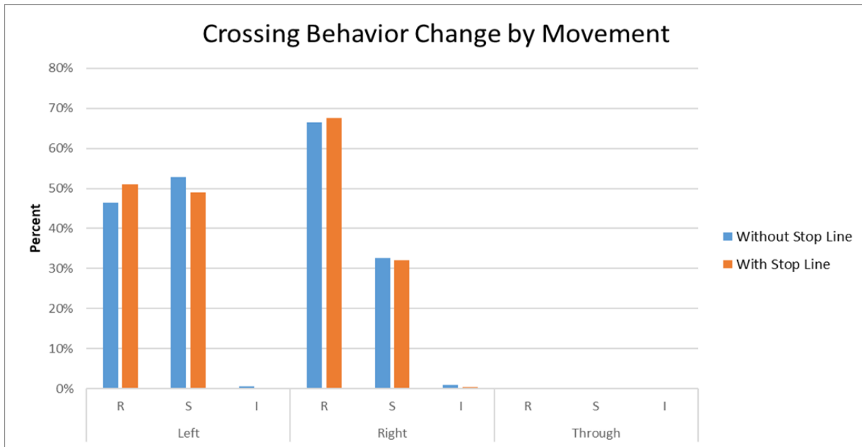
Figure 3.114 County Rd C W and Civic Center Dr distribution of driver crossing behavior as a percentage of all events without- vs with-stop line, by driver movement
