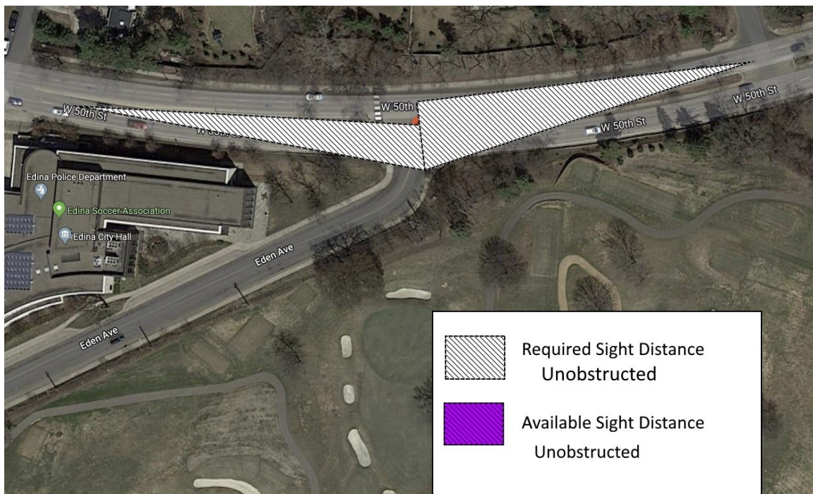
Figure 3.57 Available sight distance and required sight distance at 50th St W
