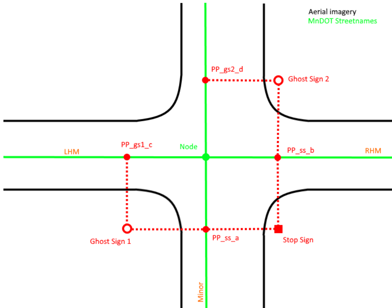
Figure A-0.9 The new ghost sign is projected onto the two nearest polylines.
