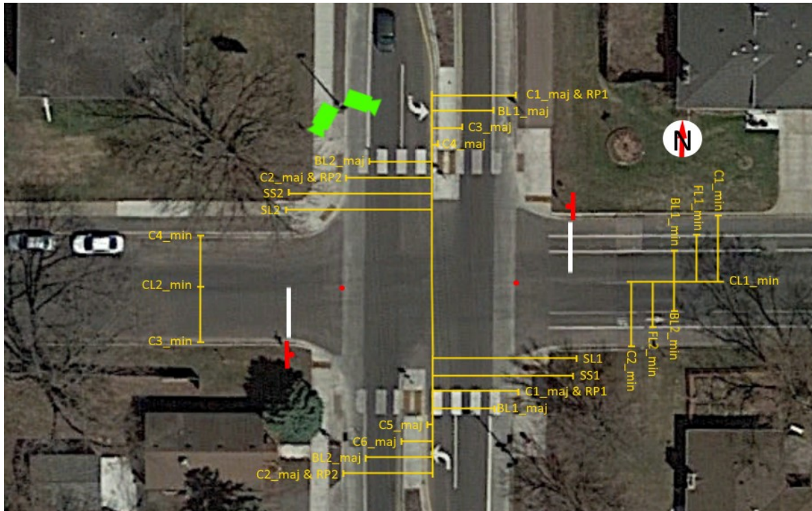
Figure 3.68 Aerial view of the intersection of Portland Ave and E 73 rd St with measurements marked
