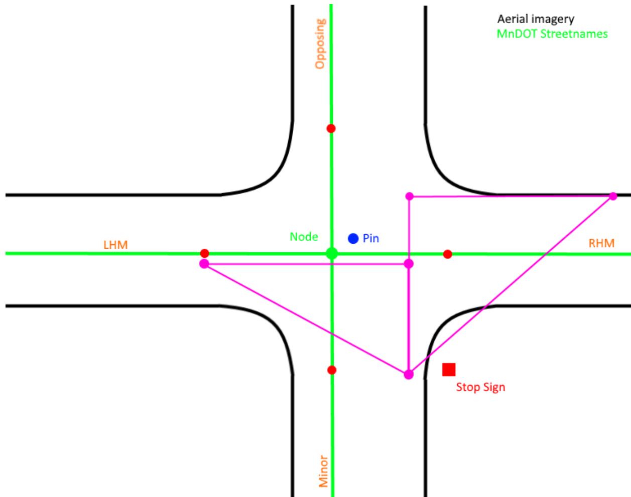
Figure B-0.5 Creation of rudimentary required sight distance triangles – Step 5
