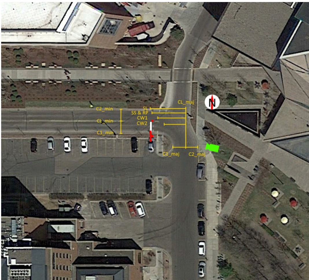
Figure 3.10 Aerial view of the intersection of Walnut St SE and Beacon St SE with measurements marked
