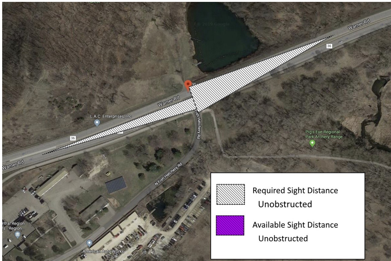
Figure 3.83 Available sight distance and required sight distance at Warner Rd and Fish Hatchery Rd N
