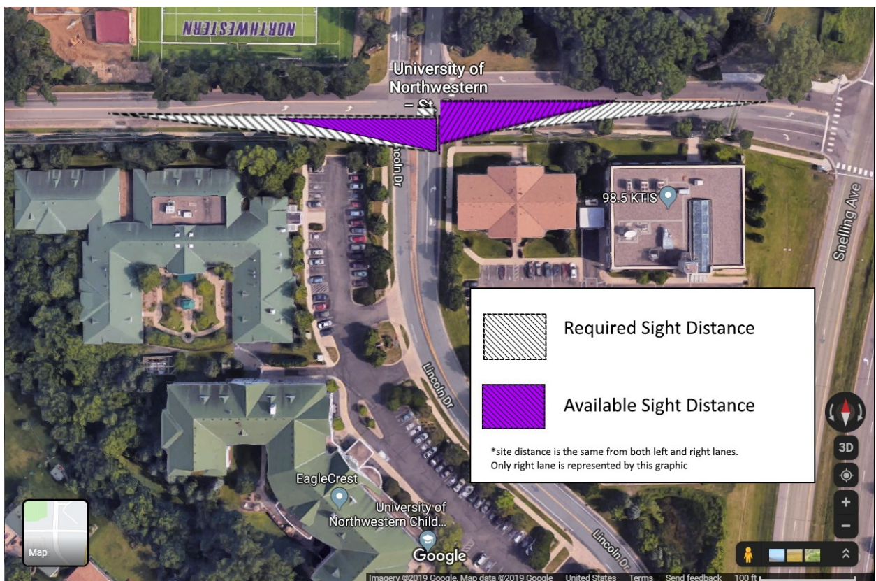
Figure 3.47 Available sight distance and required sight distance at Lincoln Dr and Lydia Ave W, for both left and right lane
