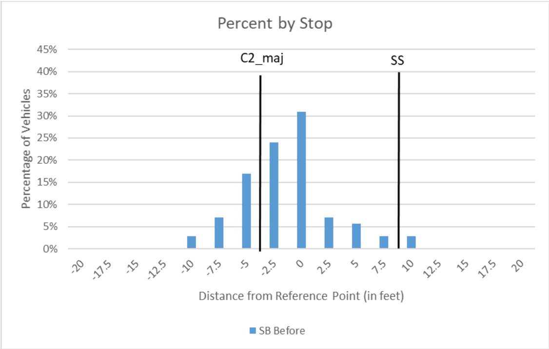
Figure C-0.14 Quentin Ave SB Distribution of Stopping Distance During Stop Events
