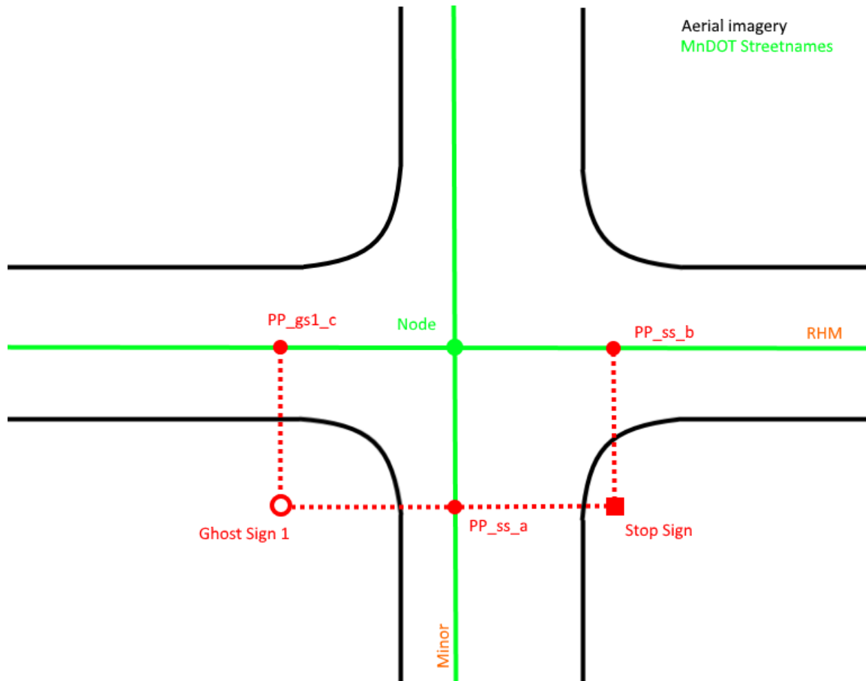
Figure A-0.6 Identification and assignment of approaches – Step 6
