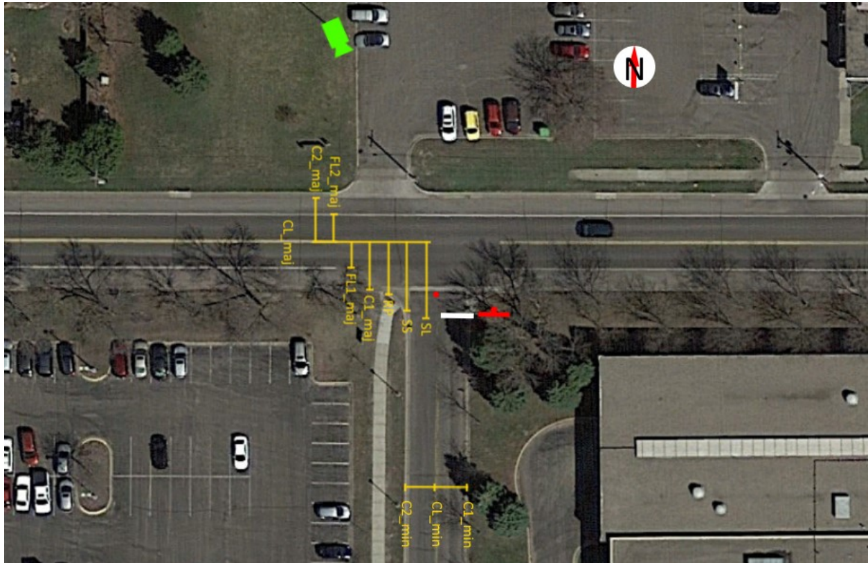
Figure 3.31 Aerial view of the intersection of Woodhill Dr and Civic Center Dr with measurements marked
