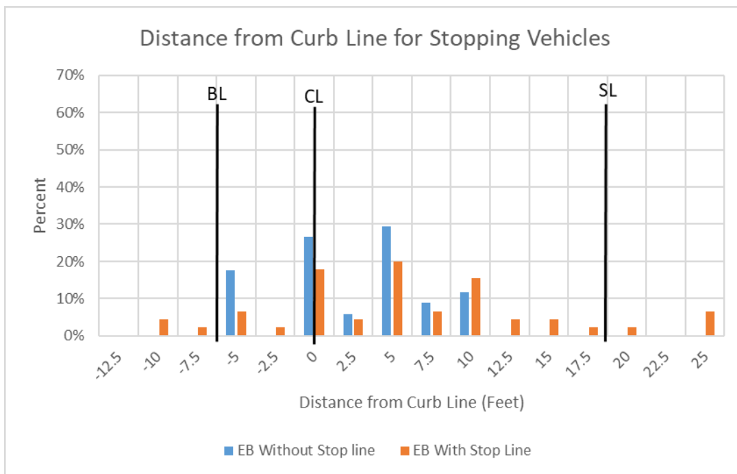
Figure 3.29 Como Ave and Knapp St Distribution of Stopping Distance During Stop Events
