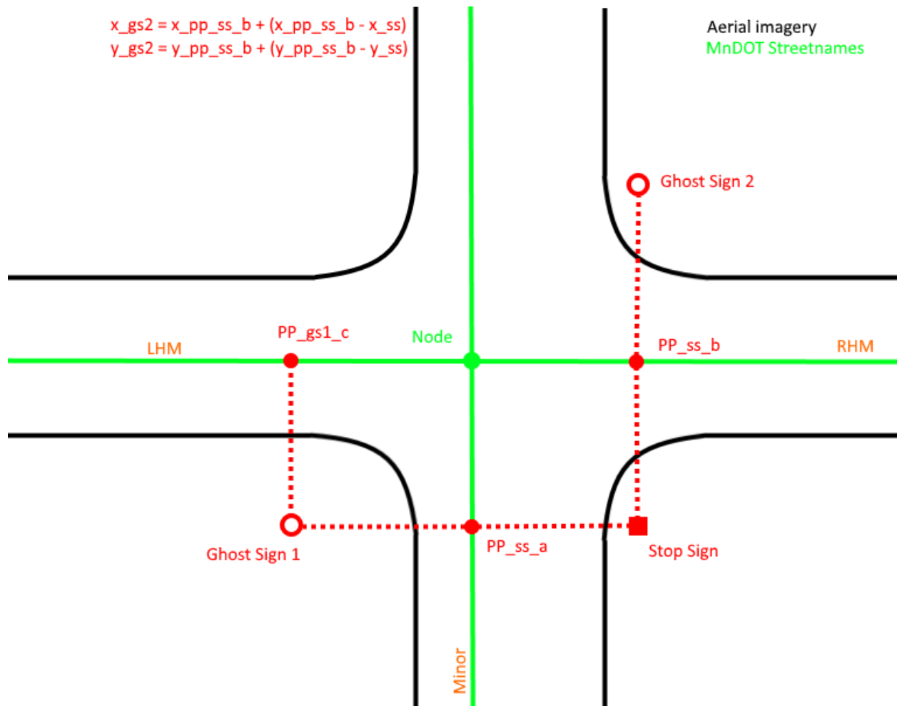
Figure A-0.8 Identification and assignment of approaches – Step 8
