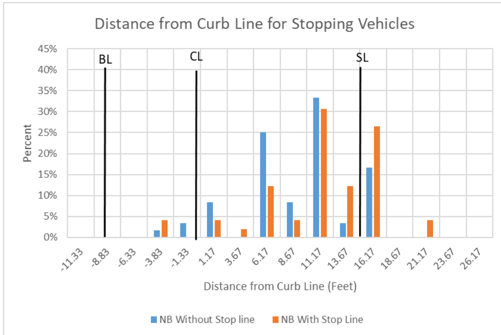
Figure 3.36 Woodhill Dr and Civic Center Dr Distribution of Stopping Distance During Stop Events
