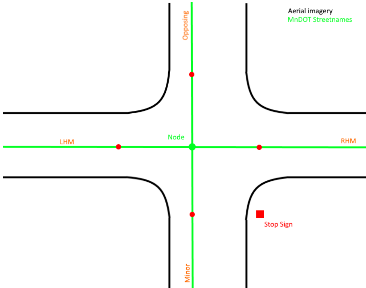
Figure B-0.1 Creation of rudimentary required sight distance triangles – Step 1
