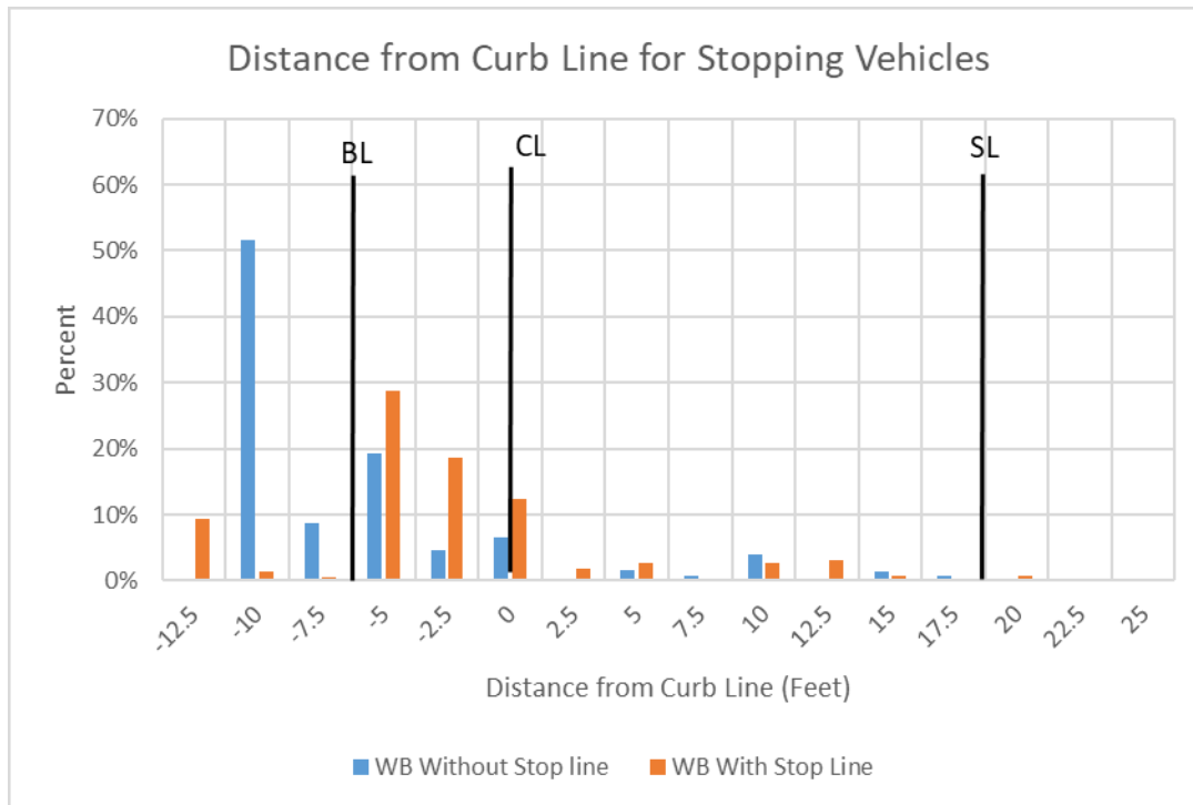
Figure 3.79 Portland Ave and E 73rd St WB Distribution of Stopping Distance During Stop Events
