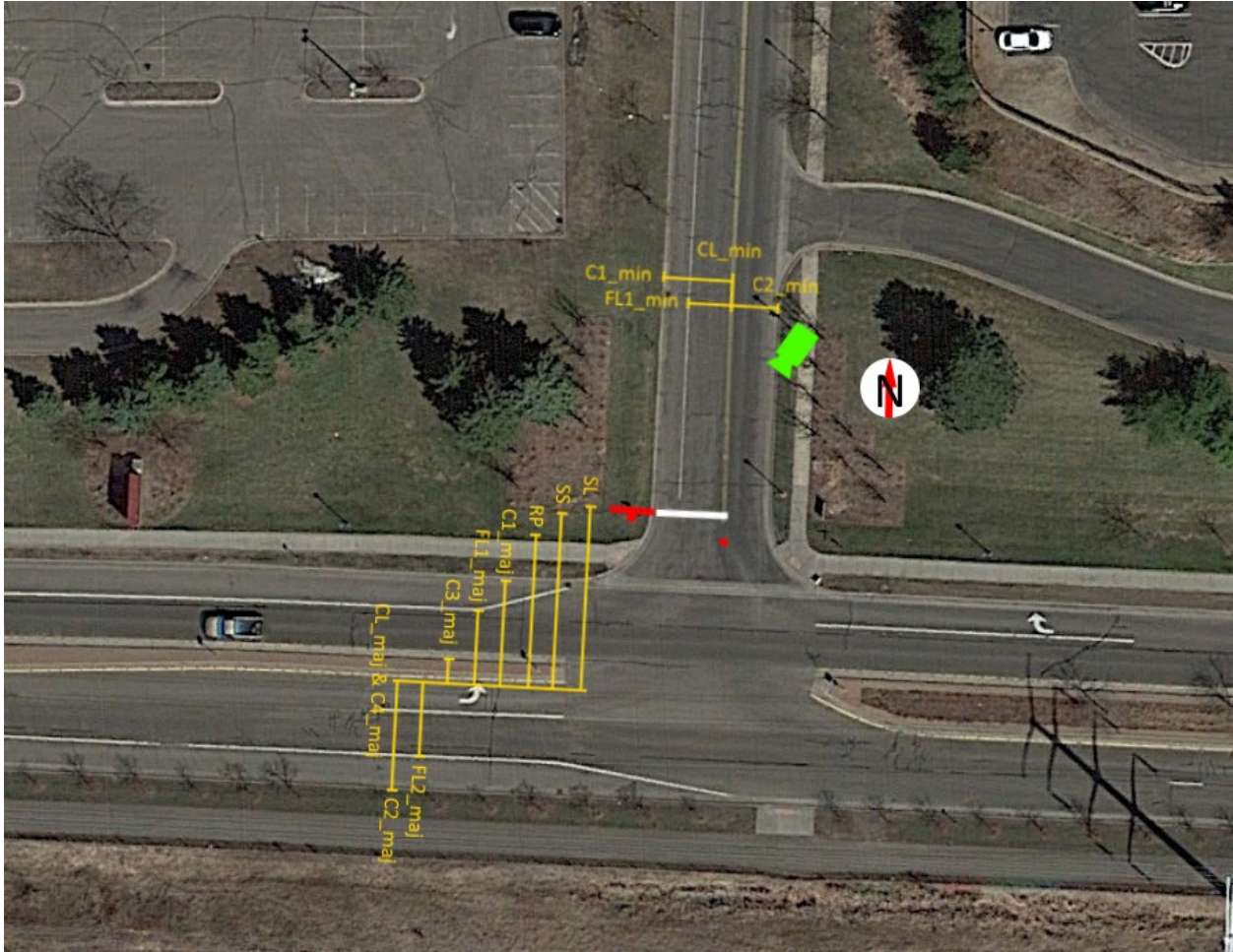
Figure 3.110 Aerial view of the intersection of County Rd C W and Civic Center Dr with measurements marked
