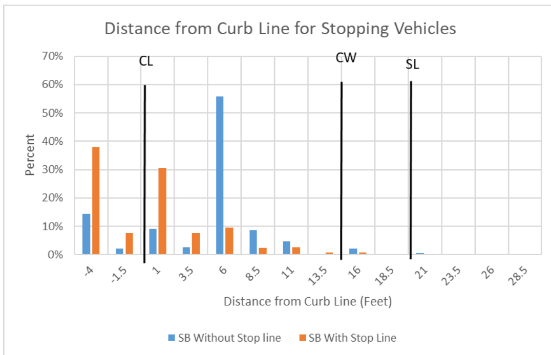
Figure 3.50 Lincoln Dr Left Lane and Lydia Ave W Distribution of Stopping Distance During Stop Events
