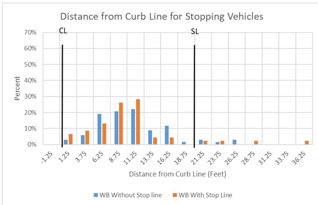
Figure 3.43 Dale St N and Iona Ln Distribution of Stopping Distance During Stop Events
