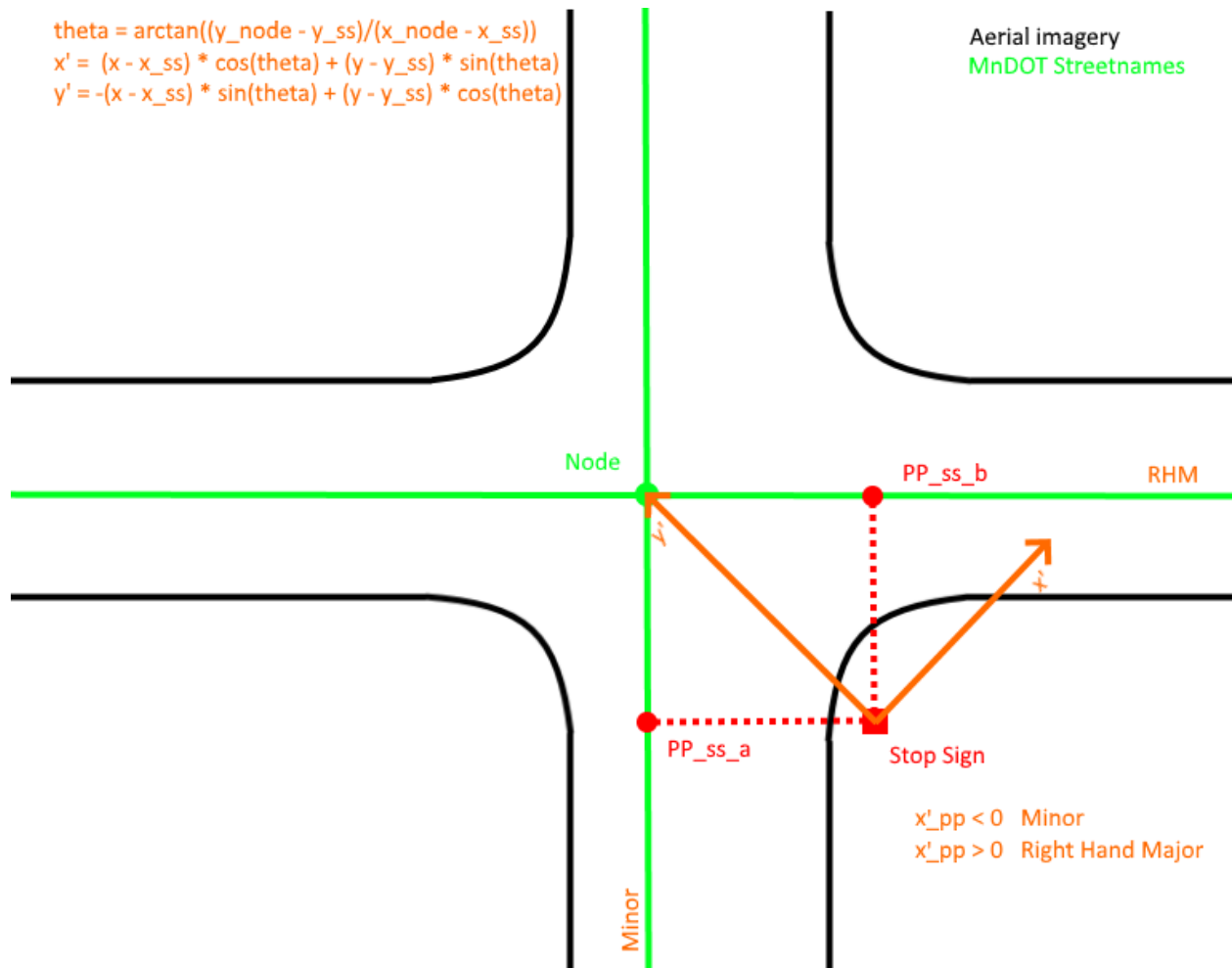
Figure A-0.4 Identification and assignment of approaches – Step 4
