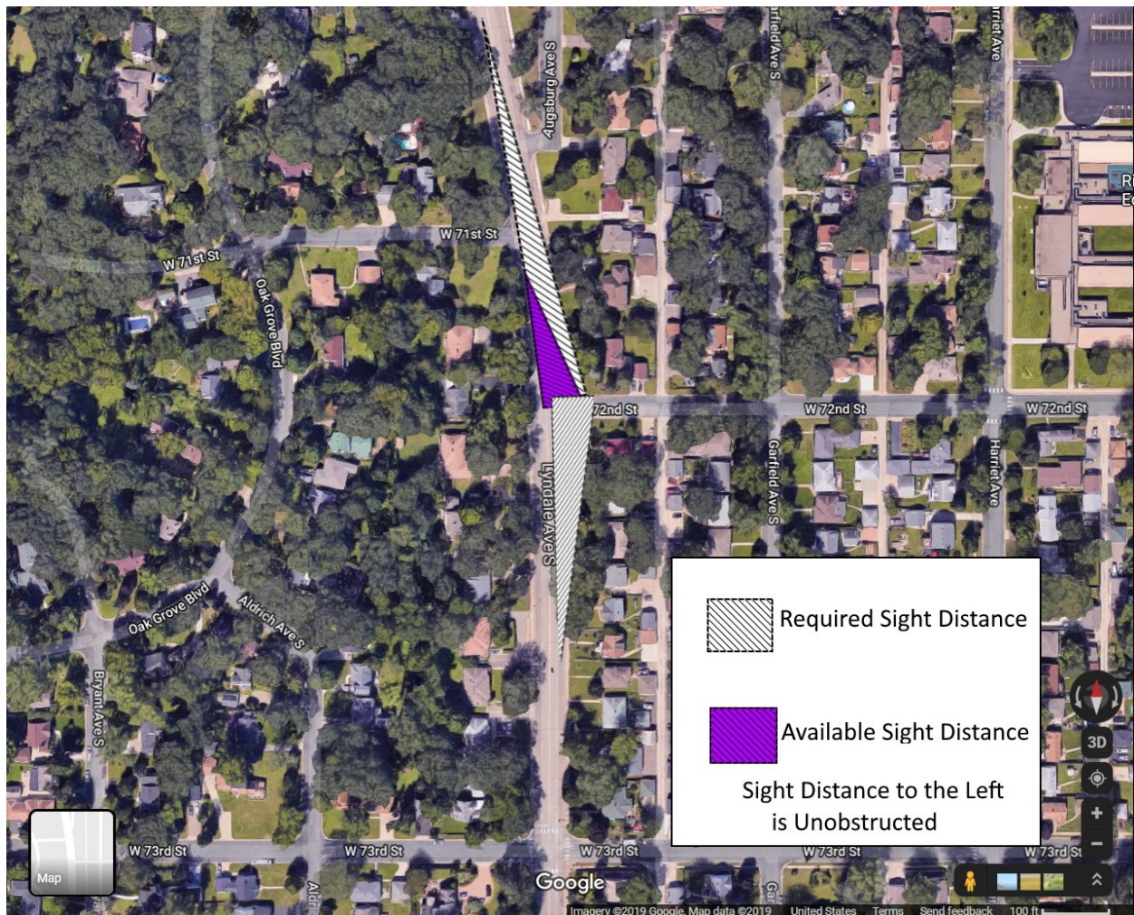
Figure 3.19 Available sight distance and required sight distance at Lyndale Ave S and W 72nd St
