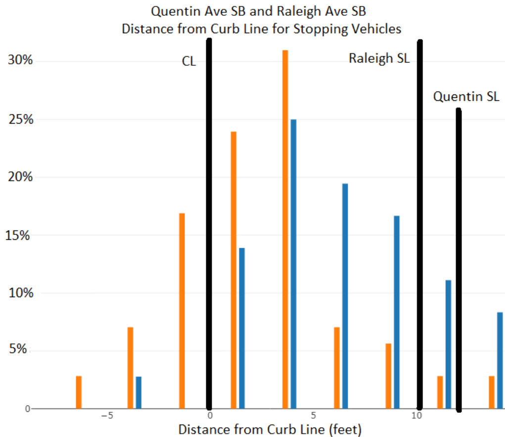
Figure C-0.21 Comparison of Stop Events at Quentin Ave SB and Raleigh Ave SB
