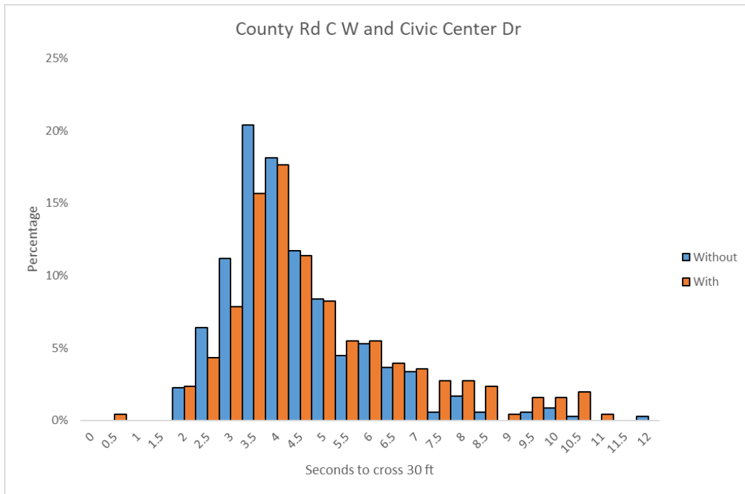
Figure 3.116 County Rd C W and Civic Center Dr Histogram of Roll and Ignore behaviors, (sec over 30ft)
