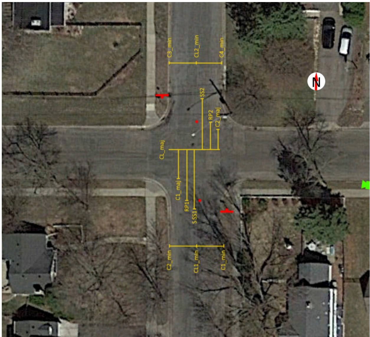
Figure C-0.5 Aerial view of Quentin Ave NB and SB with measurements
