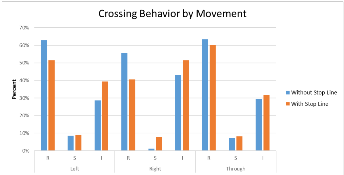
Figure 3.102 Raleigh Ave NB distribution of driver crossing behavior as a percentage of all events without- vs with-stop line, by driver movement
