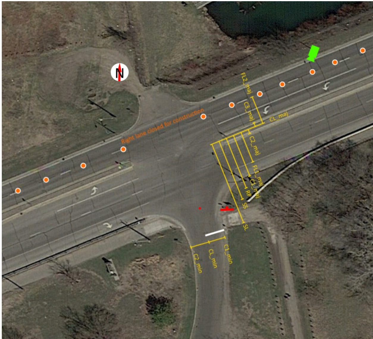
Figure 3.81 Aerial view of the intersection of Warner Rd and Fish Hatchery Rd N with measurements marked
