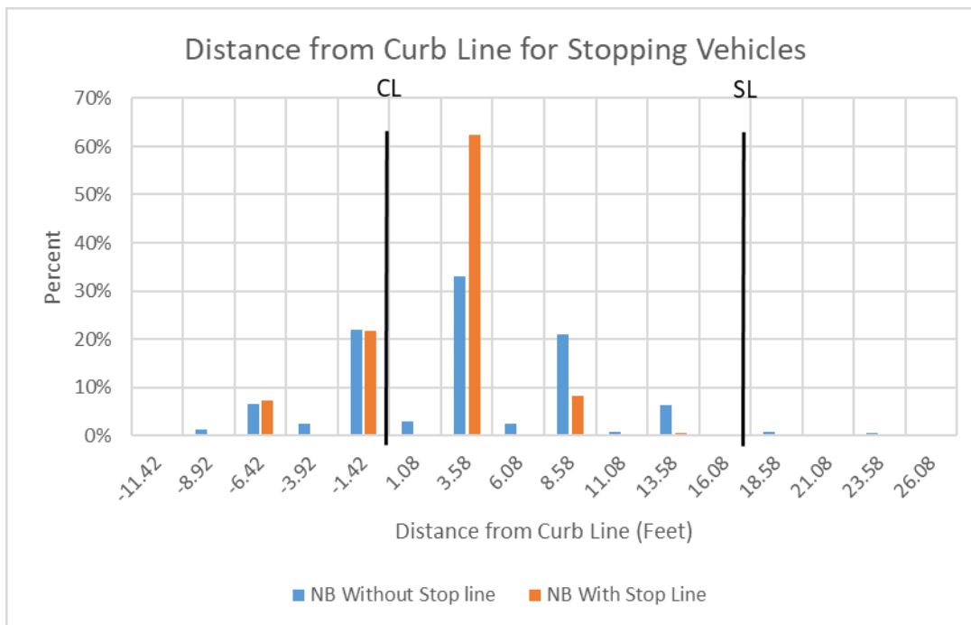
Figure 3.66 Vernon Ave S and Arcadia Ave Distribution of Stopping Distance During Stop Events
