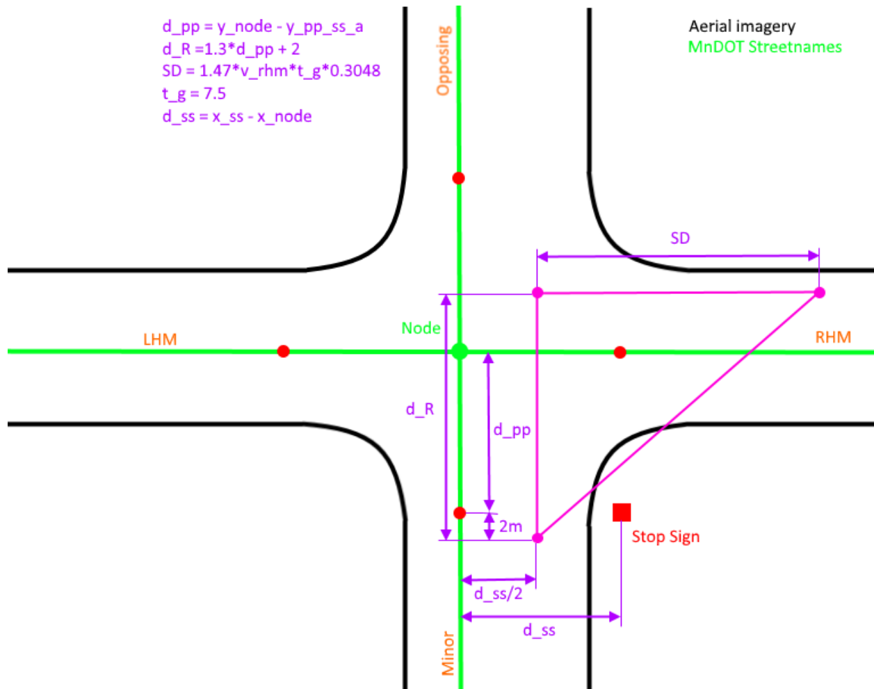
Figure B-0.2 Creation of rudimentary required sight distance triangles – Step 2
