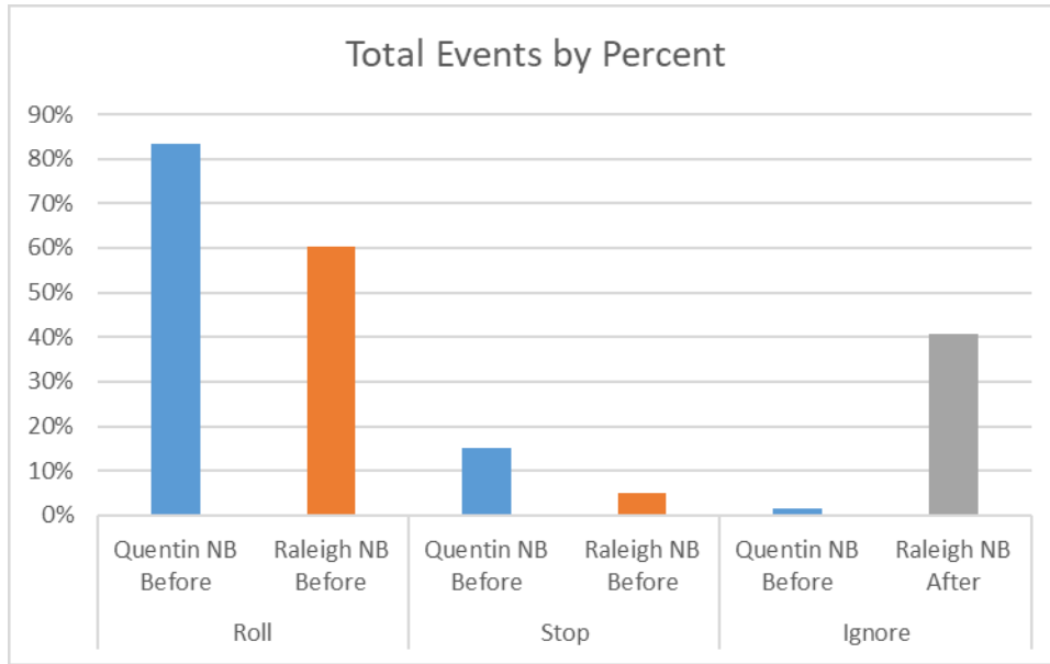
Figure C-0.19 Quentin Ave NB and Raleigh Ave NB, no stop line
