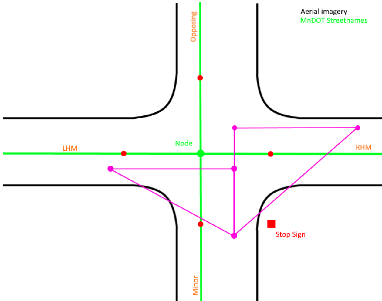
Figure B-0.4 Creation of rudimentary required sight distance triangles – Step 4
