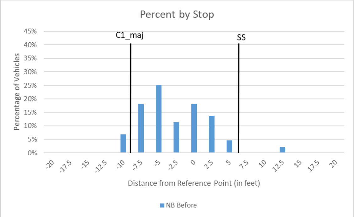
Figure C-0.8 Quentin Ave NB Distribution of Stopping Distance During Stop Events
