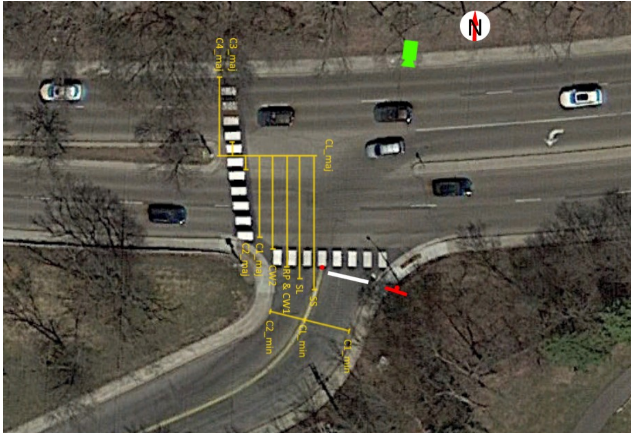
Figure 3.55 Aerial view of the intersection of 50th St W and Eden Ave with measurements marked
