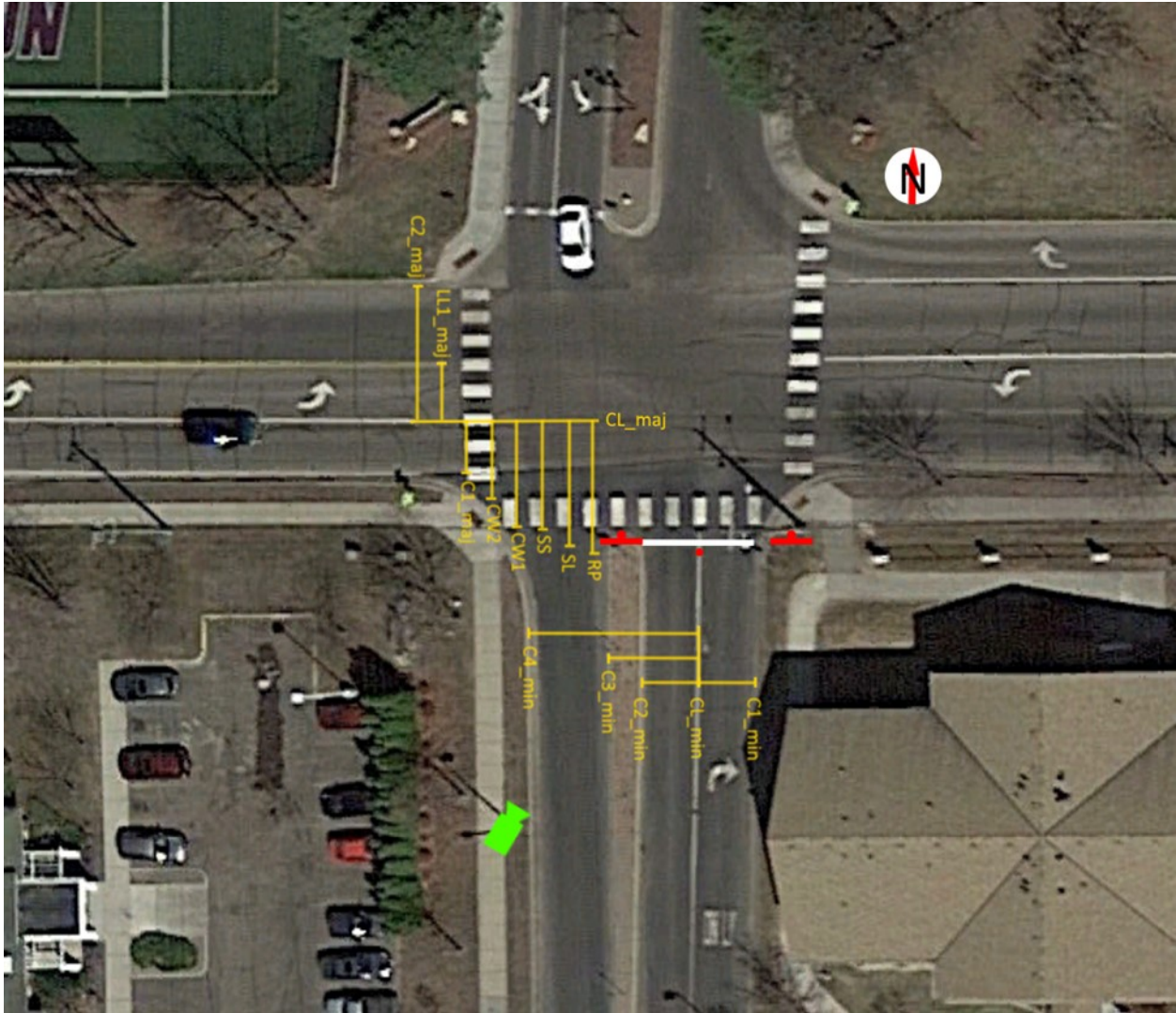
Figure 3.45 Aerial view of the intersection of Lincoln Dr and Lydia Ave W with measurements marked
