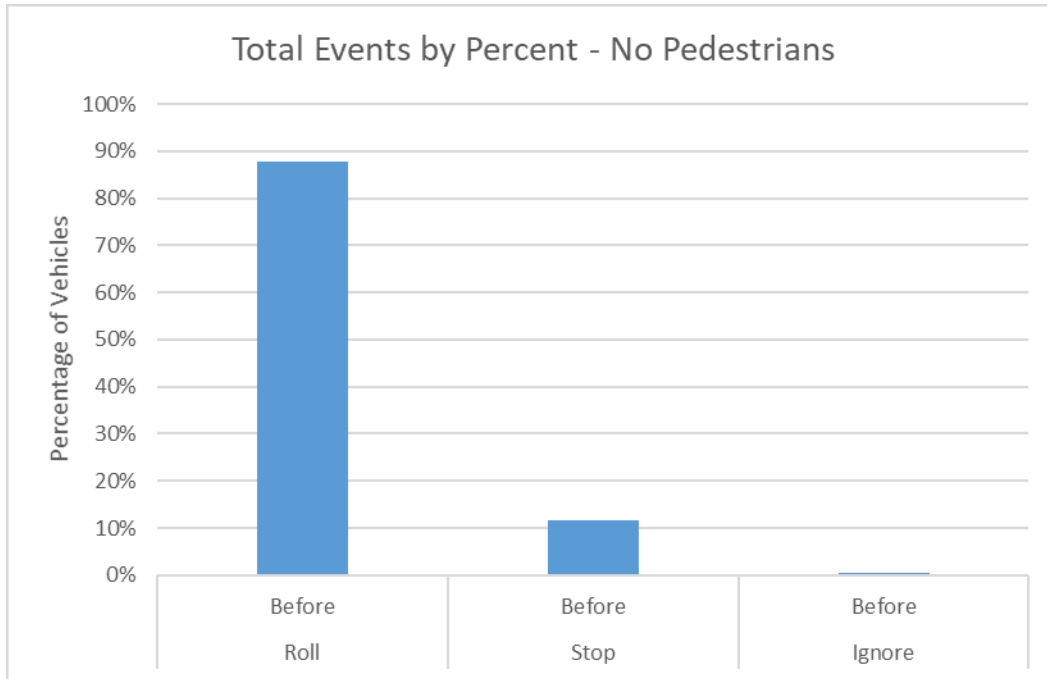
Figure C-0.15 Quentin Ave SB distribution of driver crossing behavior – No Pedestrians
