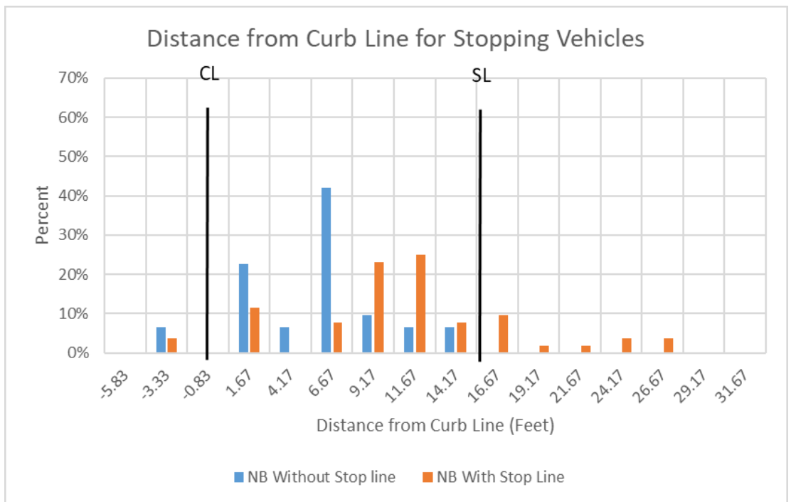
Figure 3.103 Raleigh Ave NB and W 28 th St Distribution of Stopping Distance During Stop Events
