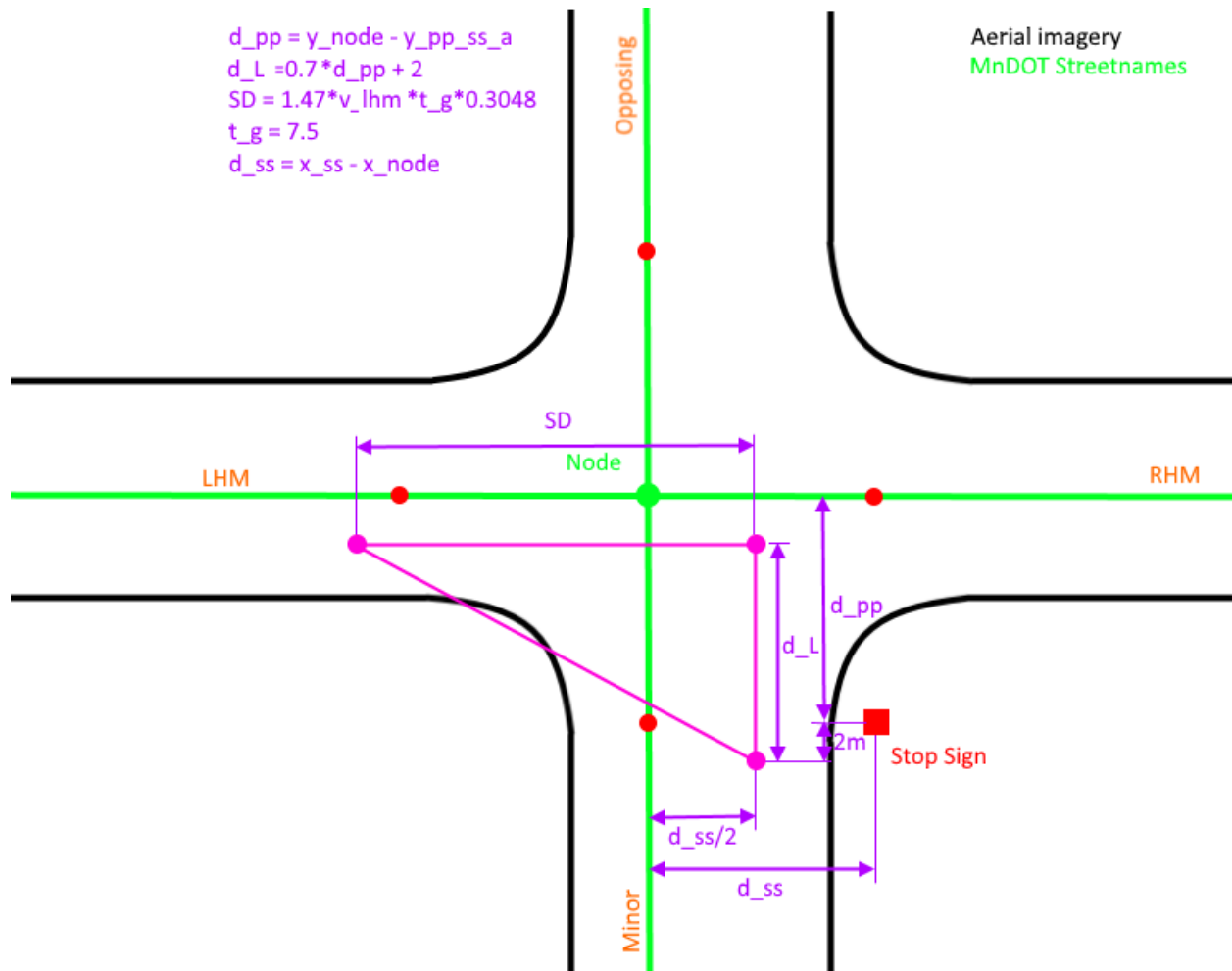
Figure B-0.3 Creation of rudimentary required sight distance triangles – Step 3
