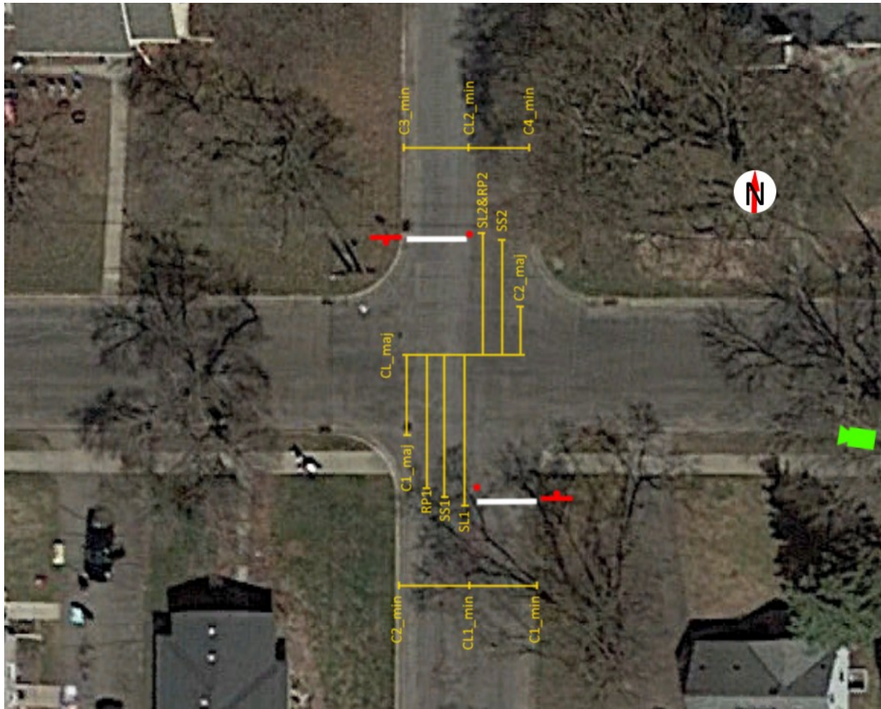
Figure 3.98 Aerial view of the intersection of Raleigh Ave and W 28 th St with measurements marked
