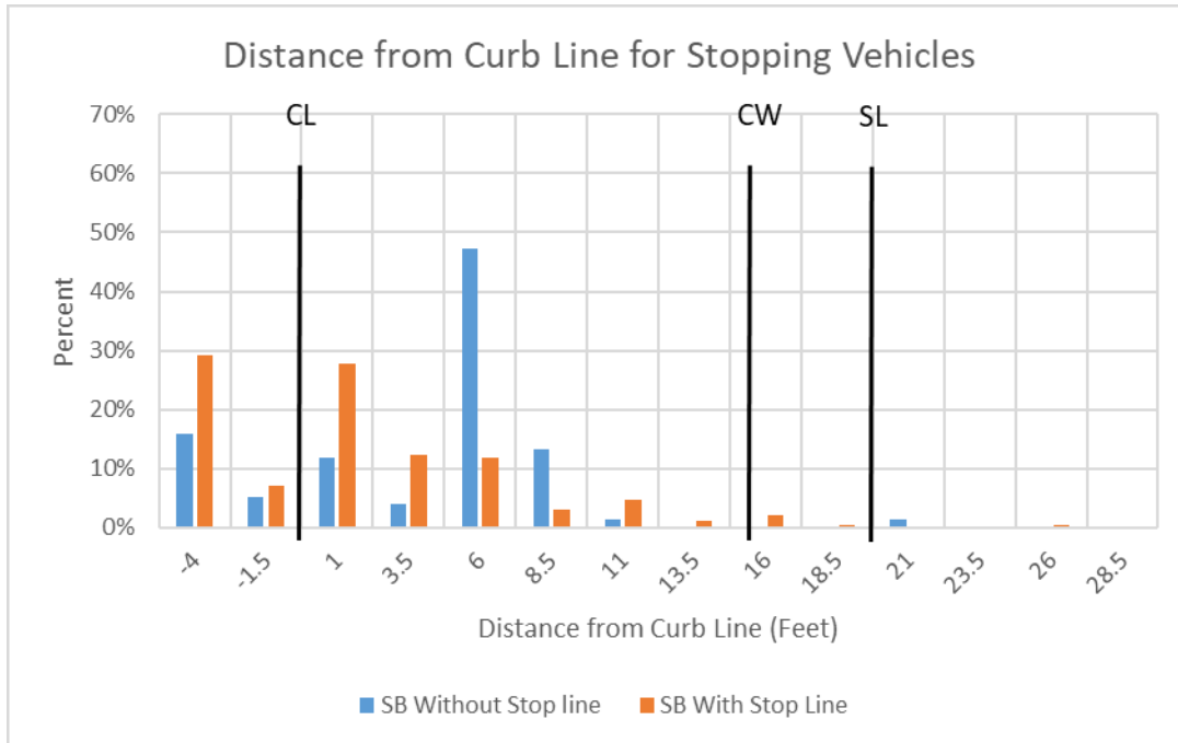
Figure 3.53 Lincoln Dr Right Lane and Lydia Ave W Distribution of Stopping Distance During Stop Events
