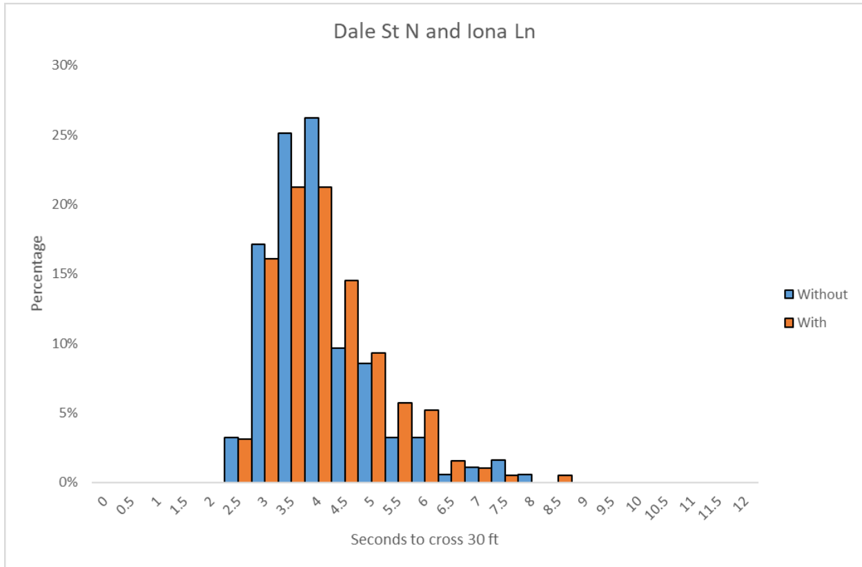
Figure 3.44 Dale St N and Iona Ln Histogram of Roll and Ignore behaviors, in seconds to travel 30 ft
