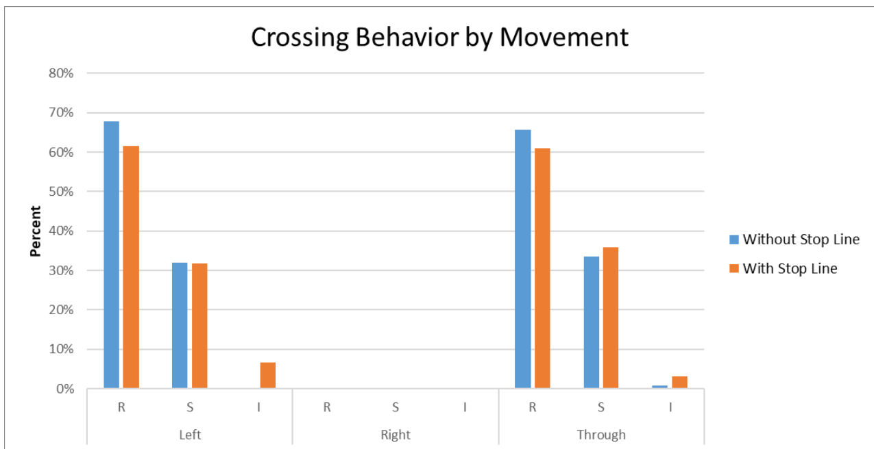
Figure 3.95 W Territorial Rd and Cromwell Ave N (through) distribution of driver crossing behavior as a percentage of all events without- vs with-stop line, by driver movement
