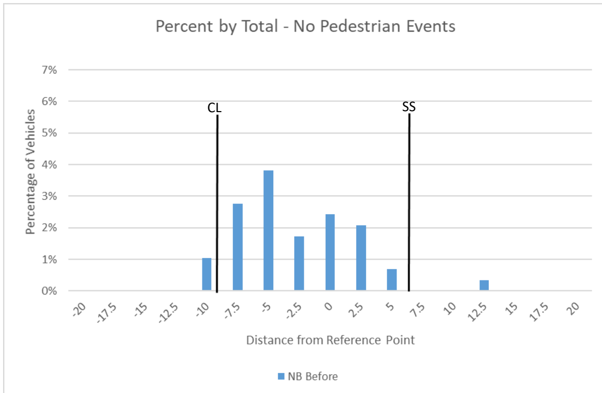
Figure C-0.9 Quentin Ave NB distribution of driver crossing behavior – No Pedestrians
