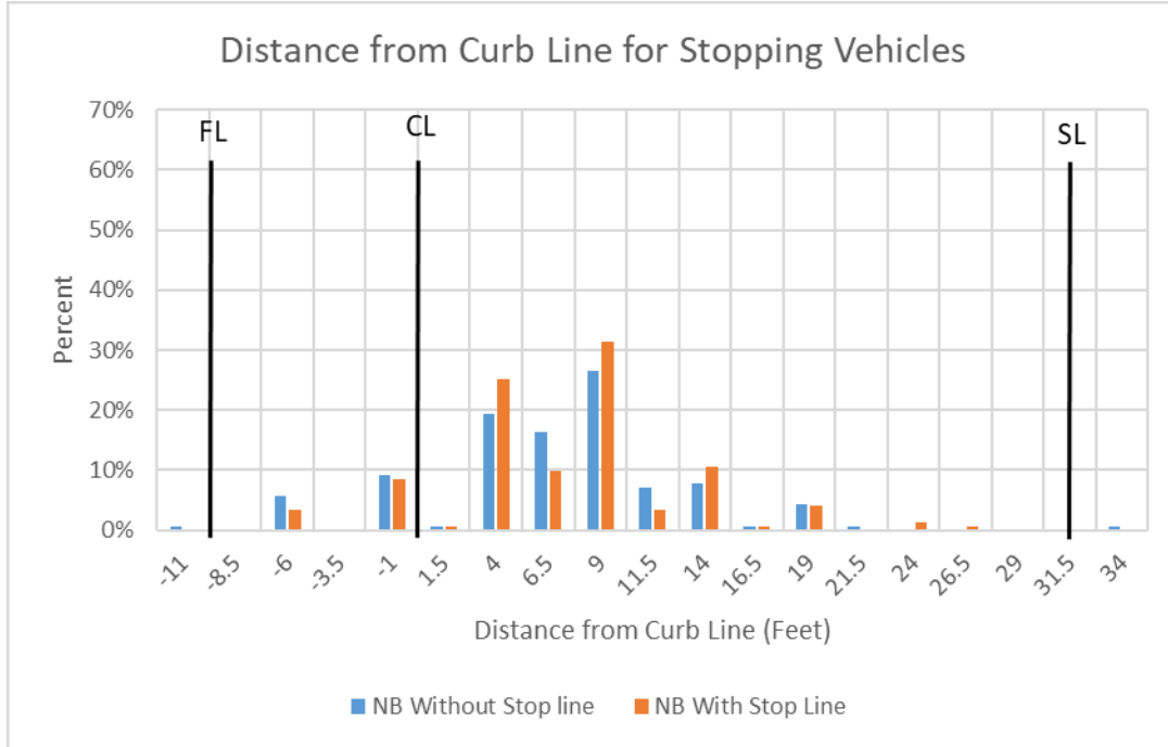
Figure 3.86 Warner Rd and Fish Hatchery Rd N Distribution of Stopping Distance during Stop Events
