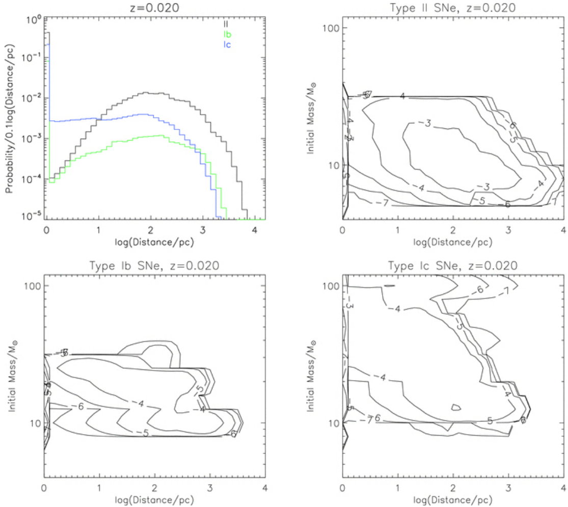
Figure 1.3: The top-left plot shows the distribution of distance traveled by SN progenitors for SNe II, Ib, and Ic with respect to the probability of traveling that distance. While we see that it is most likely that progenitors do not travel very far, there is reasonable probability for a progenitor star to travel hundreds of parsecs before explosion. The top-right and bottom two plots show the distribution of distance traveled by SN progenitors versus the progenitor's original mass. The data comes from the simulations of Eldridge et al. (2011). The contours represent the probability in \log_{10} of a SN progenitor of that initial mass traveling that distance. This figure is from Eldridge et al. (2011).
