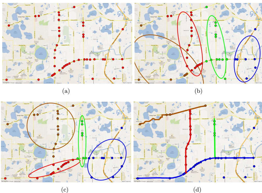
Figure 14: An example of network footprint to summarize high activity patterns. (a) A spatial network with activities. (b) Polygon footprint to summarize activities with Euclidian distance (by CrimeStat) [107] (c) Polygon footprint to summarize activities with network distance (by CrimeStat). (d) Network footprint to summarize activities.
