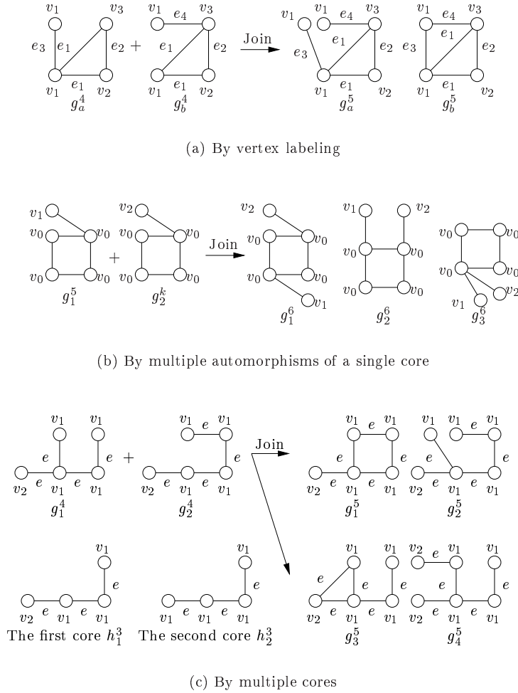
Figure 2: Three different cases of candidate joining
