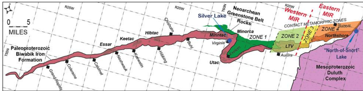
Figure 1. Simplified geologic map of the BIF and contact metamorphic zones adjacent to the Duluth Complex (after French, 1968; Jirsa et al., 2005; McSwiggen and Morey, 2008).
