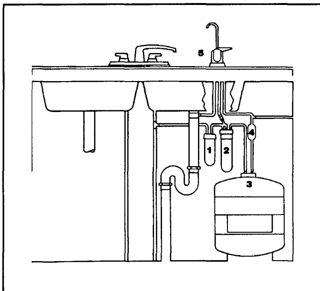
Figure 2. A Typical Home RO System Includes: (1) particle filter, (2) reverse osmosis membrane unit, (3) pressurized treated-water storage container, (4) carbon adsorption post-filter, and (5) separate treated-water tap.
