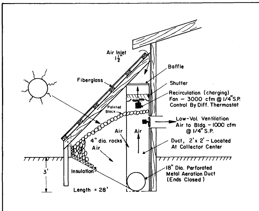
Figure 6. Lean-to solar collector with rock heat storage.
