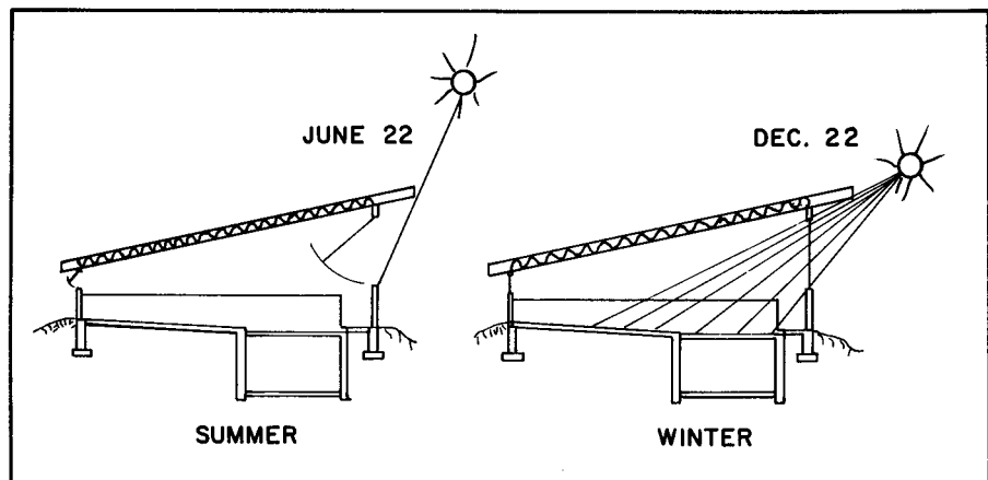
Figure 2. Passive solar system—use roof overhang to block out the sun during summer.
