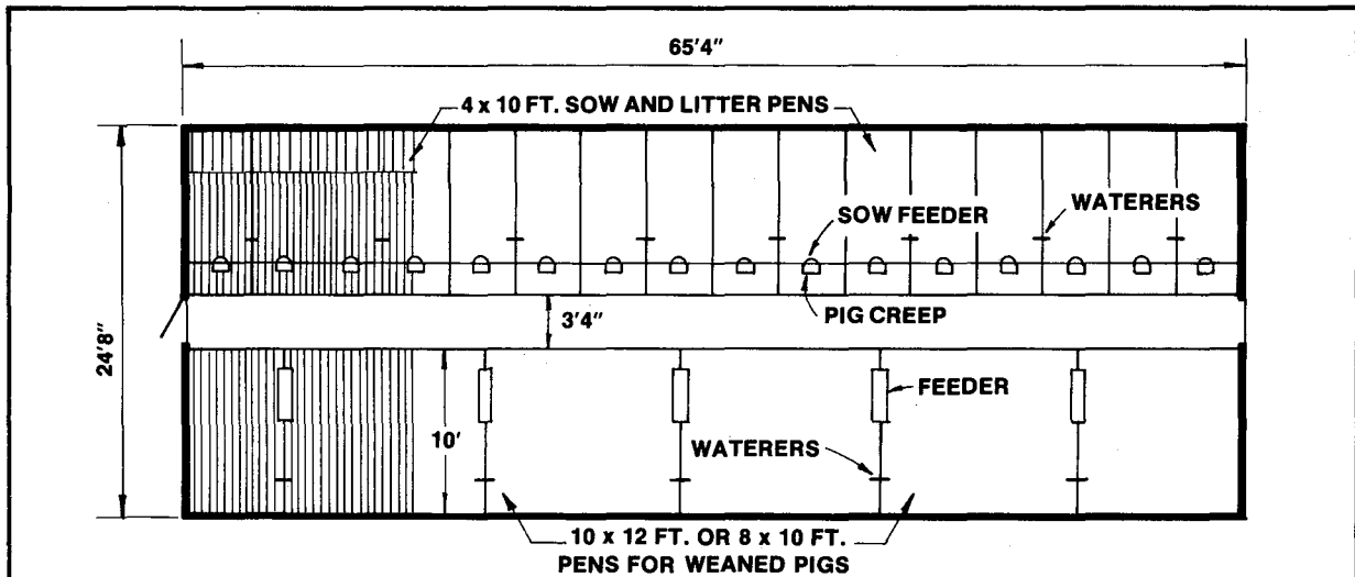
Figure 1. Total slotted floor nursery — 4 x 10 ft. pen for sow and litter, 8 x 10 ft. loft pens, or 10 x 12 ft. pens for 20 and 30 weaned pigs, respectively.
