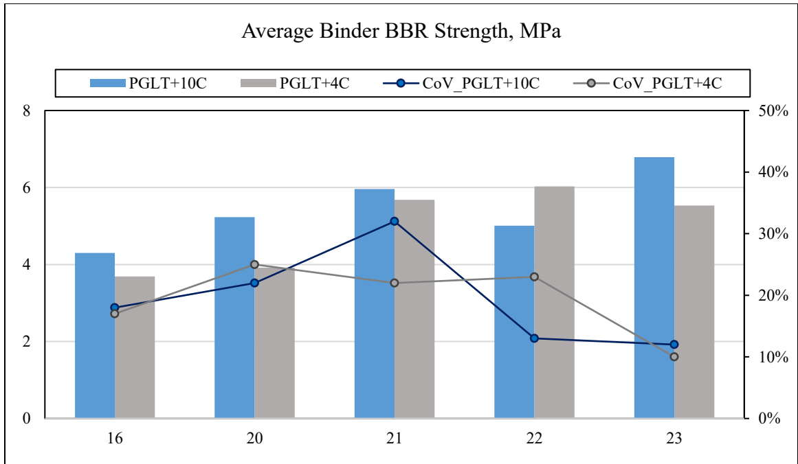
Figure 4.8: BBR Strength of Binders from Cell 16, 20-23.
