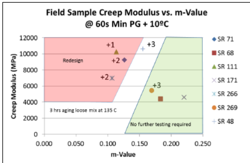
Figure 5.12: Example of diagram used for a design temperature of -22°C.
