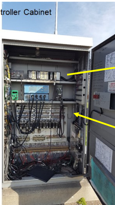
Figure 2.6 Controller Cabinet and Loop Detector Cards at TH169 & TH282 Intersection.
