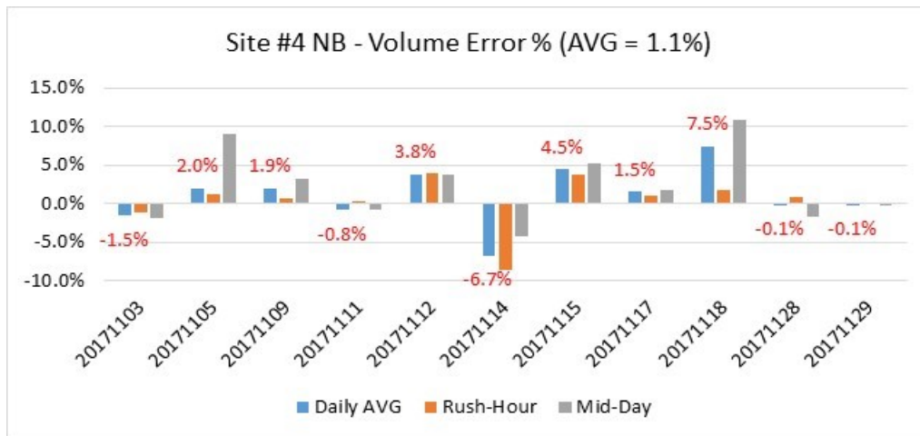
Figure 4.27 Traffic Volume Error Percentage at Site #4 NB.
