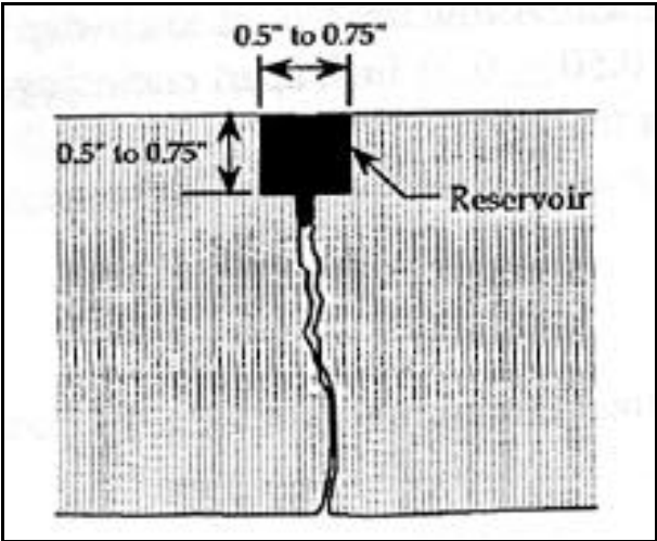
Figure 4-1. Reservoir Dimensions
