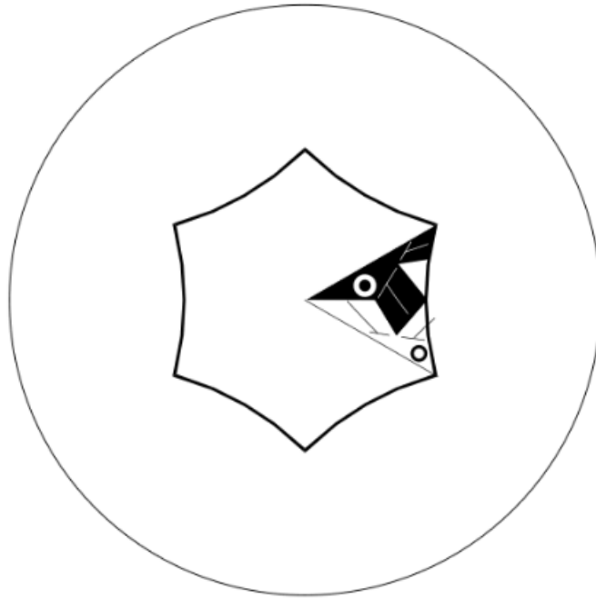
Figure 4.3: Pattern with central p-gon before replicating the motif
