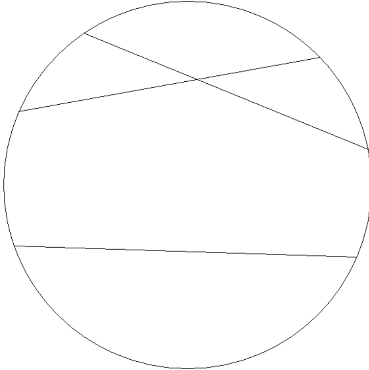
Figure 3.1: Beltrami Klein Model
