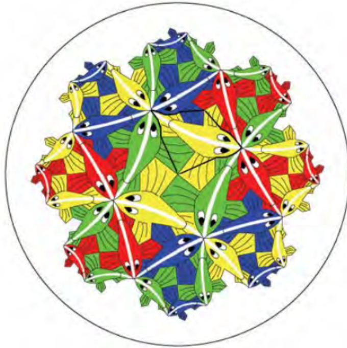
Figure 4.2: A sample motif outlined in black
