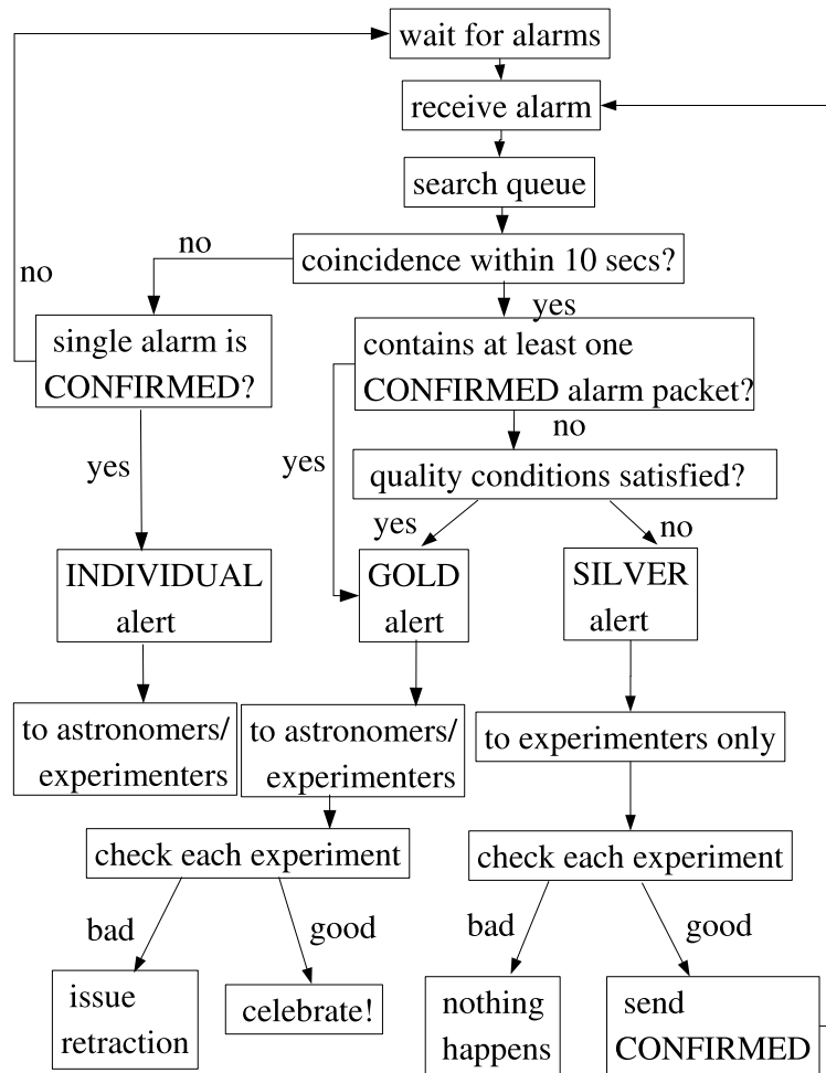
FIG. 4.4. SNEWS alert flowchart [29]. This algorithm runs on the SNEWS coincidence server at Brookhaven National Laboratory, and discriminates against alarms to determine their candidacy as a supernova event.
