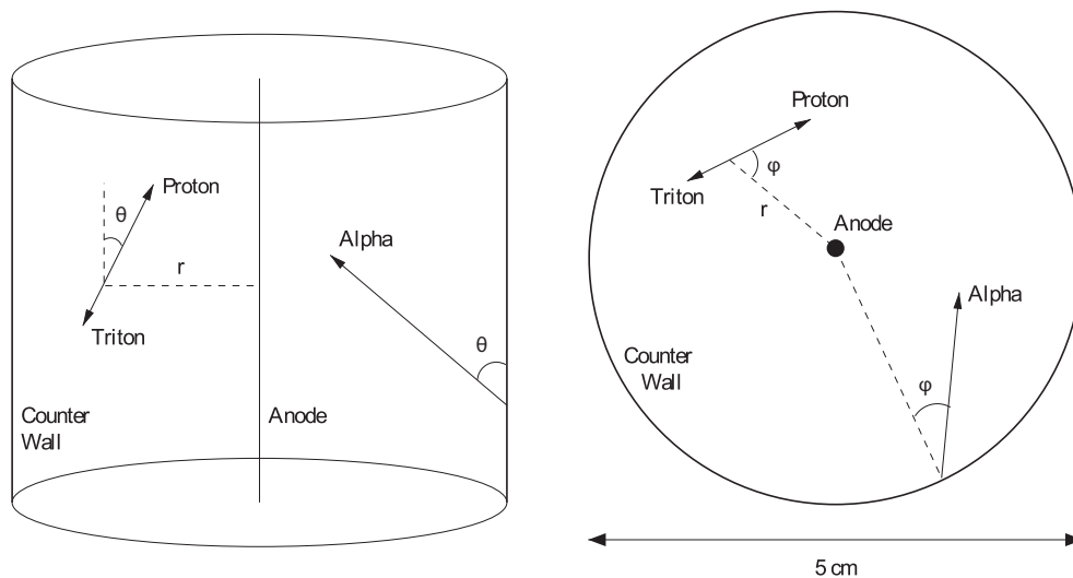
FIG. 5.4. ^3\text{He} Neutron capture schematic [38]. The proton-triton pair are produced and move in opposite directions. The proton and triton peaks may be separated in time by an amount determined by their orientation in the counter.
