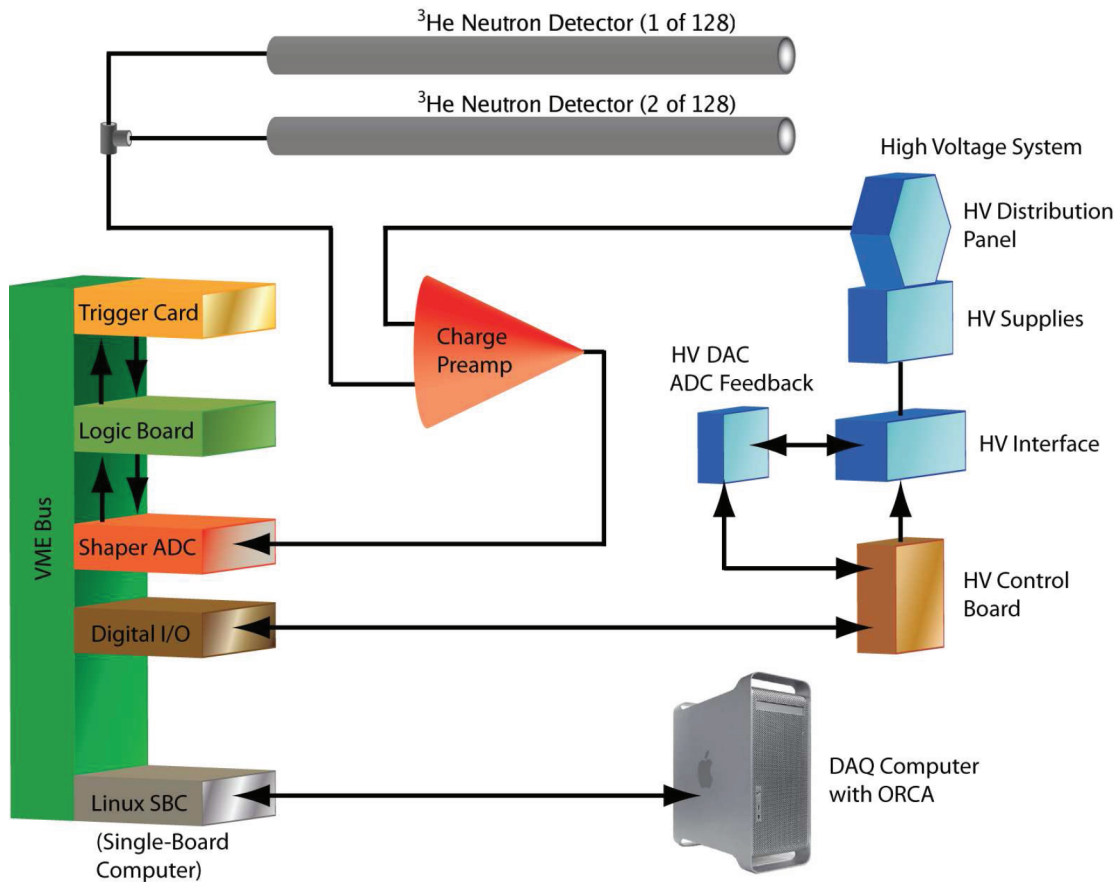
FIG. 5.6. HALO electronics diagram. The ^3\text{He} detectors are joined in pairs and connected to 64 preamps where the charge collected at the ^3\text{He} counter anode is converted into a high voltage (HV). The signal is sent to shaper ADC boards which digitize and integrate the current. The digitized signal is then sent to a Linux single board computer (SBC) and is passed to the ORCA software that runs on the DAQ computer. The HV system is controlled by the ORCA software. A HV ADC is used as a feedback mechanism to monitor the voltages in nearly-real-time. A pulse distribution (not shown) has been implemented to allow the injection of simulated pulse signals into the preamps as a way to test their response.
