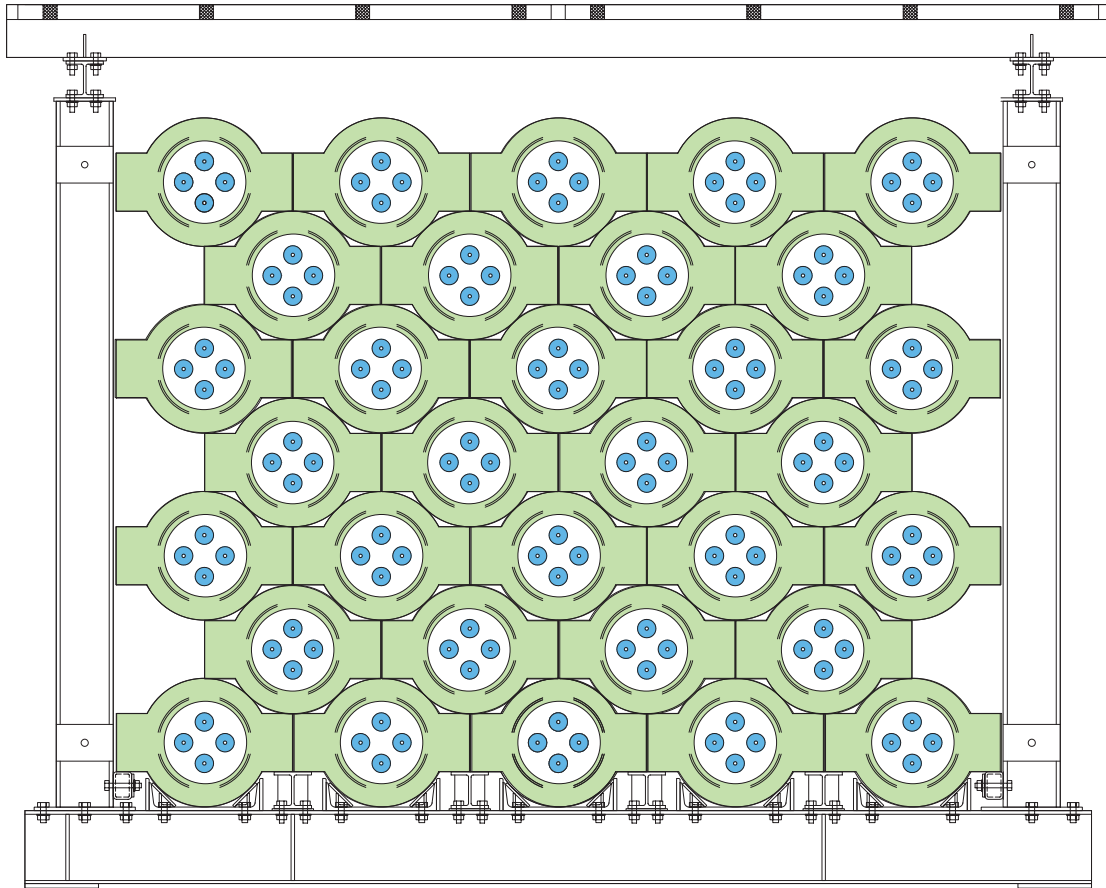
FIG. 5.1. Schematic of the HALO detector design (Front View). The lead blocks (stacked objects, shaded green) are the site of neutrino interactions. The products of those interactions, neutrons, travel into the ^3\text{He} proportional counters (four circles contained within each lead block, shaded blue) and are captured on ^3\text{He} . The structure is 2.4 m tall.
