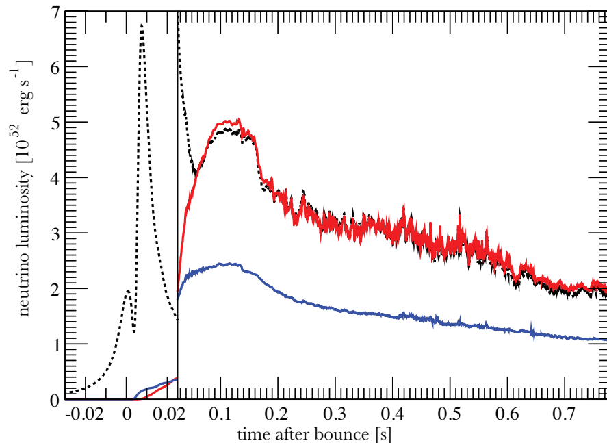
FIG. 3.2. Simulated supernova neutrino signal. The simulation of this 15M_{\odot} star was general relativistic and 2 dimensional. The black lines are for \nu_e , the red lines for \bar{\nu}_e , and the blue lines for heavier neutrinos \nu_x [19]. The neutrino flux persists for several tens of seconds and then fades.
