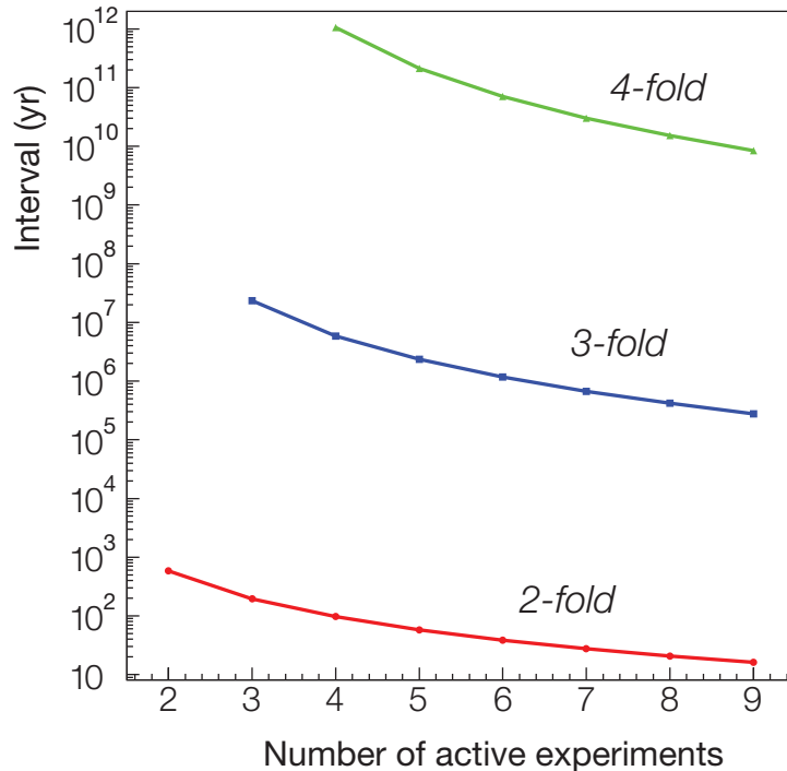
FIG. 4.3. SNEWS rate of accidental alerts. The average interval between false-alarms is modeled to first order as a Poisson process parameterized by the number of required coincidences in a 10 second window and the number of active experiments[30].
