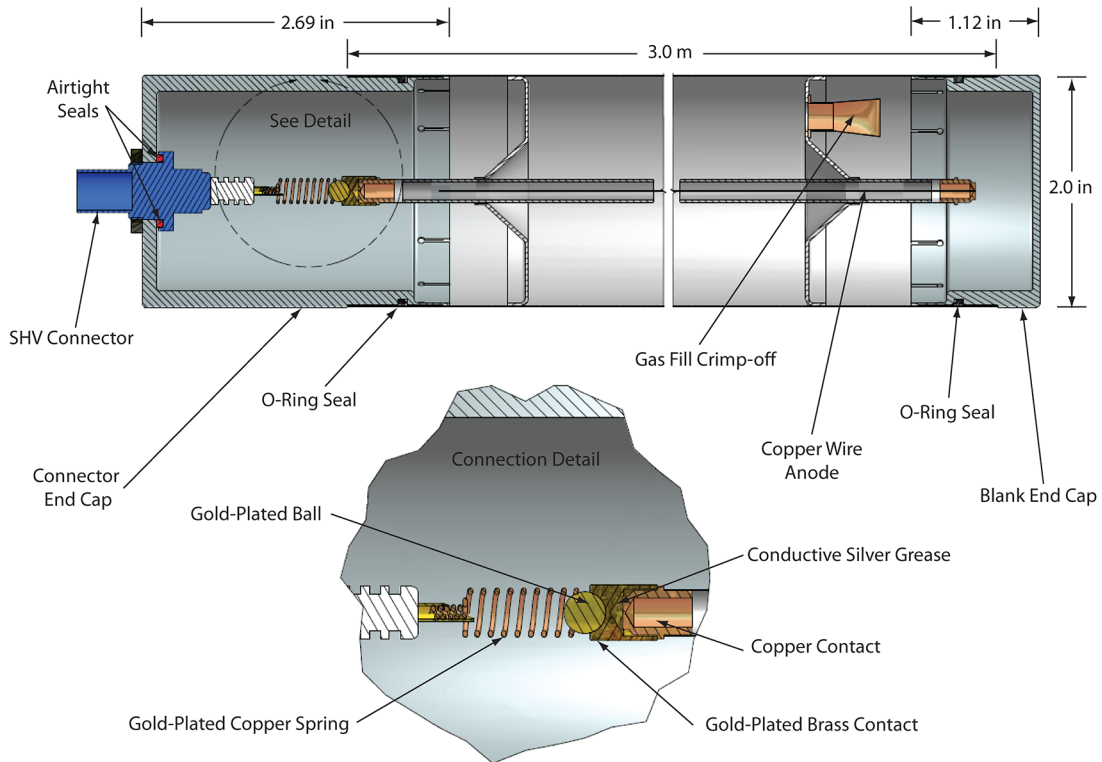
FIG. 5.3. Technical diagram of ^3\text{He} proportional counter [37]. The counters were originally used in Phase III of the SNO experiment, but have been refitted with new endcaps for use in HALO.
