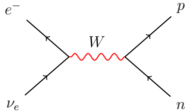
FIG. 2.1. Charged current interaction. A W boson is exchanged between the neutron and neutrino to produce an electron and proton.
