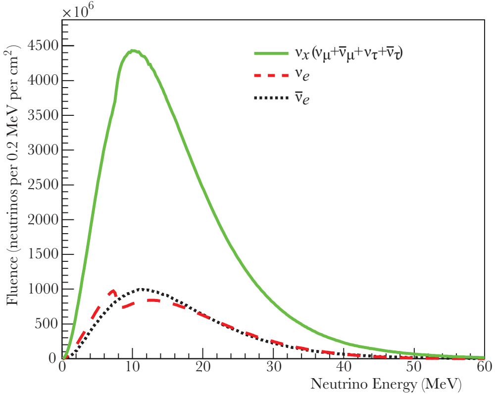
FIG. 3.3. Simulated supernova neutrino fluence [22]. The neutrino flux generated by the GVKM model[24] for a supernova 10 kpc from Earth was integrated over a period of 10 s to produce this fluence. The energy distribution for all neutrino flavors are centered around \gtrsim 10 MeV. The model accounts for neutrino-neutrino interactions and dynamic MSW effects, which cause the wobble seen in the \nu_e profile.
