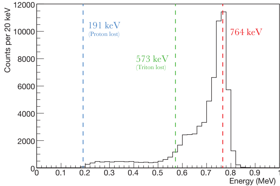
FIG. 5.5. {}^3\text{He} neutron-capture spectrum from {}^{24}\text{Na} calibration[38]. The neutron peak is clearly located at 764 keV, but there also exist shoulders that terminate at 573 keV and 191 keV due to some of the triton’s or proton’s energy (respectively) being lost due to collisions with the walls of the counter.
