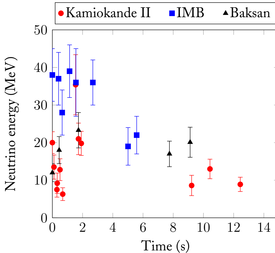
FIG. 4.1. Observed neutrino spectrum from SN 1987a. Twenty six events were recorded by three separate experiments during a 13-second period. A scintillator detector in Mont Blanc in Italy detected a neutrino signal, but it was not coincident with the other detectors and are not thought to be associated with the supernova[28].
