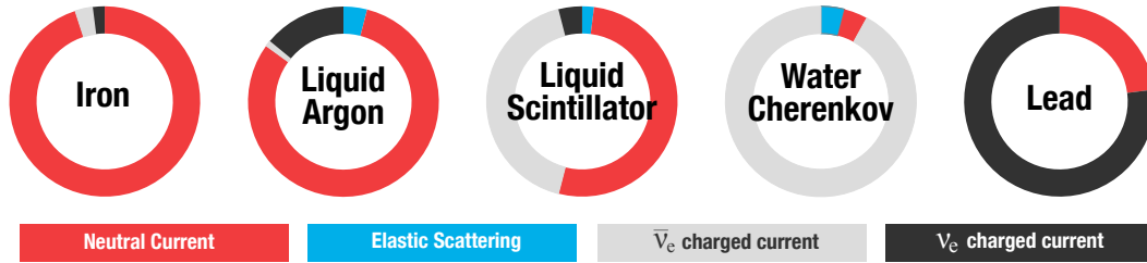
FIG. 5.2. Neutrino detector sensitivities. Different neutrino interaction materials have different neutrino flavor sensitivities. This figure shows which interaction channels appear as a proportion of the total neutrino signal for popular interaction media. Since HALO is the first experiment to lead as an interaction medium, it will offer unique insight into the \nu_e charged current channel.
