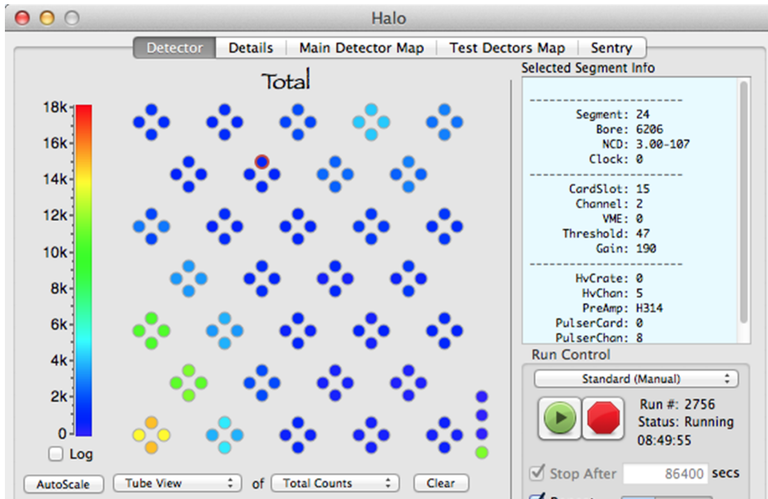
FIG. 6.4. DetectorView improvements The DetectorView looks like the physical HALO detector. The colors represent the total counts on each ^3\text{He} tube during the run. This can be used as a quick inspection of relative detector response. You can see the tubes in the lower left of HALO have relatively high rates (there was a neutron source in that area). Each ^3\text{He} can now be selected to reveal its hardware map information (on the right).
