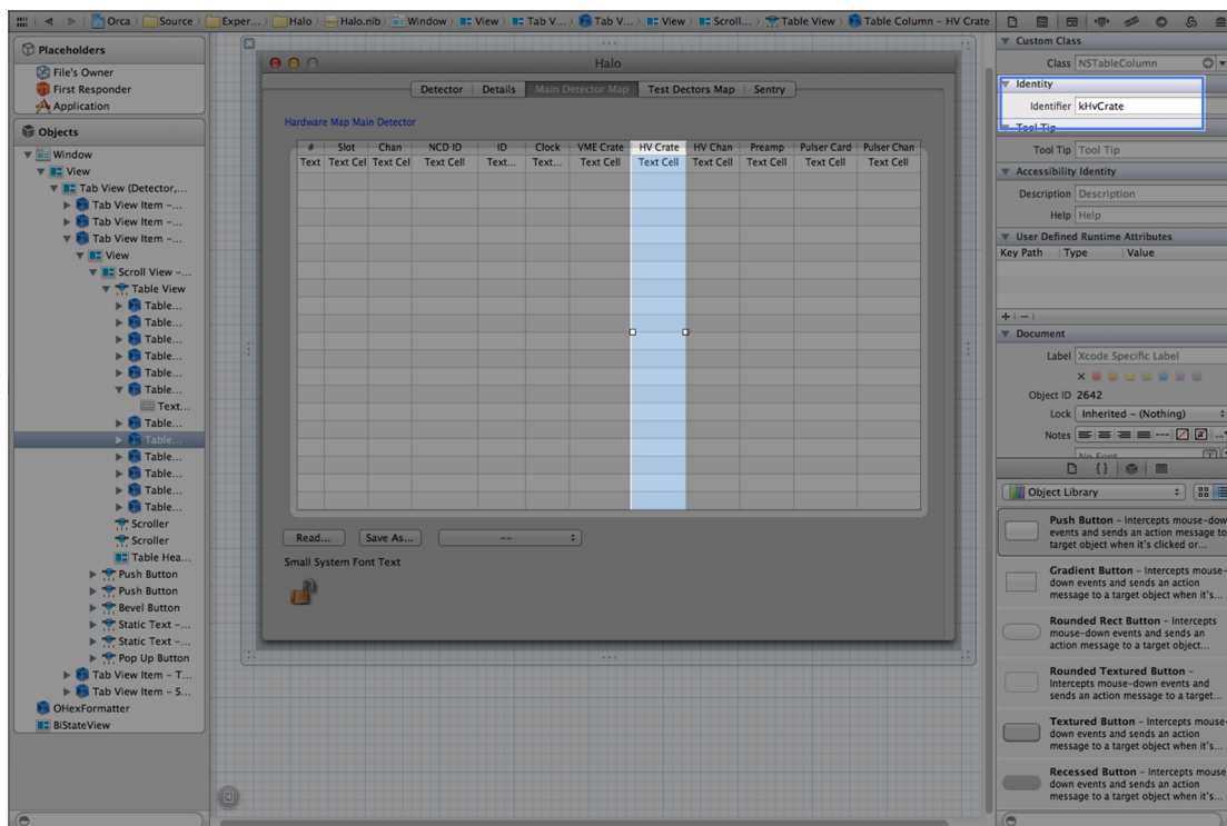
FIG. 6.2. Building the hardware map. This screenshot of Xcode shows the graphical Interface Builder that is used to design user interfaces. Halo.nib is the file being edited here. In the center of the interface is the table that will be populated with the details of the hardware map. When a CSV file containing the map is read, each column is assigned a unique identifier, which must also be assigned to a column in the table (on the right).
