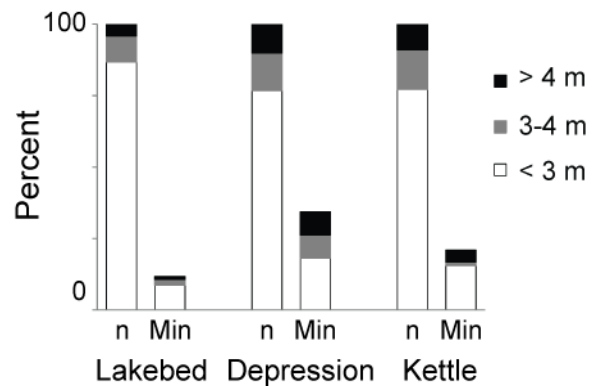
Figure 11. Peat thickness in different geomorphic classes. Bars labeled n refer to the percentage of measurements in each thickness category, shown by the legend. Bars labeled Min refer to the percentage of the measurements in each category that were minimum thickness estimates.
