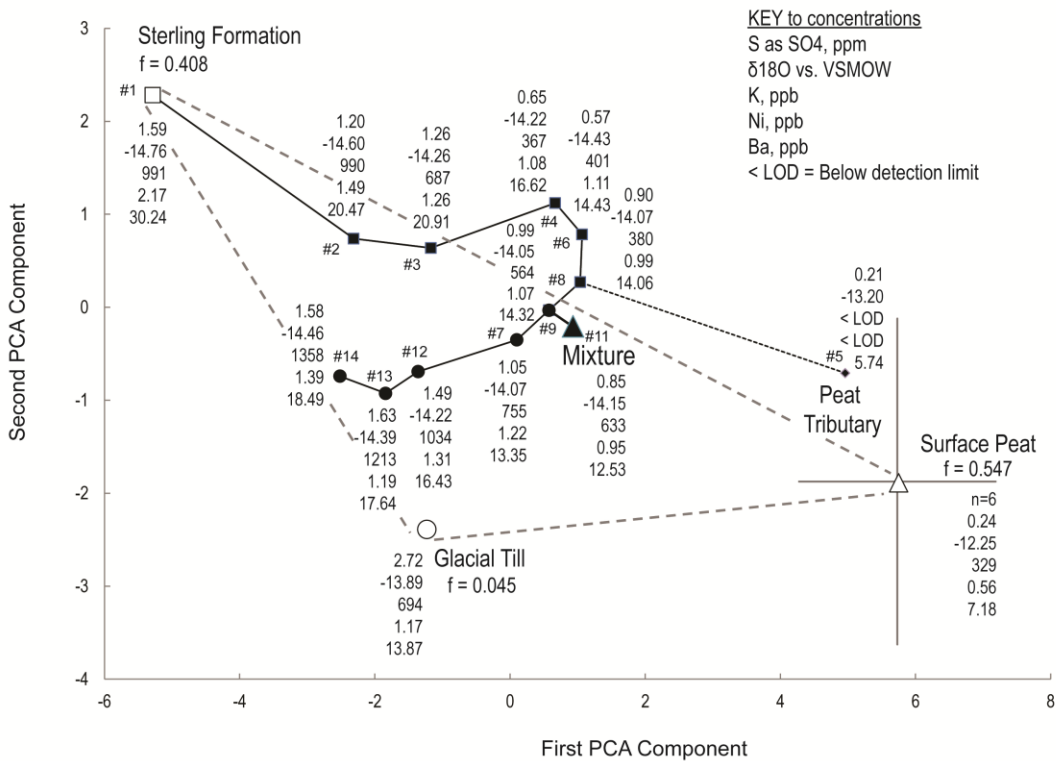
Figure 27. End-member mixing diagram at a single point-in-time during the summer dry-period along the two tributaries of Limpopo Creek. A mixing space (approximated by the dashed lines) is defined by three end-members (hollow squares) enclosing stream samples (solid squares), which are connected in downstream order. Concentrations of the tracers at each point are given in the order shown in the key. The point labeled “peat tributary” represents a sample taken from a small tributary flowing into the creek from a peatland just above the confluence of the two tributaries. The peat surface end-member is depicted with one standard deviation in its projected values (large cross). The f-value listed under each end-member is the fractional proportion that the end-member contributed to the mixture, the sample taken at the mouth of the stream (solid triangle).
