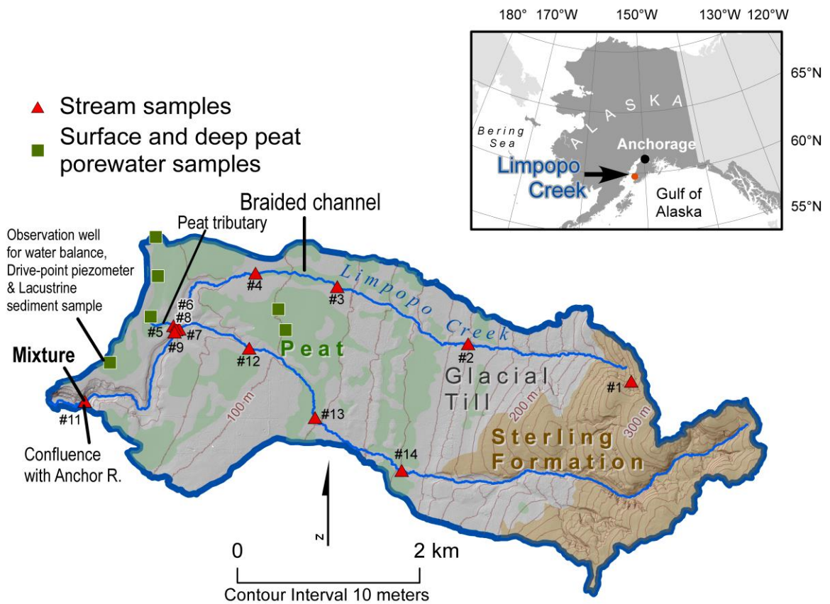
Figure 22. The Limpopo Creek Watershed in Southcentral Alaska. The steeper eastern third of the watershed is underlain by the Sterling Formation (tan), whereas the western two-thirds is composed of glacial till (gray) and lacustrine deposits overlain by peatlands (green). Sample locations are numbered and marked by triangles for stream samples and squares for EMMA end-members. The northern tributary of Limpopo Creek flows as a braided channel where indicated.
