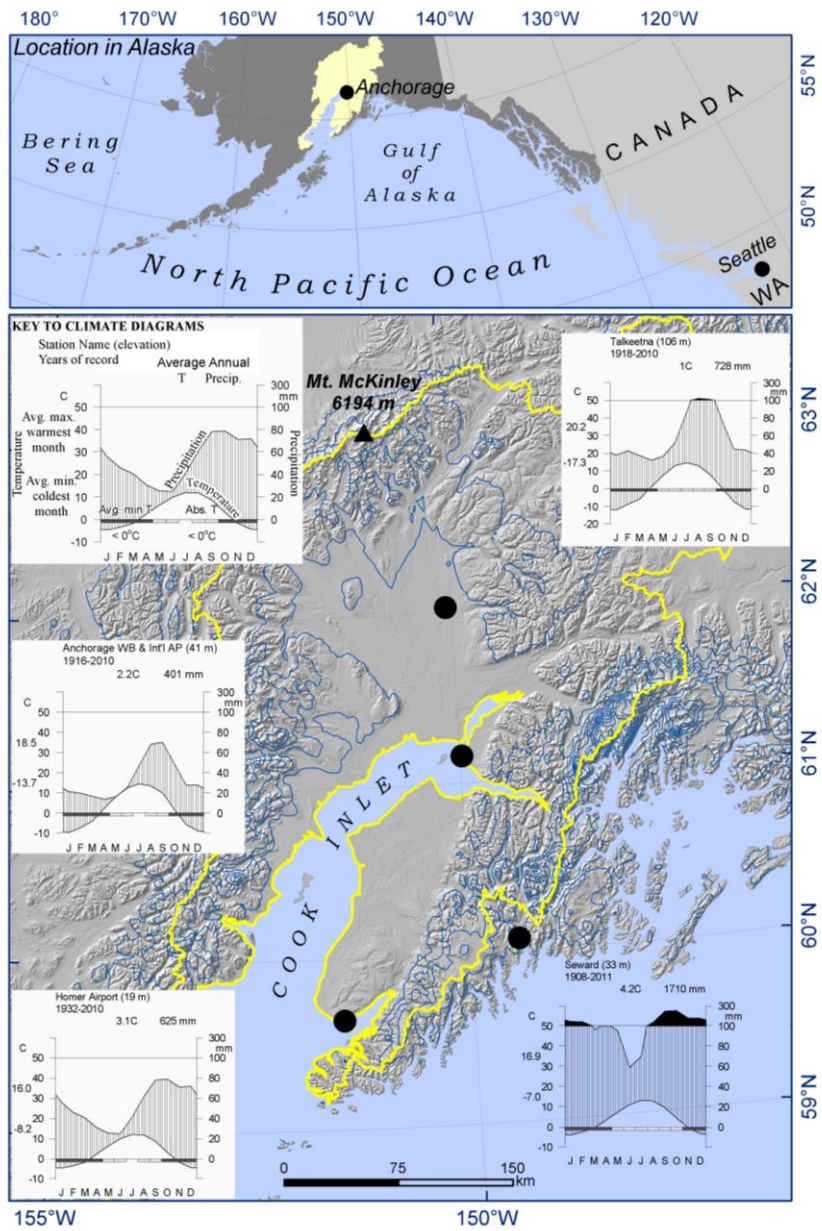
Figure 18. Location, physiography, and climate of Cook Inlet Basin, Alaska, shown by yellow polygon (top) and outlined in yellow (bottom). Blue lines show 1000 mm isohyets (bottom). Black circles on bottom map show locations of climate stations. Climate diagrams follow Walter & Leith (1960).
