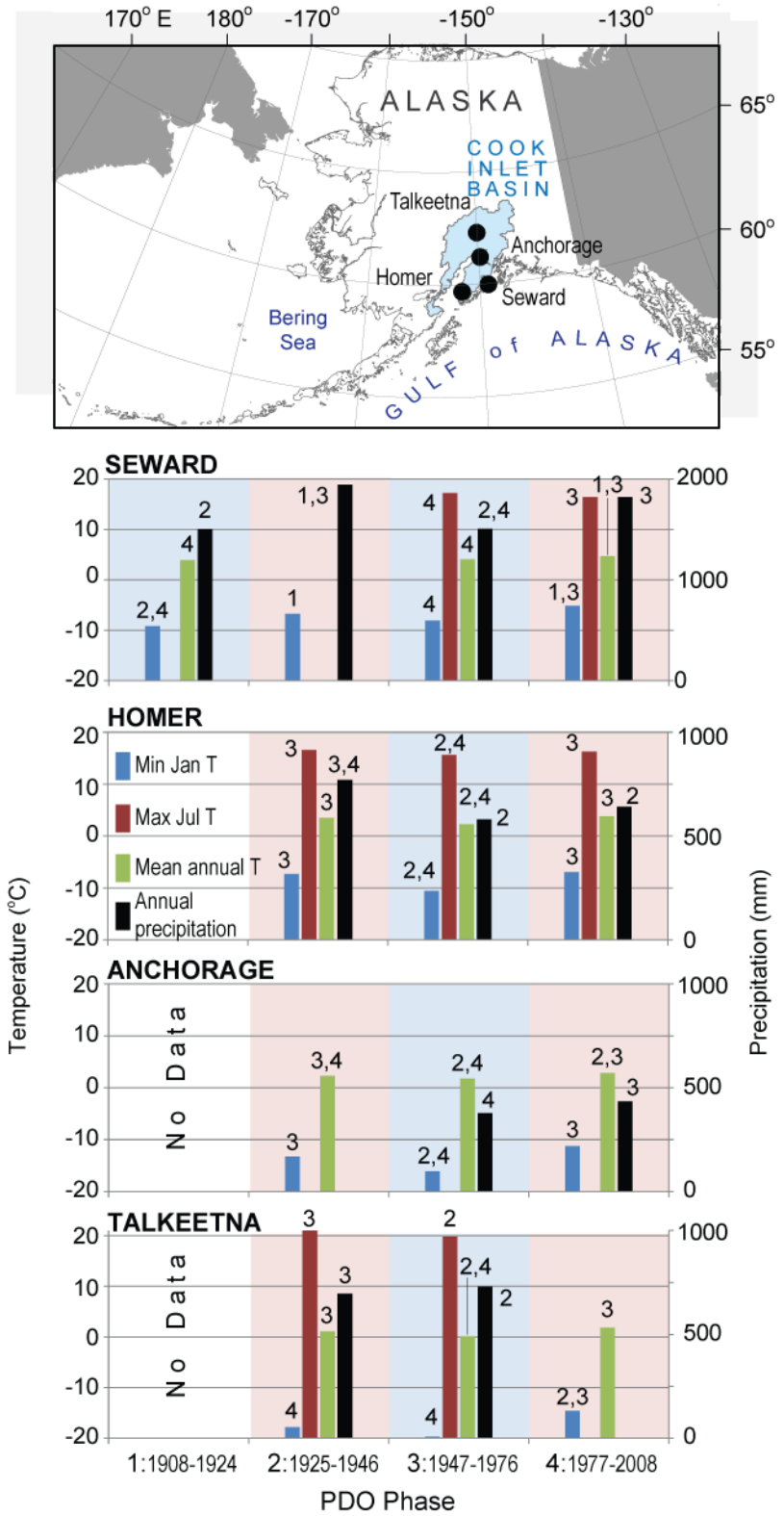
Figure 1. The effect of PDO phases on climate at four stations in CIB. The stations are shown on the map of Alaska (top). Cool phases are shown with a blue background, warm phases with pink, and years of each numbered phase are shown along the x-axis. Temperatures are shown along the left-hand axis, and precipitation on the right. Bars show: average daily minimum temperature for January (blue); average daily maximum temperature for July (red); average annual temperature (green); and annual precipitation (black). Numbers above bars indicate significant differences among PDO phases using the Mann-Whitney U-test with \alpha < 0.05 corrected for multiple comparisons using the Holm-Bonferroni method. Only the bars with significant differences are shown.
