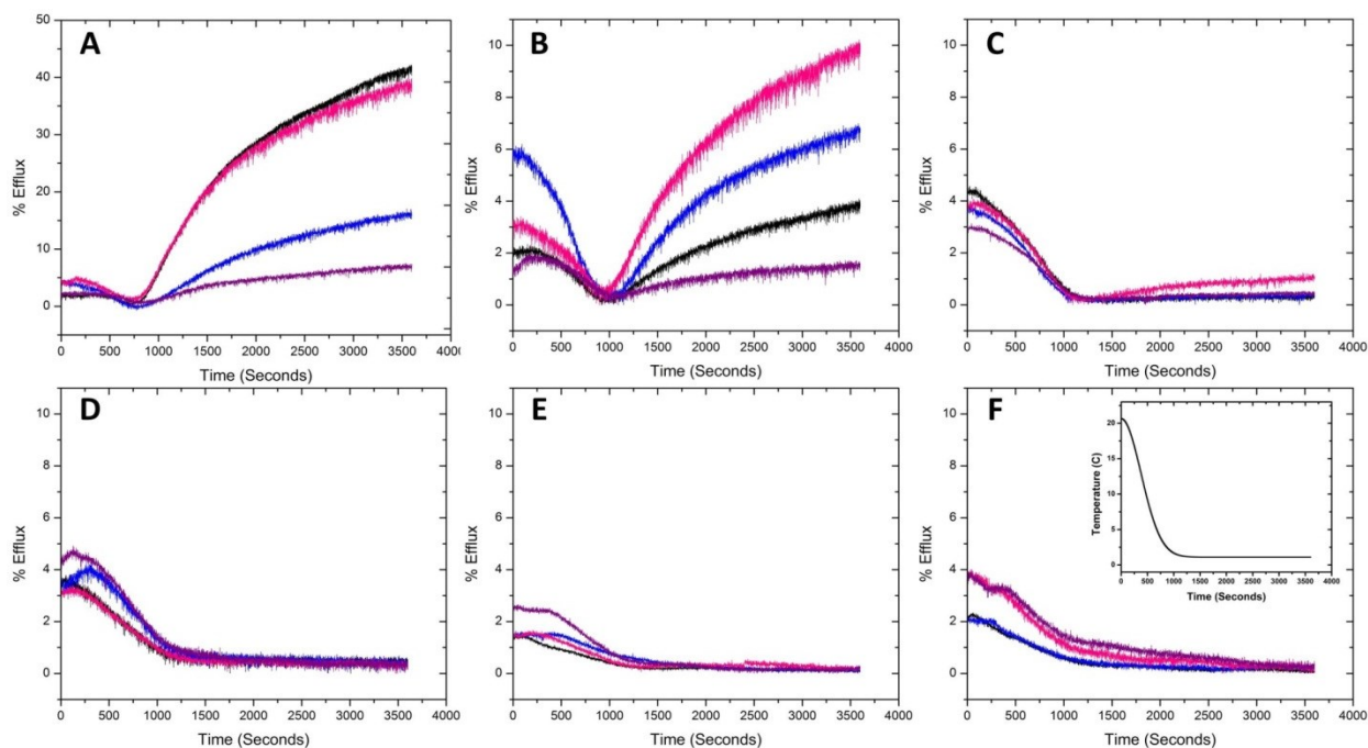
Figure 2. The efflux of carboxyfluorescein (CF) from Large Unilamellar Vesicles composed of POPC:POPS (60:40) and varying cholesterol. All samples contained 333 \mu\text{M} lipid and all plots are an average of three trials. Black: lipid alone; blue: lipid and \text{Ca}^{2+} ; pink: lipid and Annexin a5; purple: lipid, Annexin a5, and \text{Ca}^{2+} . (A) POPC:POPS (60:40), no cholesterol in the vesicles; (B) POPC:POPS (60:40), with 5% cholesterol; (C) POPC:POPS (60:40), with 10% cholesterol; (D) POPC:POPS (60:40), with 20% cholesterol; (E) POPC:POPS (60:40), with 30% cholesterol; (F) POPC:POPS (60:40), with 40% cholesterol. The inset in (F) shows the decrease in temperature for all scans over 60 minutes with the water bath set to decrease from 20°C to -3°C. 3
