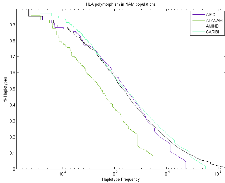
Supplementary Figures 2A-E. Comparison of HLA haplotype frequency distributions of detailed race populations within each broad race category (A - AFA, B - API, C - CAU, D - HIS, E - NAM).
