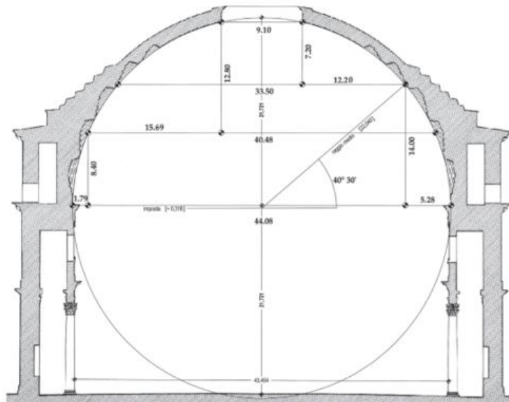
4. Hadrian, Pantheon, Rome, 126BC (Harrison, Alec 4 )
