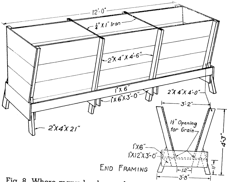
Fig. 8. Where many lambs are being fed, self-feeding may be desirable, using ground hay and grain as the ration. An adjustable feeder permitting feeding down of the feed is necessary. This feeder is cheap and easy to construct. With hand feeding, 12 inches of space is needed for each lamb; with self-feeding, 12 inches for three lambs. Self-feeders need attention several times a day to keep the feed poked down so that it is always available.
