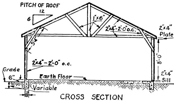
Fig. 1. This one-story type of sheep barn is most satisfactory. It is not expensive, is convenient, and provides suitable shelter. Pole-type construction may also be used.
