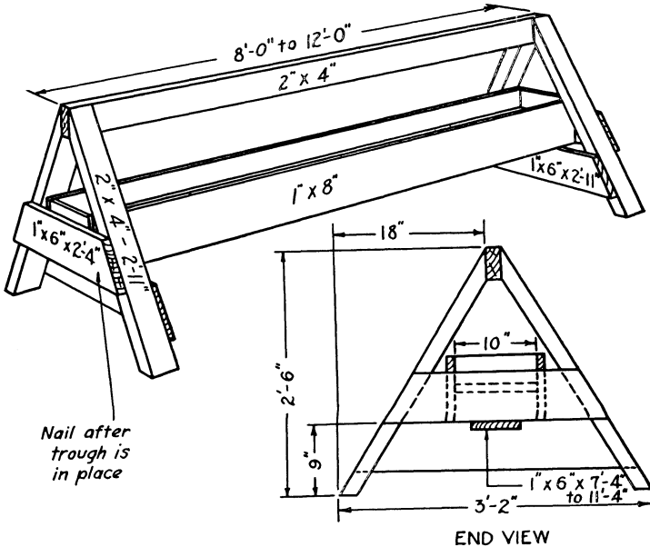
Fig. 3. A movable type of reversible feeding trough. Feeding troughs may be of any length, depending on the individual needs.
