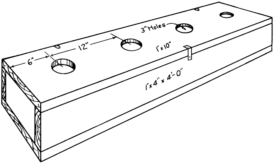
Fig. 19. Prevention is the only control for grub in the head. Pine tar on the noses repels the fly causing the infestation. A salt box with pine tar smeared around the hole that sheep reach through for salt applies the tar where needed. Pads of gunny bagging around these holes hold the pine tar. This salt box is 3 or 4 inches deep and has openings 3 inches across.
