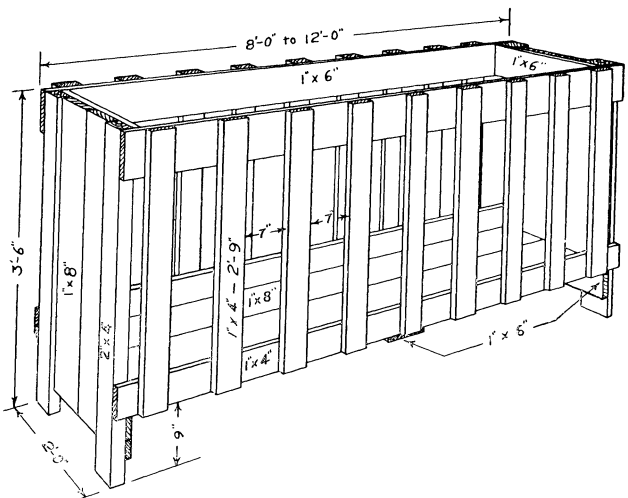
Fig. 9. Combination hay and grain racks are convenient equipment for small flocks. This straight-sided rack will keep fleeces fairly free from chaff, except for the head and neck wool. Chaffy necks can easily be separated at shearing time.
