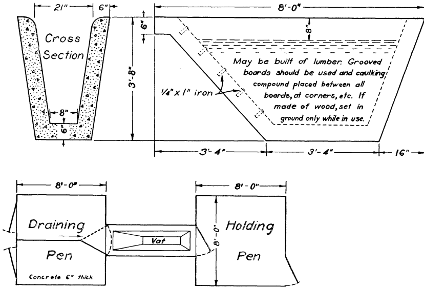
Fig. 21. The above dipping tank may be made of concrete or from lumber in areas where lumber is cheap. This tank may appear narrow, but large sheep can go through easily, and much less dip is needed with these dimensions to accomplish the same results. Drain pens at the outlet of the tank are important to save dip as it drains from the sheep. A holding pen is needed to hold sheep before entering the tank, though a good place to set the tank is at a door through which the sheep are accustomed to going. Portable dipping outfits are available in many areas, offering a convenient dipping service.
