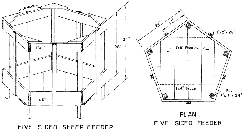
Fig. 22. A convenient combination feeder where space is limited.
