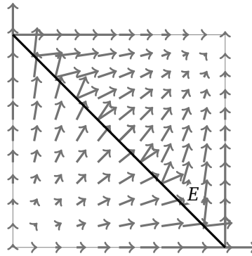
Figure 4.6: Raviart-Thomas basis function \varphi_E in \mathbb{R}^2 belonging to the edge E . The normal jumps over all edges are zero and \varphi_E is therefore H(\text{div}) -conforming.
