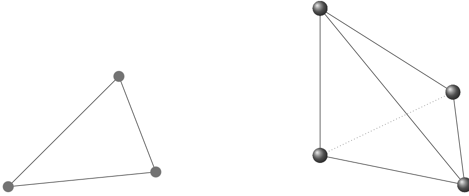
Figure 4.1: The P_1 functions in \mathbb{R}^2 and \mathbb{R}^3 have three resp. four degrees of freedom. The values of the function can be chosen for each node of the simplex - the resulting functions are H^1 -conforming.
