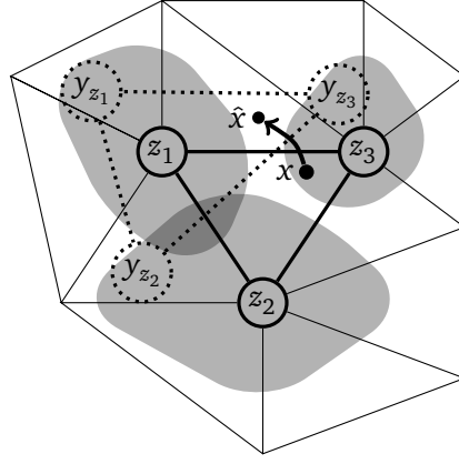
Figure 4.8: Illustration of the mapping \hat{x} defined in equation (4.6). It maps a point x in a triangle T (printed bold) with nodes z_i and fixed points y_{z_i} in regions \omega_{z_i} (grey shaded) around the triangle's nodes to a point \hat{x} in the triangle T' = \text{conv}\{y_z : z \in \mathcal{N}_\ell(T)\} (dotted).
