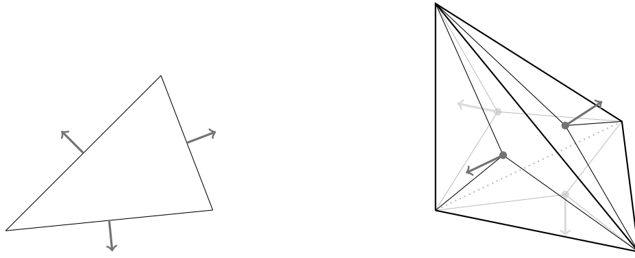
Figure 4.5: The Raviart-Thomas functions in \mathbb{R}^2 and \mathbb{R}^3 of the form v(x_1, x_2) = (a_1 + b x_1, a_2 + b x_2) , have three resp. four degrees of freedom. For each face, the normal component can be chosen - the resulting functions are H(\text{div}) -conforming.
