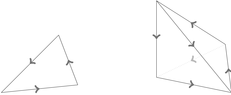
Figure 4.3: The Nédélec functions in \mathbb{R}^2 and \mathbb{R}^3 of the form v(x_1, x_2) = (a_1 - bx_2, a_2 + bx_1) and v(x) = a + b \wedge x , respectively, have three resp. six degrees of freedom. For each edge, the tangential component can be chosen - the resulting functions are H(\text{curl}) -conforming.
