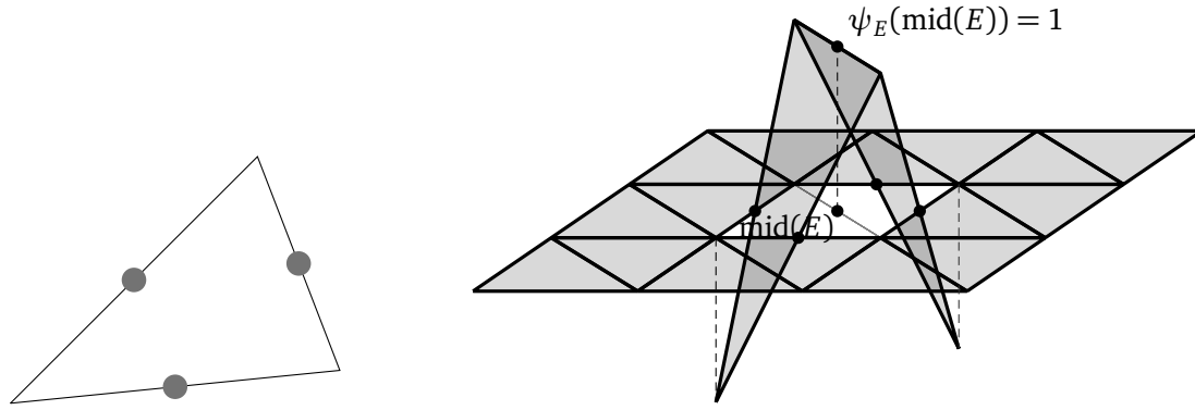
Figure 4.7: The \text{CR}_1 functions in \mathbb{R}^2 have three degrees of freedom. The values of the function can be chosen for the midpoints of the edges/faces (left). The figure on the right shows the \text{CR}_1 basis function \psi_E belonging to edge E (grey). The function is continuous in the midpoints of all edges.
