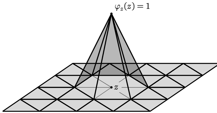
Figure 4.2: P_1 basis function \varphi_z in \mathbb{R}^2 belonging to node z . The function is continuous and therefore H^1 -conforming.
