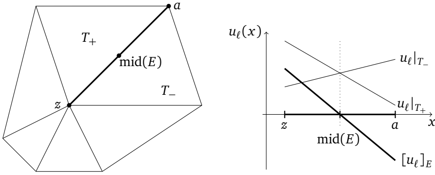
Figure 5.1: Illustration of the geometry and notation in the proof of (5.2d) of Theorem 5.1. To calculate the L^2 -norm of the jump of the CR 1 -function u_\ell along the edge E = T_+ \cap T_- , merely u_\ell|_{T_+} and u_\ell|_{T_-} are evaluated in z .
