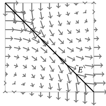
Figure 4.4: Nédélec basis function \varphi_E in \mathbb{R}^2 belonging to the edge E . The tangential jumps over all edges are zero and \varphi_E is therefore H(\text{curl}) -conforming.
