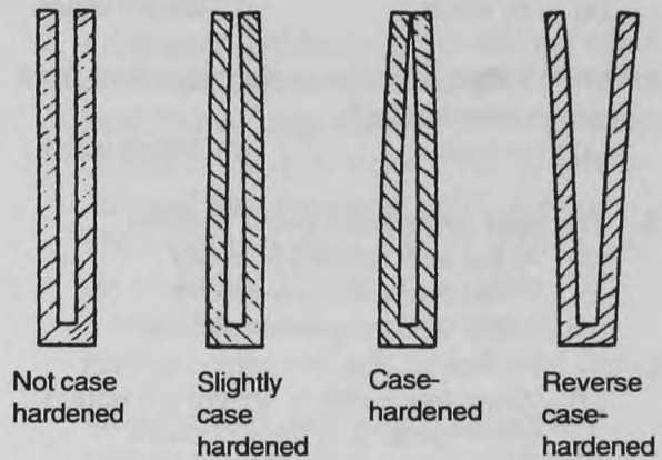
Figure 2.5c Residual drying stress. The severity of residual drying stress (or case hardening) is indicated by cutting a stress section from the cross-section of a board, and noting how far the prongs bend in or out.
