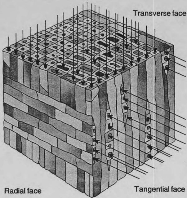
Figure 5.1a In softwoods most preservative flow occurs by means of the vertical fiber tracheids and the horizontal ray tracheids. As these make up virtually all the wood volume, it is possible to fully saturate some softwoods with preservative.
