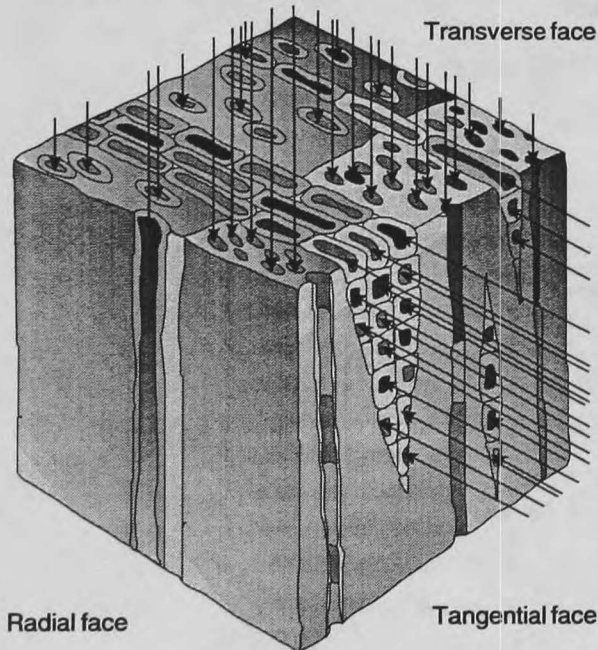
Figure 5.1b In hardwoods only the vessels and the ray tracheids can conduct preservatives. This often leaves extensive regions of fibers unprotected. As these give hardwoods much of their strength, this can be a very serious situation.
