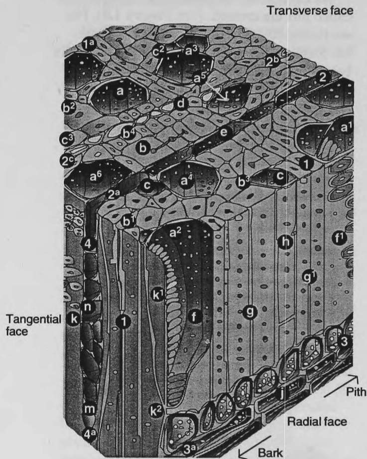
Figure 1.5 Schematic drawing of a typical hardwood-sweetgum. (magnified 330X)
