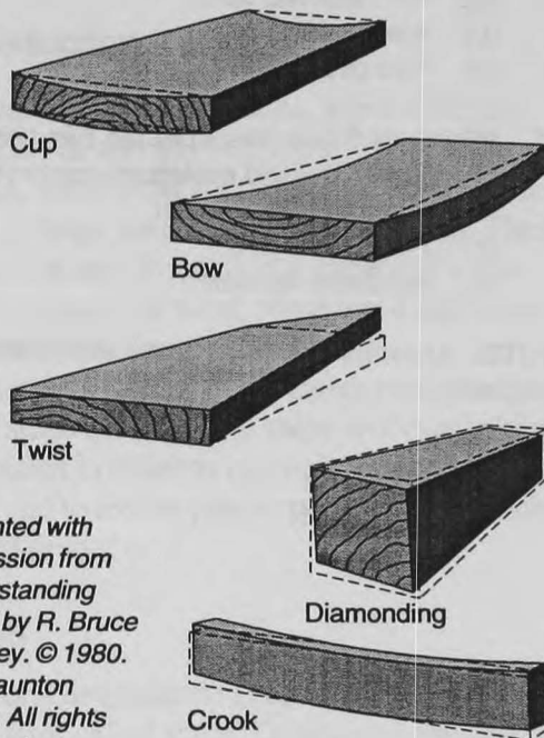
Figure 2.5a Types of warp that develop in boards during drying. Warp is caused by differences between radial tangential and longitudinal shrinkage as the board dries, or by growth stresses. It can be minimized by certain sawing techniques and proper stacking.
