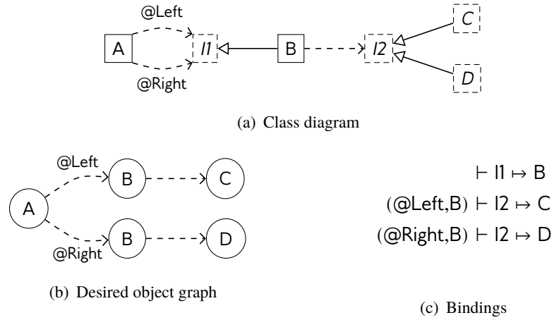
Figure 4.6: A dependency graph requiring context-sensitive policy. X \vdash I \mapsto C denotes that I is bound to C only when satisfying dependencies of X .
