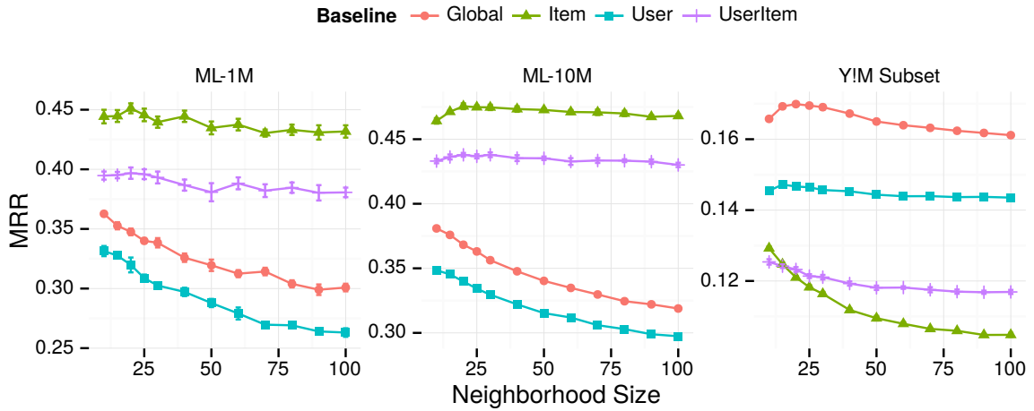
Figure 5.12: Item-item top- N performance by baseline normalizer
