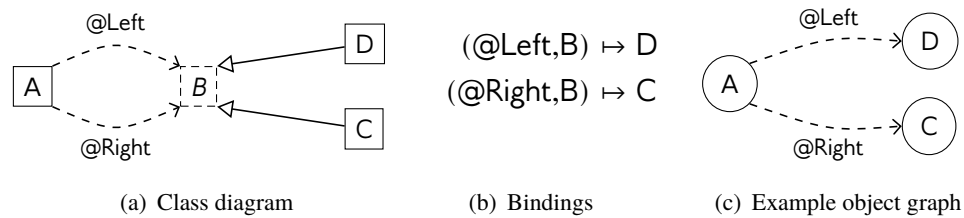
Figure 4.3: Component with qualified dependencies (indicated by edge labels).
