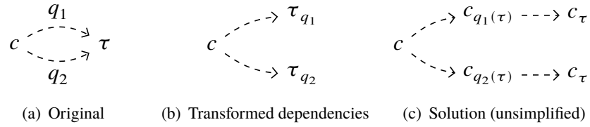
Figure 4.9: Reduction of qualified graph.
