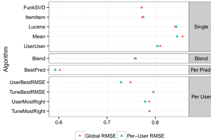
Figure 6.1: Algorithm prediction error.
