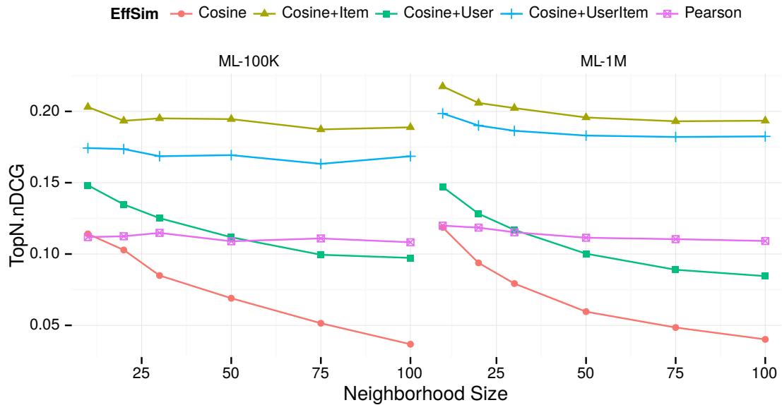
Figure 5.11: Top- N evaluation of CF configurations.
