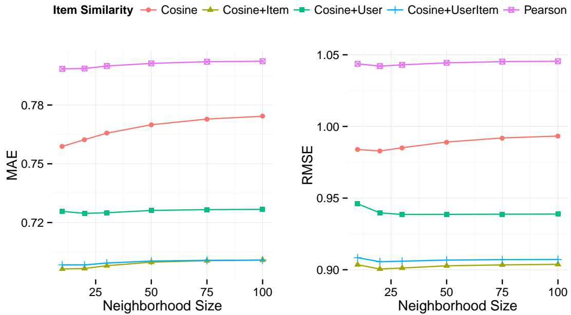
Figure 5.5: Prediction accuracy for item-item CF on ML-1M.
