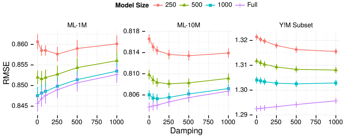
Figure 5.7: Item-item accuracy by similarity damping.
