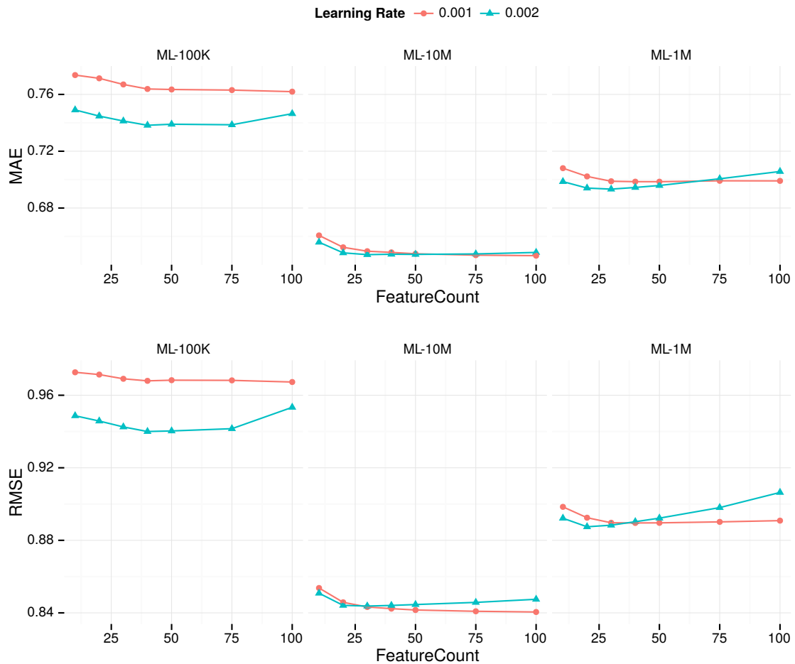
Figure 5.9: Prediction accuracy for regularized SVD.
