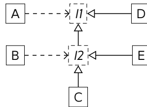
Figure 4.7: Class graph with subtypes
