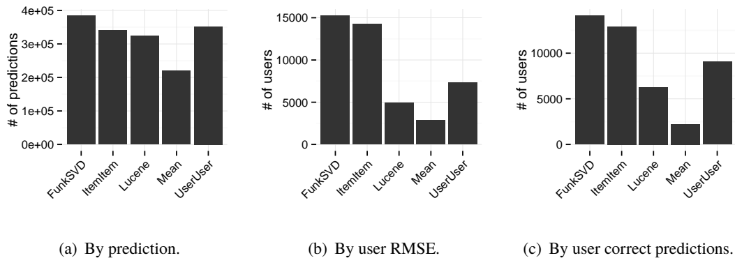
Figure 6.3: Distribution of best algorithms, by prediction and user.
