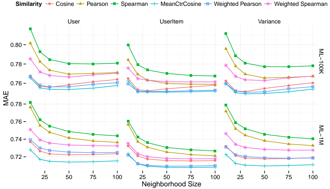
Figure 5.3: Prediction accuracy (MAE) for user-user CF, across two data sets with different choices of similarity function and score normalization.
