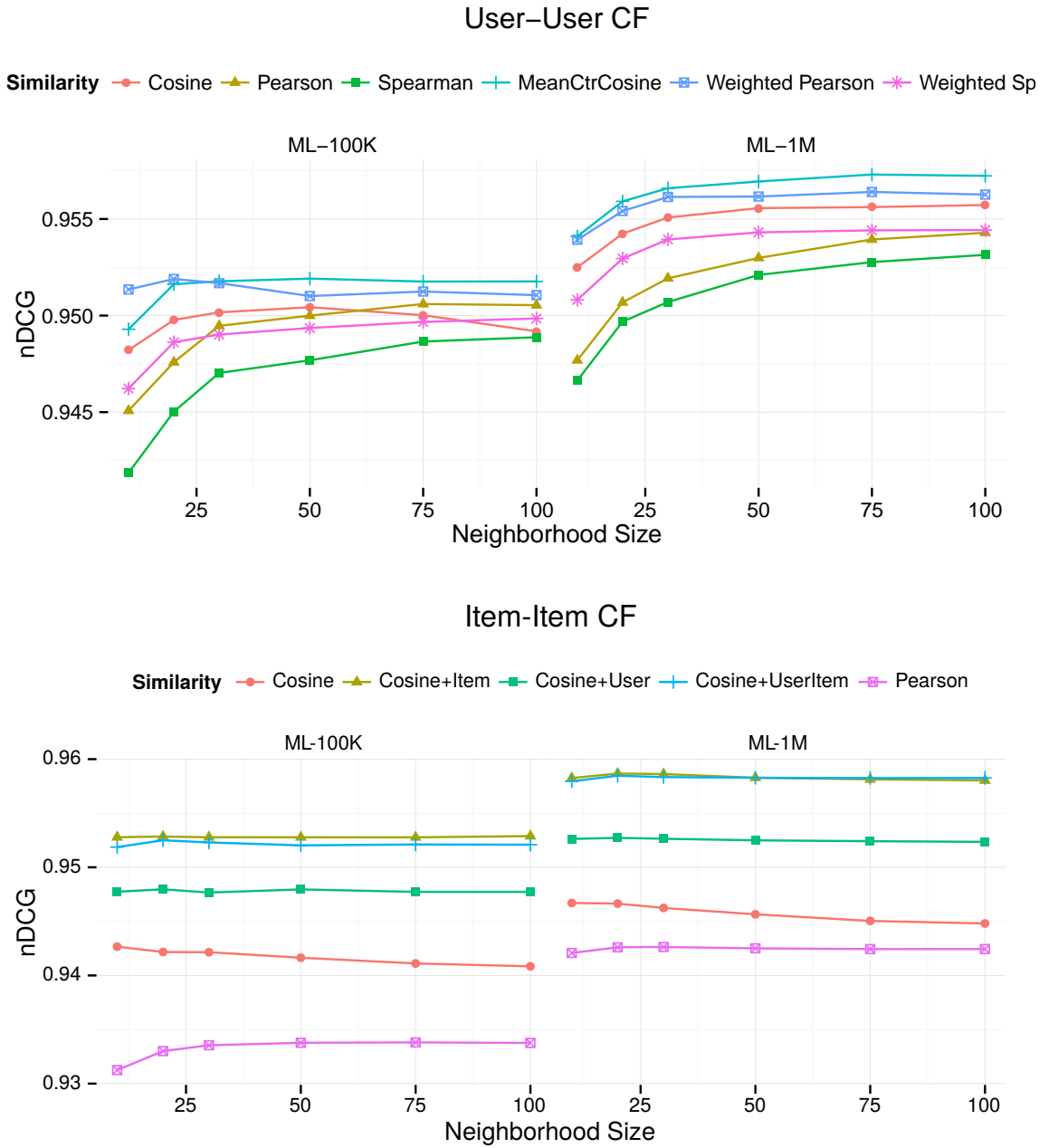
Figure 5.10: Rank-based evaluation of CF configurations.
