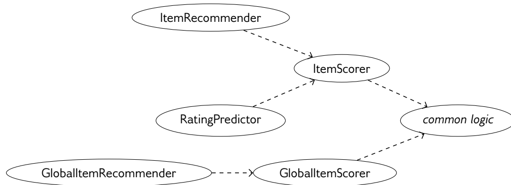
Figure 3.2: Diagram of LensKit API components
