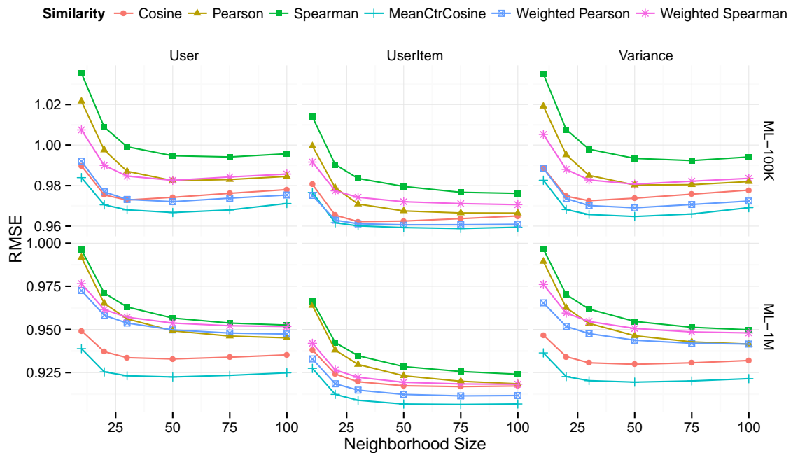
Figure 5.4: Prediction accuracy (RMSE) for user-user CF, across two data sets with different choices of similarity function and score normalization.
