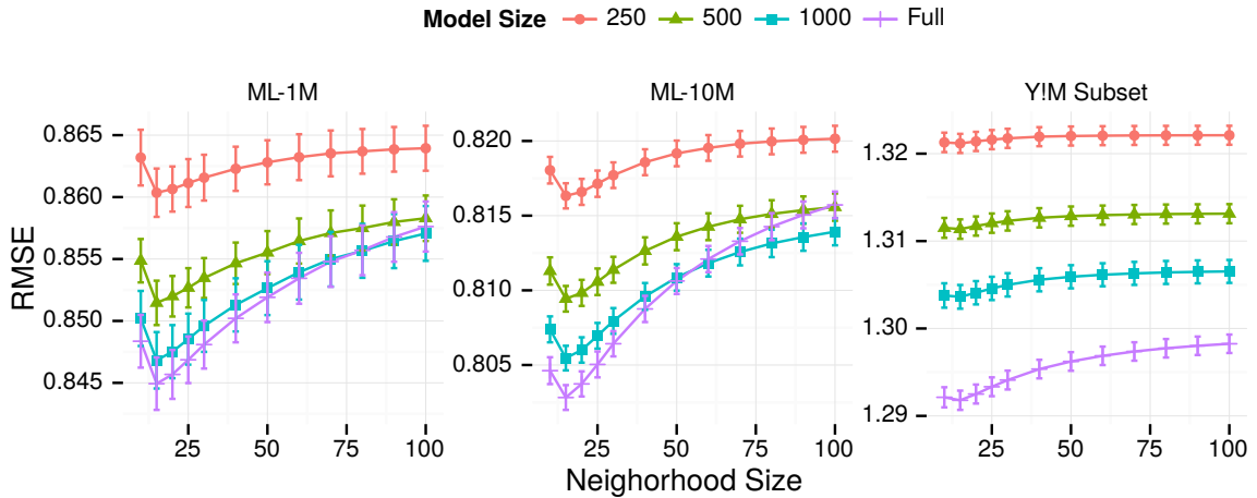
Figure 5.6: Item-item accuracy by neighborhood size.
