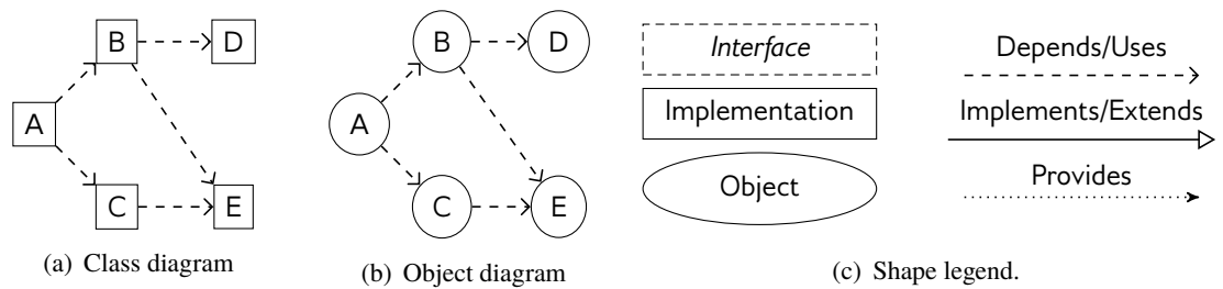
Figure 4.1: Class dependencies, object graph, and legend.
