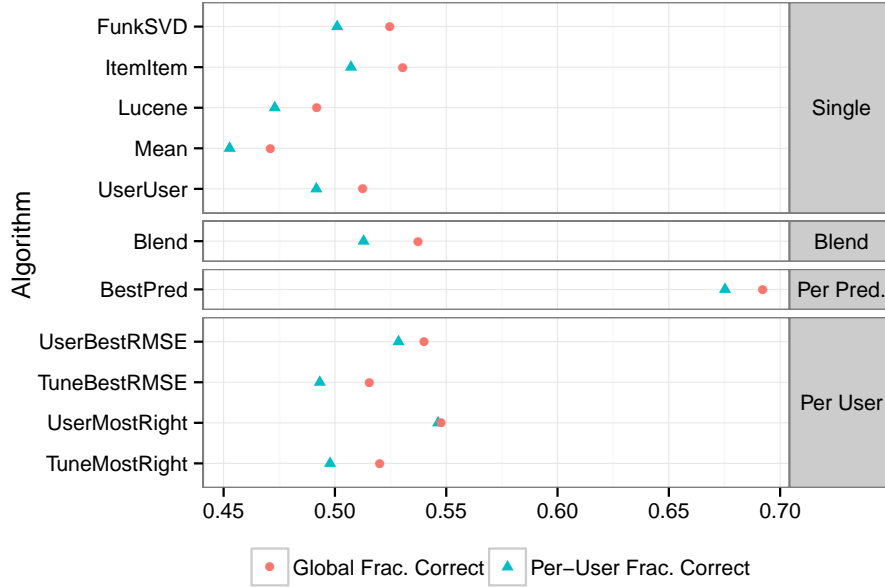
Figure 6.2: Correct predictions by algorithms.
