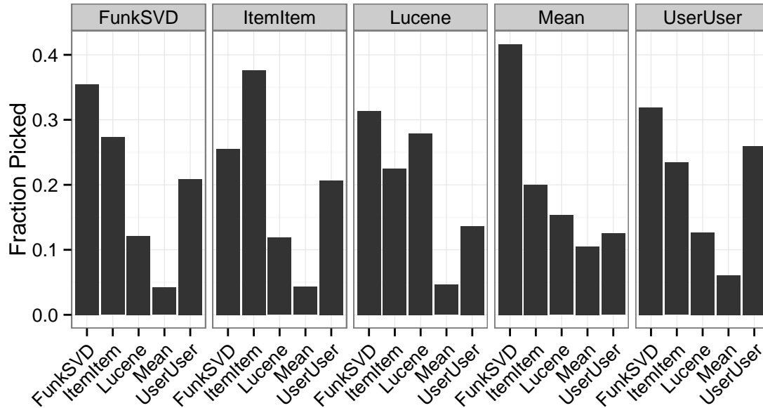
Figure 6.4: Comparative distributions of picked algorithms by user. Each panel contains the users for which the RMSE oracle hybrid picked the given algorithm, and shows the distribution of algorithms picked by the Most Right oracle hybrid.
