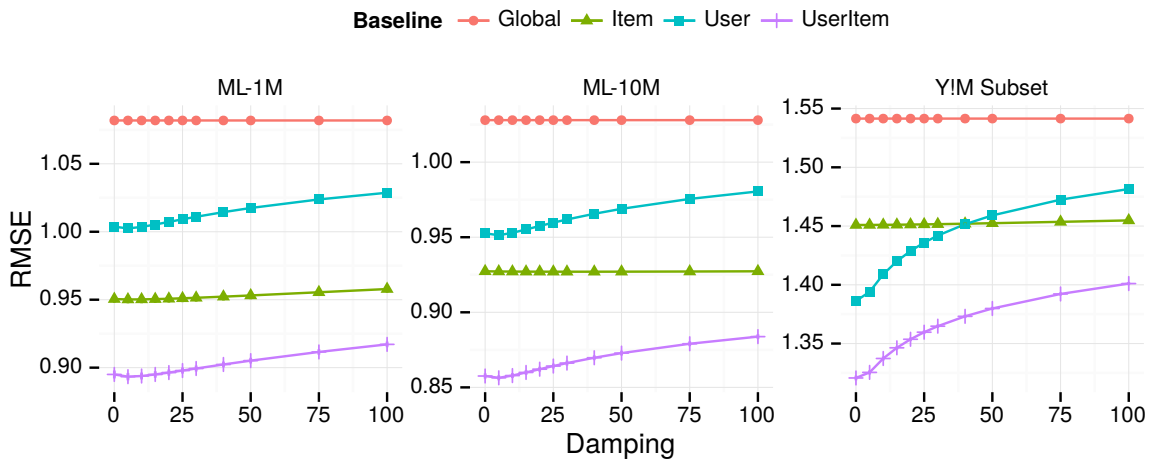
Figure 5.2: Impact of baseline damping
