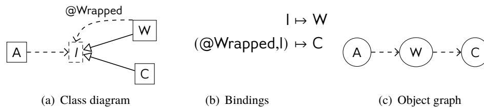
Figure 4.4: A wrapper component. W implements I by wrapping another component of type I , in this case C .
