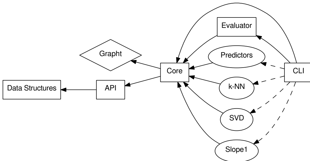
Figure 3.1: LensKit modules and their relationships
