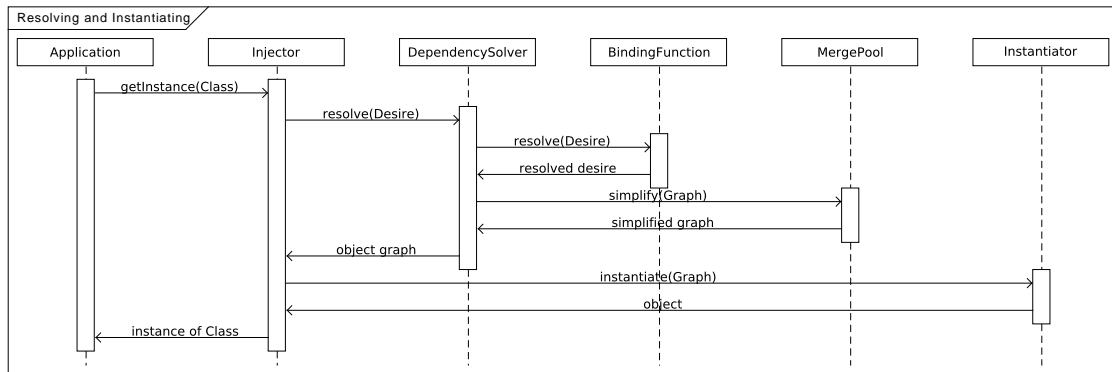
Figure 4.8: Simplified instantiation sequence diagram.
