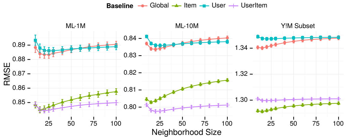
Figure 5.8: Normalizer impact on item-item performance.
