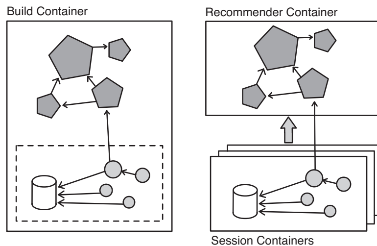
Figure 3.4: Object containers in a LensKit web application 13 .
