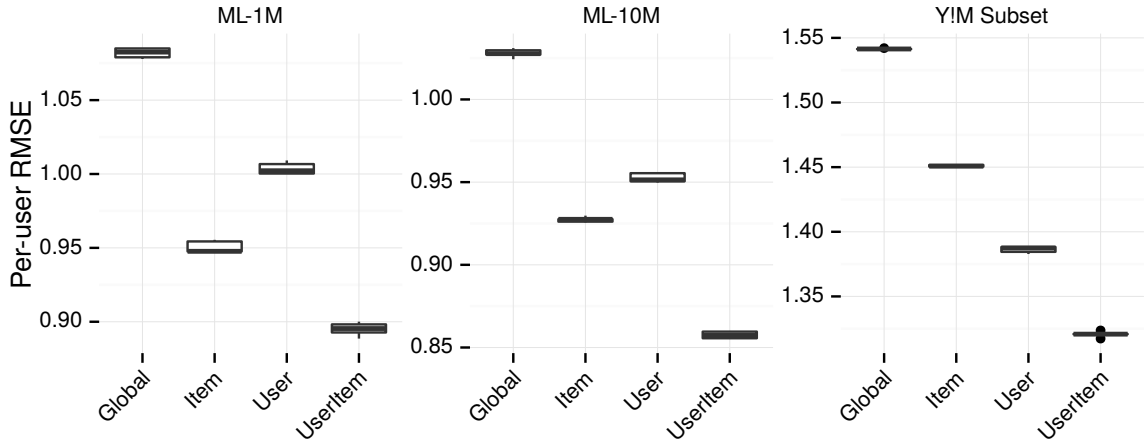
Figure 5.1: Baseline scorer accuracy
