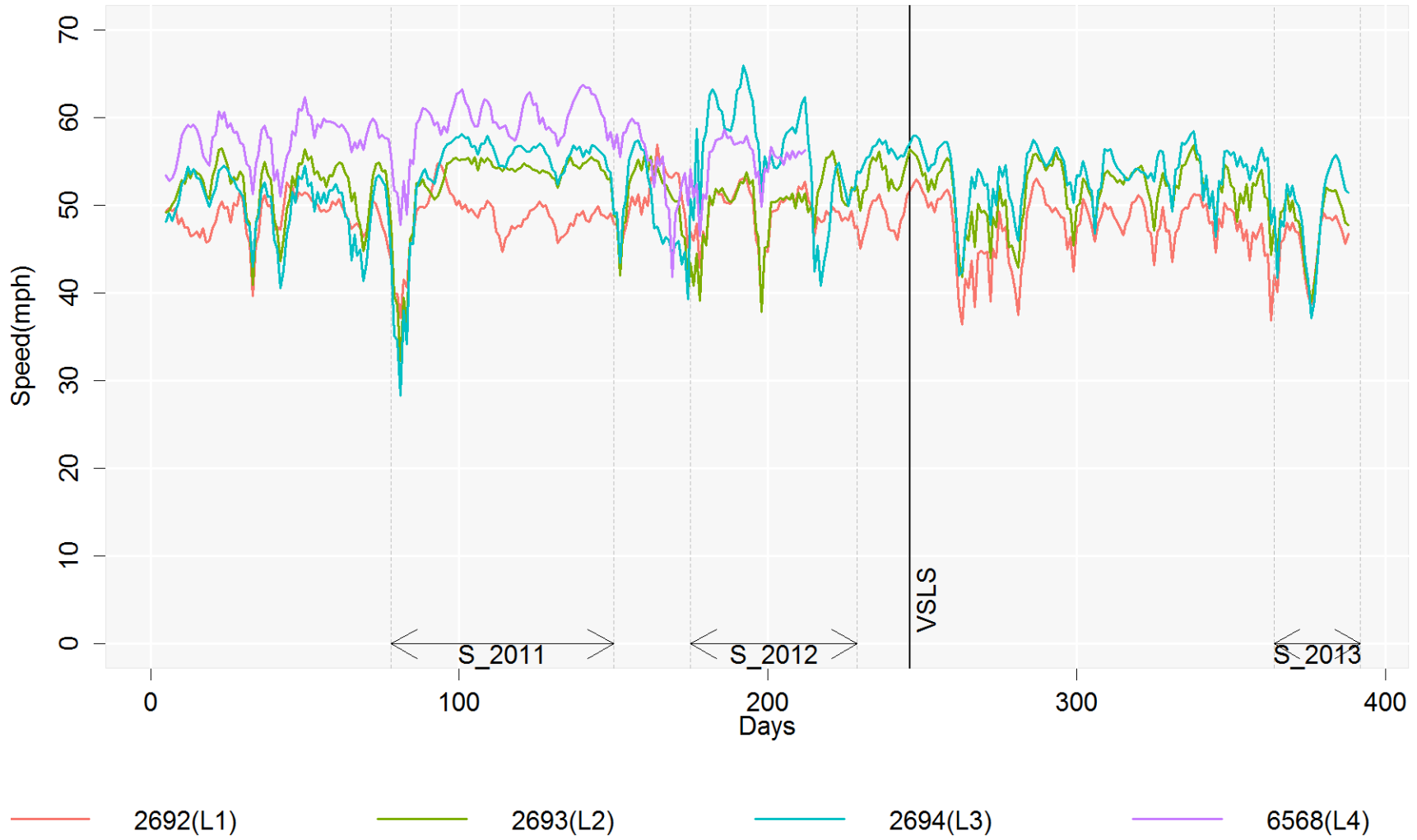
Figure 39. Five minute average speed (5 to 10 minutes after breakdown) for station 559
