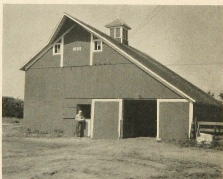
Fig. 8. A combined livestock barn, hay barn, and granary. Such structures prevent the natural, seasonal cooling of grain stored in them, and permit activity of stored grain insects throughout most of the year.
