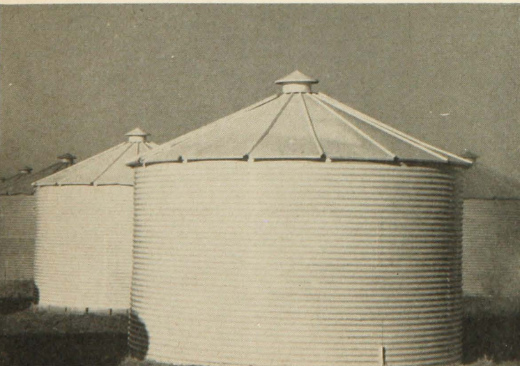
Fig. 9. Metal bins with walls and roofs painted white maintain grain temperatures several degrees lower than that of grain stored in unpainted metal bins.
