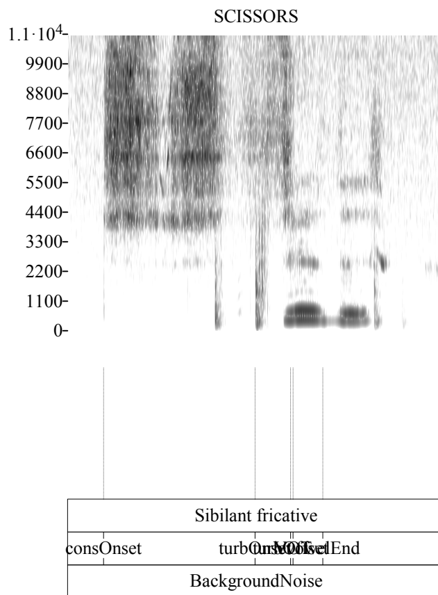
Figure I. Example of an Emerging Fricative where consOnset is used
