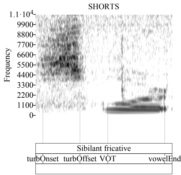
Figure G. Example showing use of turbOffset Note the period of silence between turbOffset and VOT
