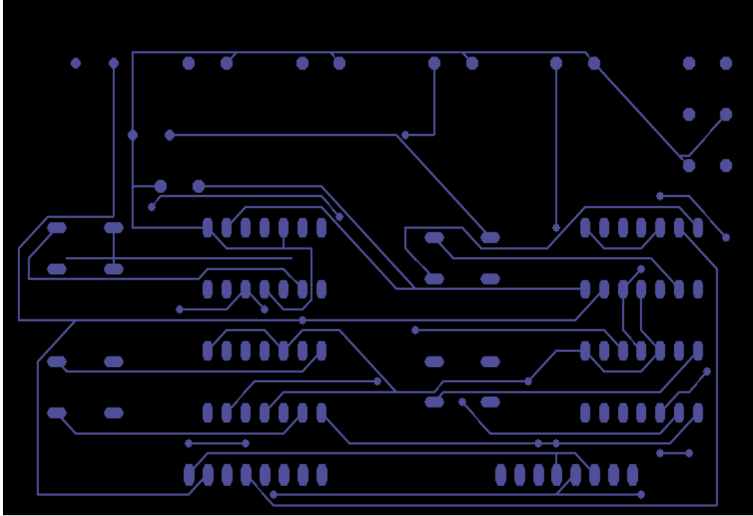
Figure 22 .sol file
