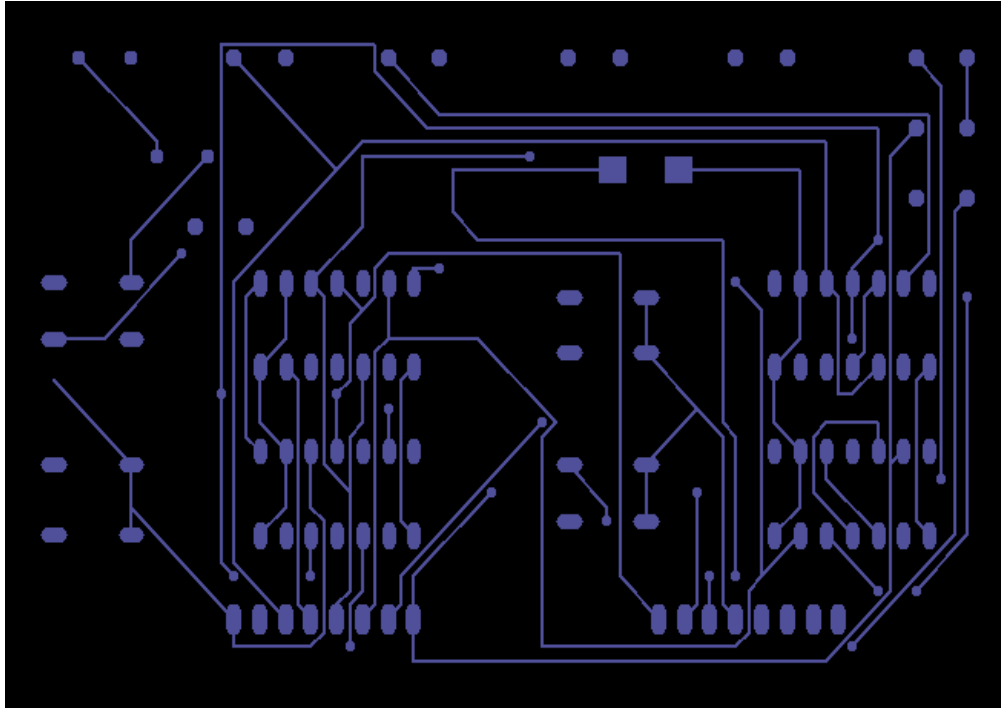
Figure 21 .cmp file
