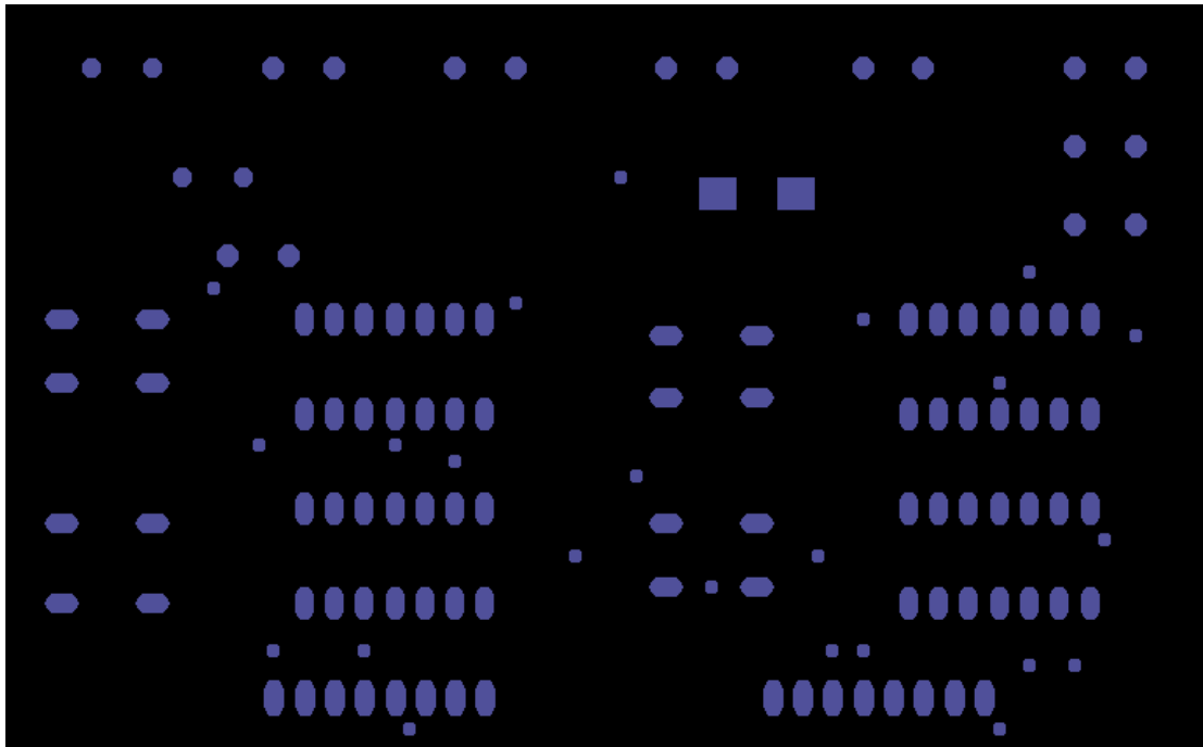
Figure 23 .stc file
